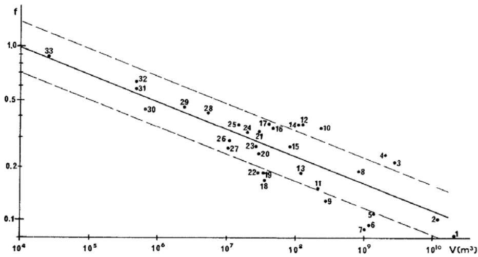
Fig. 2. Correlation between landslide volume V (in m^3 ) and the coefficient of friction f .
