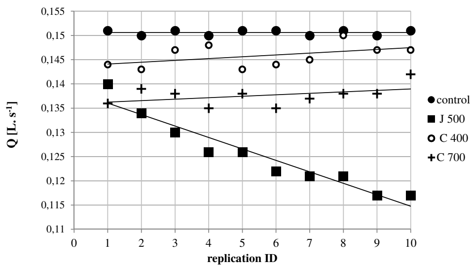
Figure 4 Peak discharge at outlet section, Q (L.s -1 ); linear trend-lines included; laboratory conditions. For the data see supplementary Table S2.
