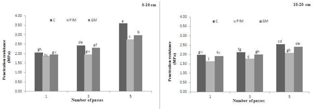
Figure 1. The effects number of passes on penetration resistance in different depths (passing×depth×treatment). Different letters written above columns indicate the difference in the treatment means at P < 0.05 .
