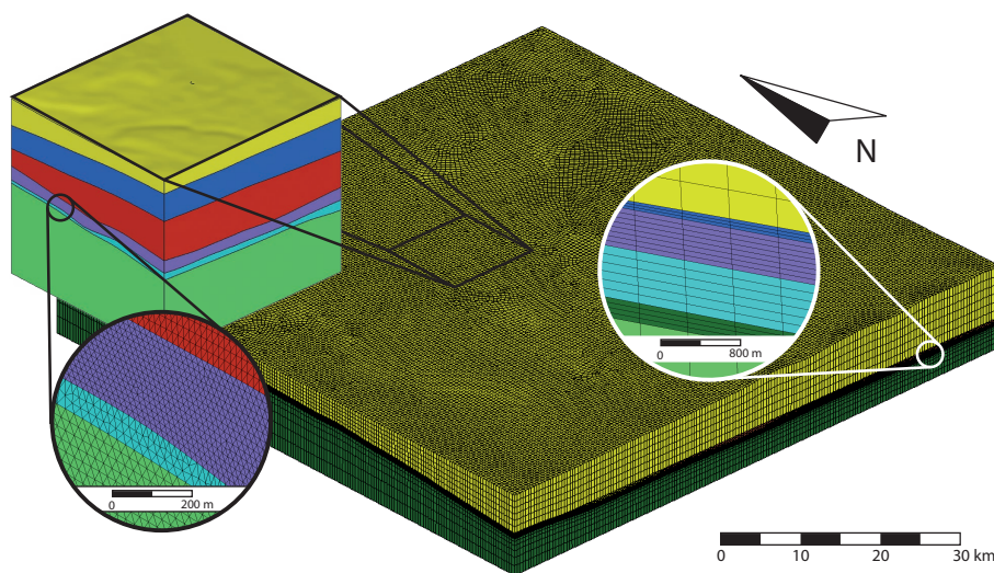
Figure 3. The root and branch model discretised with 10^6 hexahedral and 21 \times 10^6 tetrahedral elements respectively. Please note that to improve visibility the discretisation of the branch model is only displayed within the magnified inset. Both magnified regions show the Malm \alpha - \gamma (turquoise) and Malm \delta - \zeta and Purbeck (purple) units which are the predominant target units for geothermal exploration in the Bavarian Molasse Basin.
