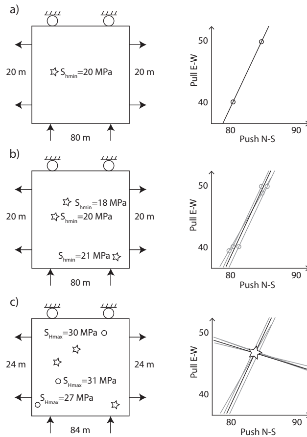
Figure 4. Left: Exemplified schematic models with the data records used for calibration (star: S_{hmin} magnitude, circle: S_{Hmax} magnitude). Right: Linear slopes that display the magnitudes of possible combinations of displacement boundary conditions applied normal to the the E-W (y-axis) and N-S (x-axis) sidewalls of the model. For each data record an individual slope defines the possible combinations of boundary conditions to fit the model to this calibration data record. a) A single S_{hmin} magnitude can be calibrated by an unlimited amount of combinations of boundary conditions which are on a linear slope. b) Several S_{hmin} magnitudes usually cannot be calibrated to an exact fit. However, a linear regression of all the linear slopes derived for the calibration of each individual data record provides a “best-fit” slope. This slope defines combinations of “best-fit” boundary conditions that fit the data records used for calibration equally well. c) Several S_{hmin} and S_{Hmax} magnitude data records used for calibration result for each S_{hmin} and S_{Hmax} in a linear slope of combinations of “best-fit” boundary conditions. At the intersection of these two slopes the “best-fit” boundary conditions (indicated by a star) are found for the calibration of both S_{Hmax} and S_{hmin} together.
