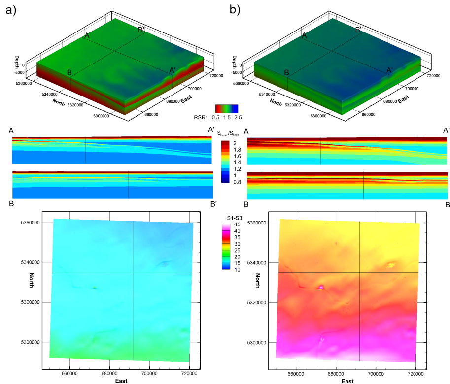
Figure 6. Results of the “best-fit” root model (b) and an alternative scenario that fits the S_{\text{Hmin}} values equally well, but is calibrated against a lower S_{\text{Hmax}} value (a). The overall difference that results from the different S_{\text{Hmax}} values used for the calibration is expressed in the continuous scale of the stress regime ratio (RSR) which is between 0.5 (normal faulting regime), 1.5 (strike slip), and 2.5 (thrust faulting regime) (Simpson, 1997) in the model volume. The horizontal stress anisotropy expressed in the ratio of S_{\text{Hmax}}/S_{\text{Hmin}} is shown on two cross sections which intersect below Munich. The differential stress (difference between the maximum and minimum principal stress, lowermost panel) is mapped on a surface which is vertically centered in the Malm \alpha - \gamma units.
