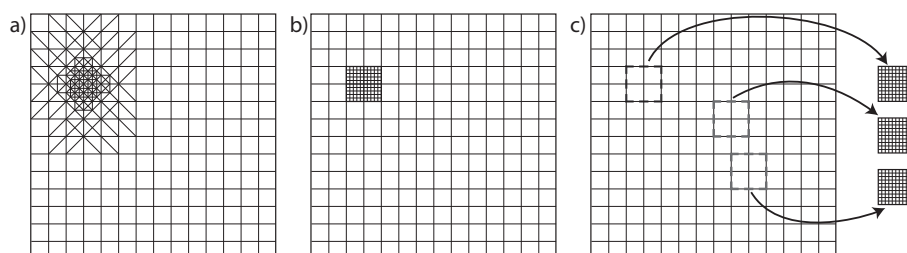
Figure 2. Different types of modelling approaches: a) A refined mesh in the area of interest is expensive and inefficient due to the large amount of elements required for the discretisation of the gradient in resolution. Furthermore, it requires a complete re-mesh and re-evaluation in case of any changes in the geometry or input data. b) A local model nested within a regional model matches the variables at the boundary. A complete re-mesh and re-evaluation is required in case of geometry or input data changes. c) A multi-stage approach has the easiest mesh generation since the differently sized models are generated independently. Furthermore, several reservoir models can be based on the same regional model.
