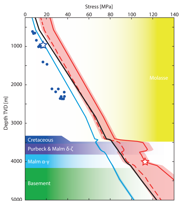
Figure 8. Stratigraphy and model result of the root model along the borehole of the geothermal project in Sauerlach. Lines show the results of the “best-fit” root model: blue for the S_{hmin} magnitude, black for the vertical stress and red for the S_{Hmax} magnitude. The blue dots are formation integrity tests (FITs) which are a lower boundary for the magnitude of S_{hmin} and not used for calibration, the blue star represents the suspected LOT, the red star shows the S_{Hmax} magnitude of 112MPa used for calibration (Seithel et al., 2015). Shaded areas in the same colour around the lines show the range of model scenarios that fit equally well to the model-independent constraints. The dotted red line shows the S_{Hmax} magnitude for the model scenario in Fig. 6a.
