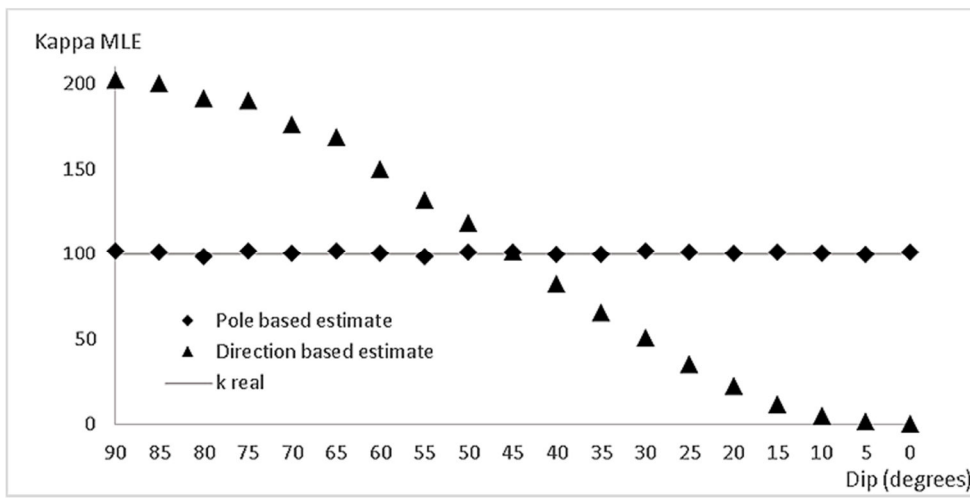
Figure 665: Distortion of the Maximum Likelihood Estimation (MLE) of concentration/spherical variance of a hundred spherical unit vector samples of a size of a thousand individuals drawn from a von Mises-Fisher distribution with \kappa = 100 . Pole based estimate is always consistent with the data while dip based ones either over or underestimate it.
