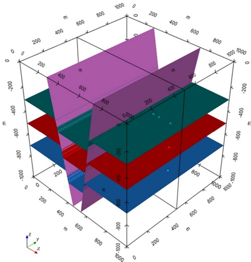
Figure 887: Structural data for the graben model and modelled surfaces for units and faults. Spheres represent interfaces and cones represent pole vectors.
