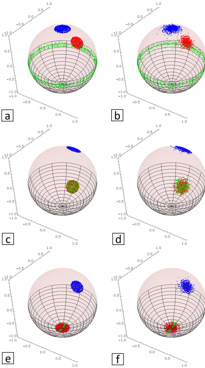
Figure 736: Effect of sampling over dip vectors or pole vectors on bounded uniform spherical distribution at range = 10^\circ (a, c, e) and von Mises-Fisher distribution at \kappa = 100.0 (b, d, f) for uncertain horizontal planes (a, b), 45^\circ dip planes (c, d) and vertical planes (e, f). Correct (pole perturbed) dip vectors are green, incorrect (dip perturbed) dip vectors are red and blue vectors are the poles. See section 4.1 for details.
