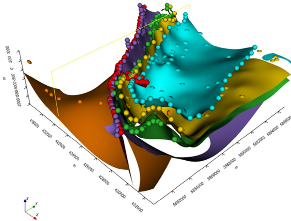
Figure 10109: Structural data for the Mansfield model and modelled surfaces for units and faults. Spheres are interfaces and cones are orientations.
