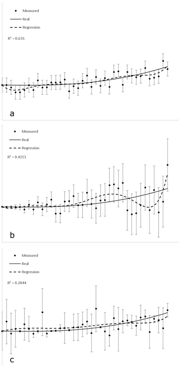
Figure 443: Synthetic examples of different levels of heteroscedasticity of measurements of the same variable. (a) homoscedastic case, (b) structured heteroscedastic case and (c) unstructured heteroscedastic case. Note how the least square polynomial residuals score ( R^2 ) is heavily impacted by heteroscedasticity.
