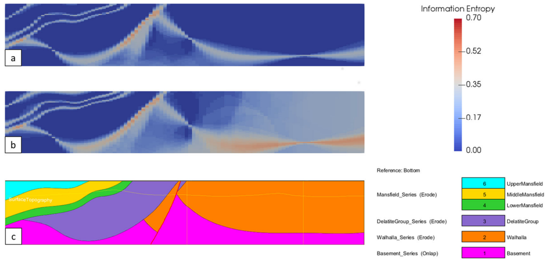
Figure 111110: Effect of pole (a) versus dip (b) perturbation on a cross-section of the Mansfield model (c), orientations are perturbed over a von Mises-Fisher distribution with \kappa = 100 .
