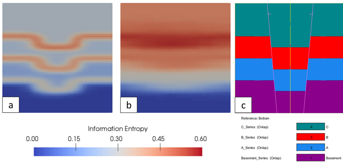
Figure 998: Effect of pole (a) versus dip (b) perturbation for a graben model (c), orientations are perturbed over a vMF distribution with \kappa = 100 .
