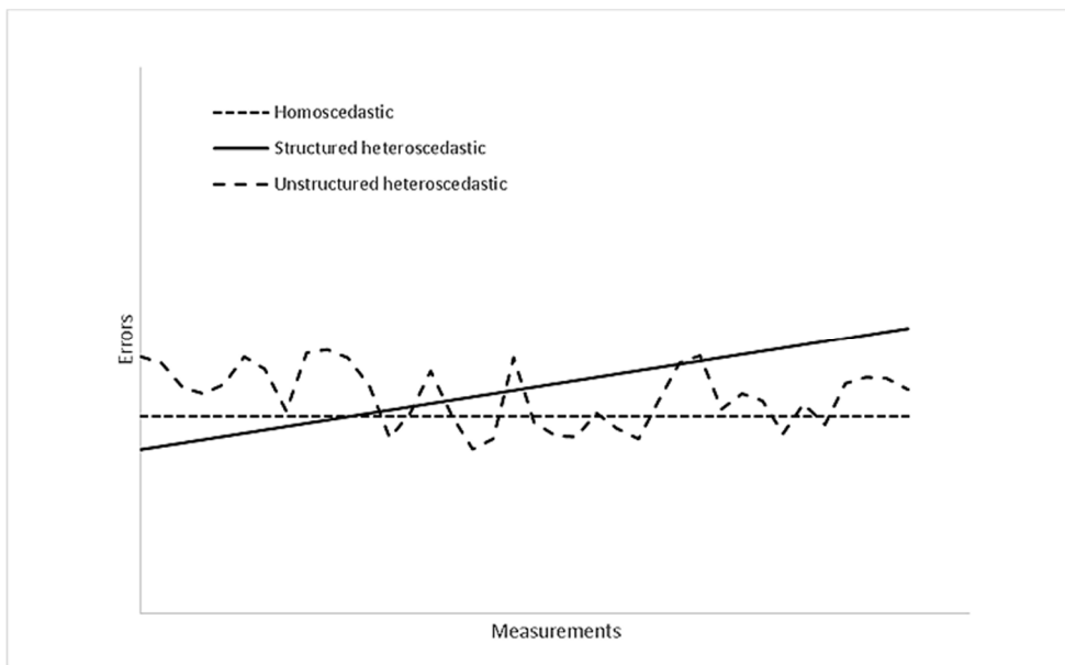
Figure 554: Distribution of errors for the cases described in Figure 3. Homoscedastic case shows constant uncertainty and no relationship of uncertainty to the data. The structured heteroscedastic case has a linear relationship of uncertainty to the data. The unstructured heteroscedastic case demonstrates no obvious relationship of uncertainty to the data and is not constant.
