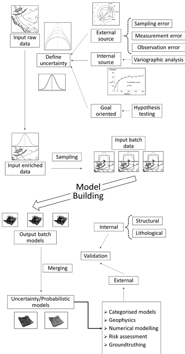
Figure 1: Monte Carlo Uncertainty Propagation procedure workflow.
