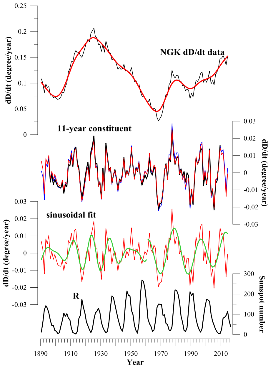
5 Figure 3: Constituents of the first time derivative of the declination at Niemegek observatory. First panel: first differences of annual means (thin black curve) and the trend from a HP filtering (thick red curve). Second panel: cyclic constituent from a HP filtering (red), the 11-year signal from filtered first differences by an 11-year cutoff high-pass Butterworth filtering (blue), and the 11-year signal obtained as a residual after the removal of an 11-year running average from the dD/dt time-series (black). Third panel: the cyclic component (red) compared to a two-waves sinusoidal fit (green) for the time intervals 1890-1960 and 1960-2011. Fourth panel: the sunspot number time series (R).
