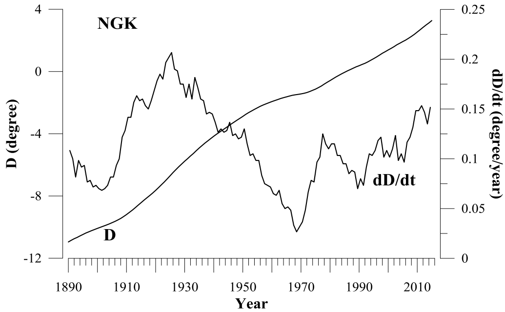
10 Figure 1: Declination and its first time derivative time-series. Example for a high-standards geomagnetic observatory (Niemegek, NGK).
