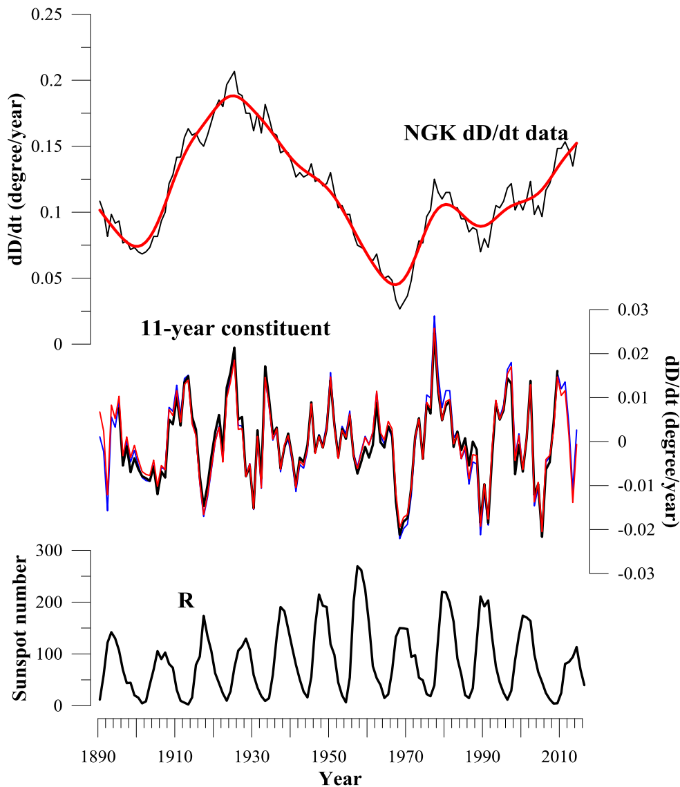
5 Figure 3: Constituents of the first time derivative of the declination at Niemegek observatory. First panel: first differences of annual means (thin black curve) and the trend from a HP filtering (thick red curve). Second panel: cyclic constituent from a HP filtering (red), the 11-year signal from filtered first differences by an 11-year cutoff high-pass Butterworth filtering (blue), and the 11-year signal obtained as a residual after the removal of an 11-year running average from the dD/dt time-series (black). Third panel: the sunspot number time series (R).
