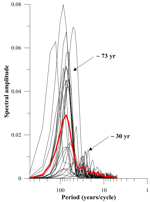
Figure 2: FFT power spectrum: observatory declination time-series (a); time derivative of declination time-series (b). The average power spectrum (red).
