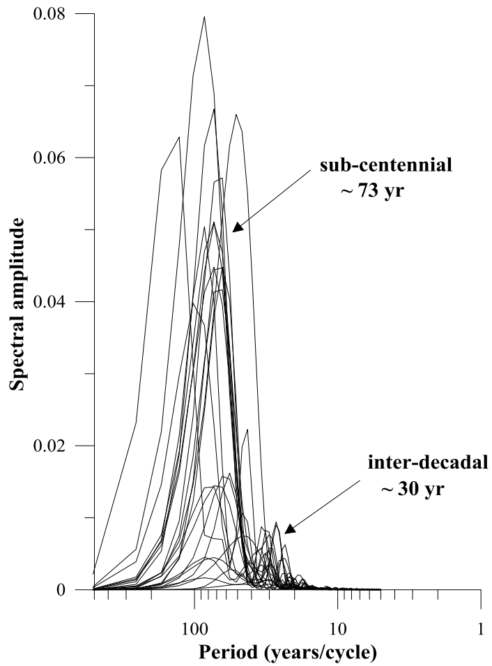
5 Figure S2: FFT power spectrum for the HP trend (i.e. the ~11-year variation removed) of declination first time derivative.
