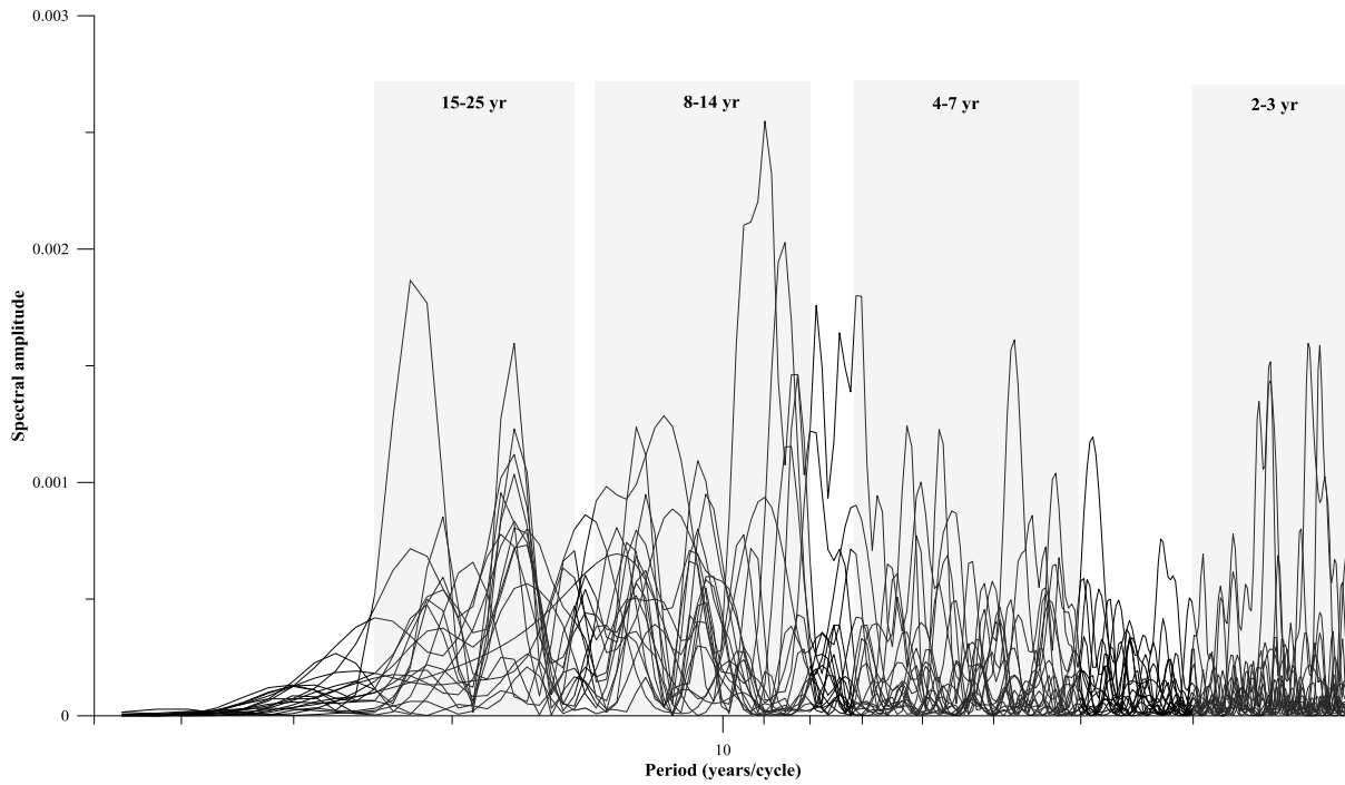
5 Figure S3: FFT power spectrum for the cyclic constituent from HP filtering of the first time derivative of declination. Gray background: domains of 8-14 years, 15-25 years, 4-7 years and 2-3 years.
