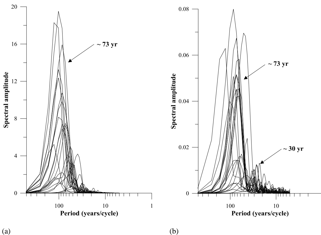
Figure 2: FFT power spectrum: observatory declination time-series (a); time derivative of declination time-series (b).
