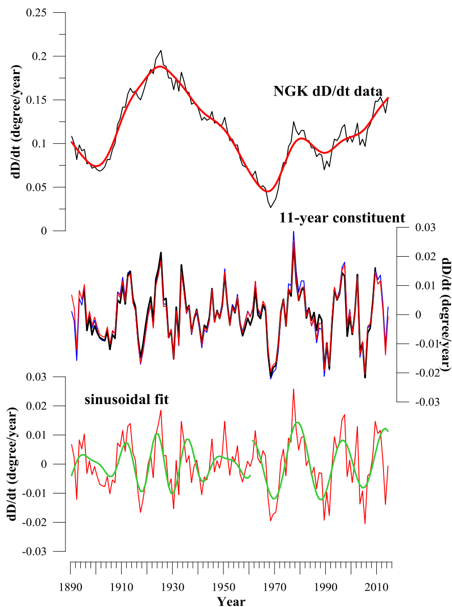
Figure 3: Constituents of the first time derivative of the declination at Niemegek observatory. Top: first differences of annual means (thin black curve) and the trend from a HP filtering (thick red curve). Middle: cyclic constituent from a HP filtering (red), the 11-year signal from filtered first differences by an 11-year cutoff high-pass Butterworth filtering (blue), and the 11-year signal obtained as a residual after the removal of an 11-year running average from the dD/dt time-series (black). Bottom: the cyclic component (red) compared to a two-waves sinusoidal fit (green) for the time intervals 1890-1960 and 1960-2011.
