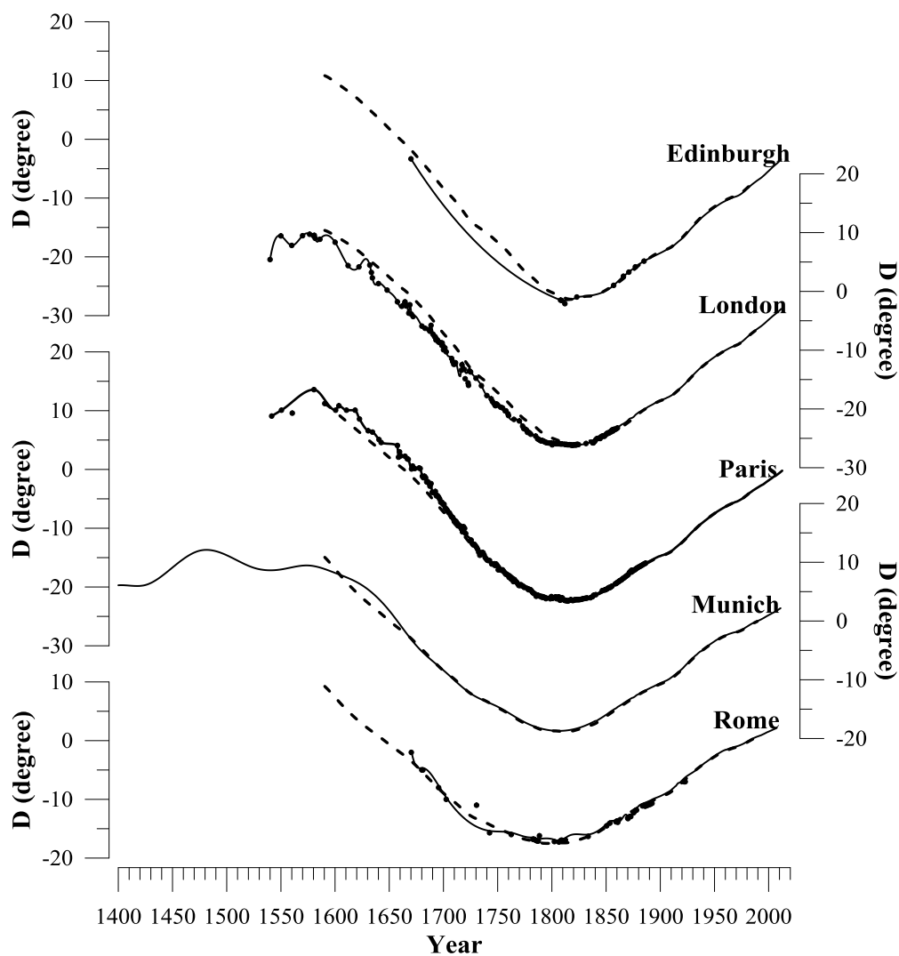
5 Figure 8: The declination evolution since 1400 AD at five locations in Europe. Annual values as obtained by a cubic B-spline interpolation on historical observations and observatory data (full black curve); and as obtained from the gufm1 time-series (dashed curve).
