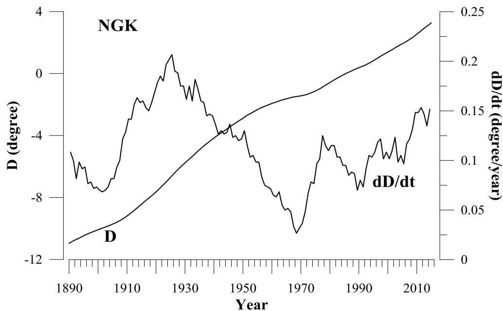
Figure 1: Declination and its first time derivative time-series. Example for a high-standards geomagnetic observatory (Niemegk, NGK).
