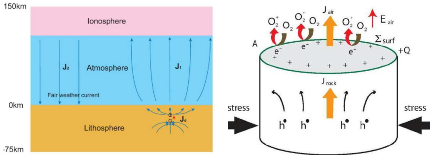
4 5 Fig. 8. Freund model (adapted from Kuo et al., 2014)
