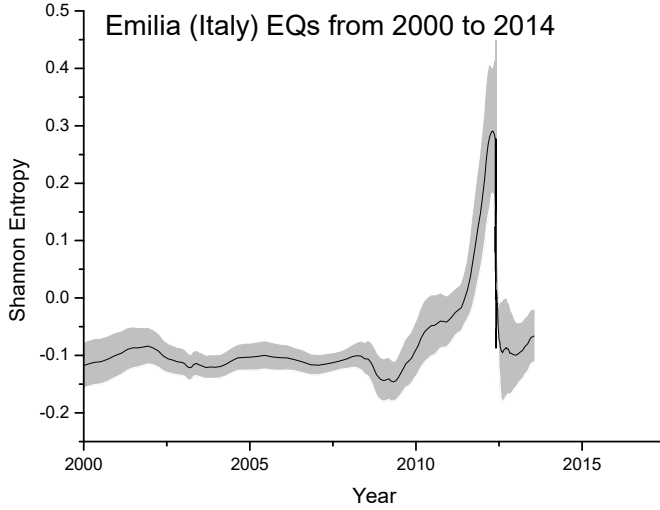
3 Fig. 5. Shannon entropy for Emilia seismic sequence from 2000 to 2014. The significant increase from around 2010, 4 with the maximum at around the main-shock occurrence, is expected to be real. The gray area defines the statistically 5 estimated (1 standard deviation) error in computing the entropy.
