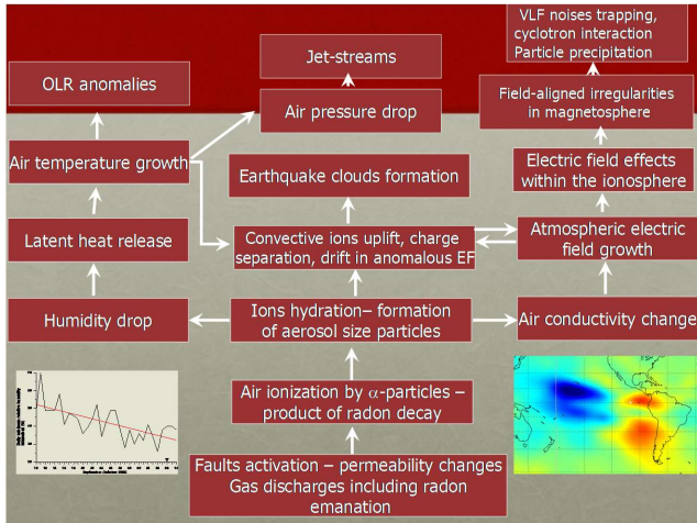
Fig.7. Pulinetz-Ouzonov LAIC model (adapted from Pulinetz & Ouzonov, 2011; Pulinetz et al., 2015)
