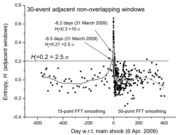
12 13 Fig. 3. Shannon entropy for L'Aquila seismic sequence from around 1.5 year before the main-shock to around 1 year 14 after, calculated for a circular area of 80 km around the main-shock epicenter. Each point is the entropy analysis based 15 on non-overlapping windows, each composed by 30 foreshocks. The gray curve defines a reasonable smoothing of the 16 entropy values: 15-point FFT before the main-shock and 50-point FFT smoothing after the main-shock. The different 17 kind of smoothing is related to the different rate of seismicity before and after the main-shock. It is interesting how the 18 smoothed curve reproduces the expected behavior of a critical system around its critical point. (Adapted from Wu et al. 19 2016). 20
