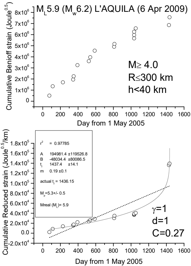
1 2 Figure 6a — Analyses of L'Aquila seismic sequence M \geq 4 EQs (main-shock not shown and not used in the analysis): 3 top) ordinary AMR method; bottom) R-AMR method. Dashed line represents the best linear fit, while solid gray curve 4 is the best power law fit. Results of the fit are shown in the frame inside the graph at the bottom; r^2 is the coefficient of 5 determination, providing a measure of the quality of the fit (the closer to 1, the better the fit). 6 7 We find a clear seismic acceleration for both seismic sequences, quantified by a low value of C 8 (0.27 for L'Aquila sequence and 0.46 for Emilia sequence) and a great determination coefficient 9 ( r^2 > 0.95 in both cases). In addition, the predicted magnitudes are comparable with (although lower 10 than) the real ones. In both cases, the beginning of clear acceleration starts around 1.5 year before 11 the main-shock.
