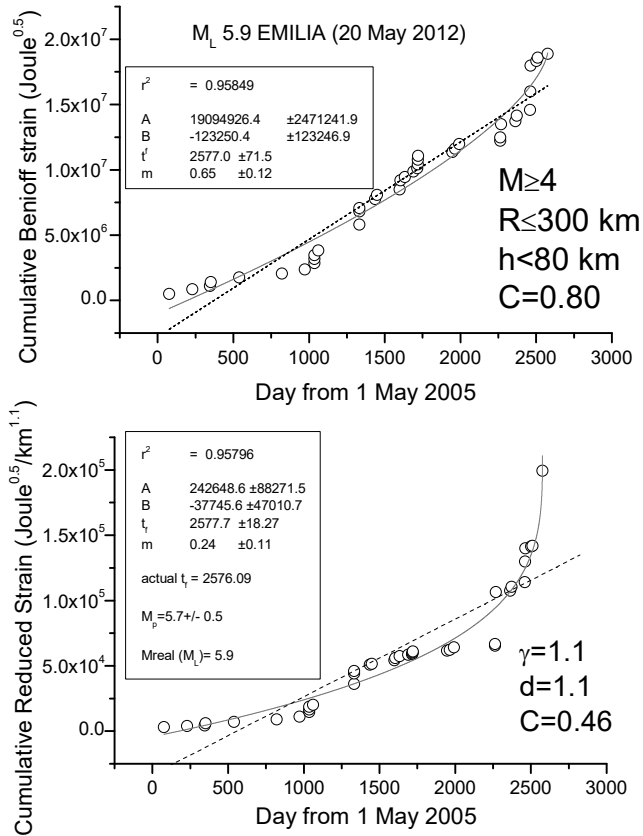
1 2 Figure 6b — Analyses of Emilia seismic sequence M \geq 4 EQs (main-shock not shown and not used in the analysis): top 3 ordinary AMR method; bottom) R-AMR method. Here the ordinary ASR also showed a little acceleration ( C - 4 factor=0.80) but the R-AMR version is much better ( C -factor=0.46). Dashed line represents the best linear fit, while 5 solid gray curve is the best power law fit. Results of the fit are shown in the frames inside the graphs; r^2 is 6 the coefficient of determination, providing a measure of the quality of the fit (the closer to 1, the better the fit).
