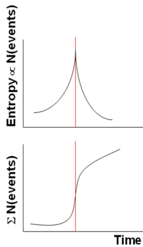
6 7 Fig. 2. Idealized Shannon entropy (above diagram) and cumulative number of events (bottom diagram) for a dissipative 8 system around its critical point, indicated by the vertical red line.
