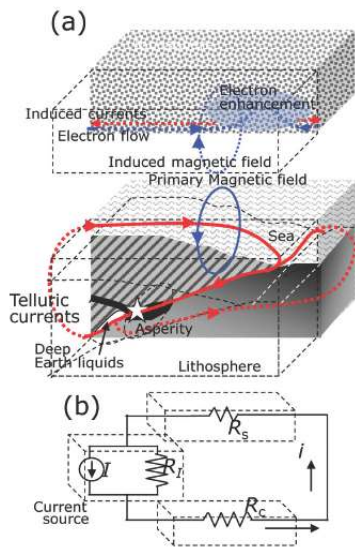
12 13 Fig. 9. Enomoto model (adapted from Enomoto, 2012)
