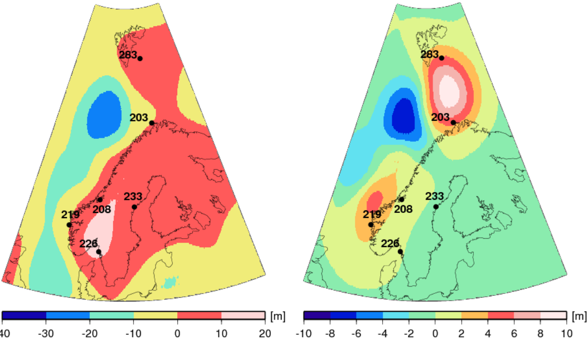
Figure 4: Colors denote the difference between RSL computed at LGM ( 26,000 years B.P. in the ICE-5G model ) and computed at present caused by GISR for sediment model Amantov2 (left) and Sed1 (right). Note the different color scales. Numbered black dots show the locations of Relative Sea Level data used in Fig. 7. Earth model M4-16-80 is used for both cases.
