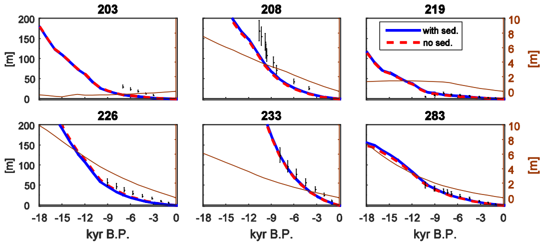
Figure 5: RSL at selected sites from the Tushingham and Peltier (1992) database, for the ICE-5G model (red dashed line) and the ICE-5G model with sediment transport (blue line) according to the Amantov2 model in combination with the M4-16-80 Earth model. The brown line shows the difference, with scale on the right y-axis.
