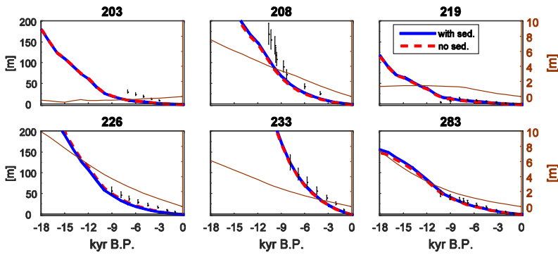
Figure 4: RSL at selected sites from the Tushingham and Peltier (1992) database, for the ICE-5G model (red dashed line) and the ICE-5G model with sediment transport (blue line) according to the Amantov 2 model in combination with the M4-16-80 Earth model. The brown line shows the difference, with scale on the right y-axis.
