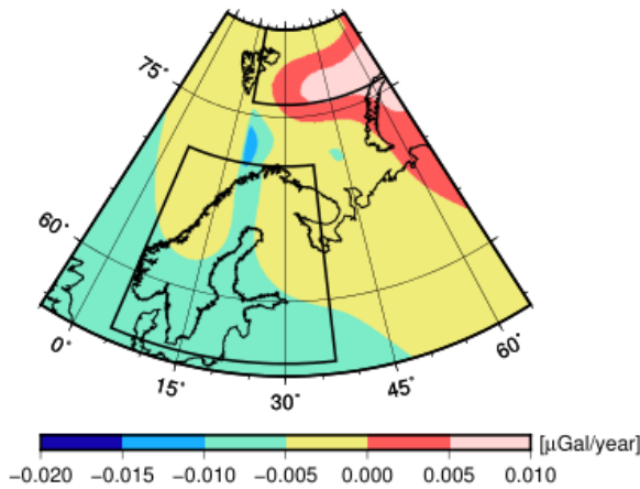
Figure 6: Gravity rate due to GISR according to the Amantov model for viscosity profile M4-16-80. Boxes in Scandinavia and the Barents Sea denote the areas for which the maximum gravity rate is given in Table 1.
