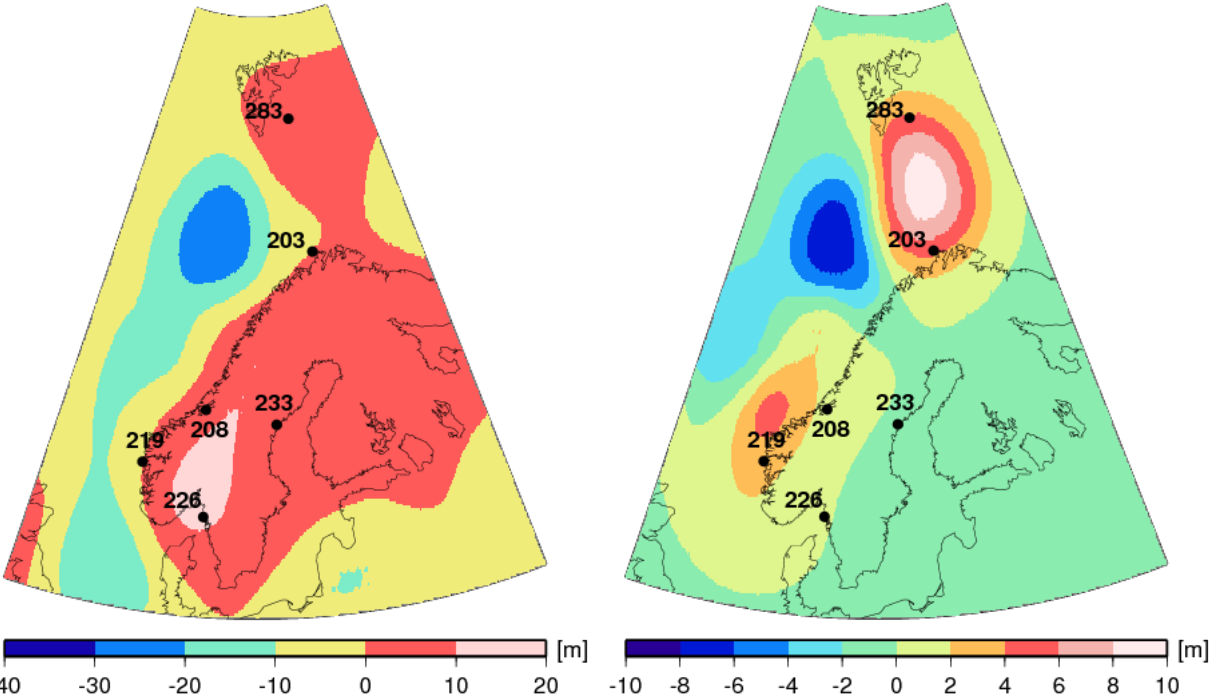
Figure 3: Colors denote the difference between RSL computed at LGM ( 26,000 years B.P. in the ICE-5G model ) and computed at present caused by GISR for sediment model Amantov2 (left) and Sed1 (right). Note the different color scales. Numbered black dots show the locations of Relative Sea Level data used in Fig. 7. Earth model M4-16-80 is used for both cases.
