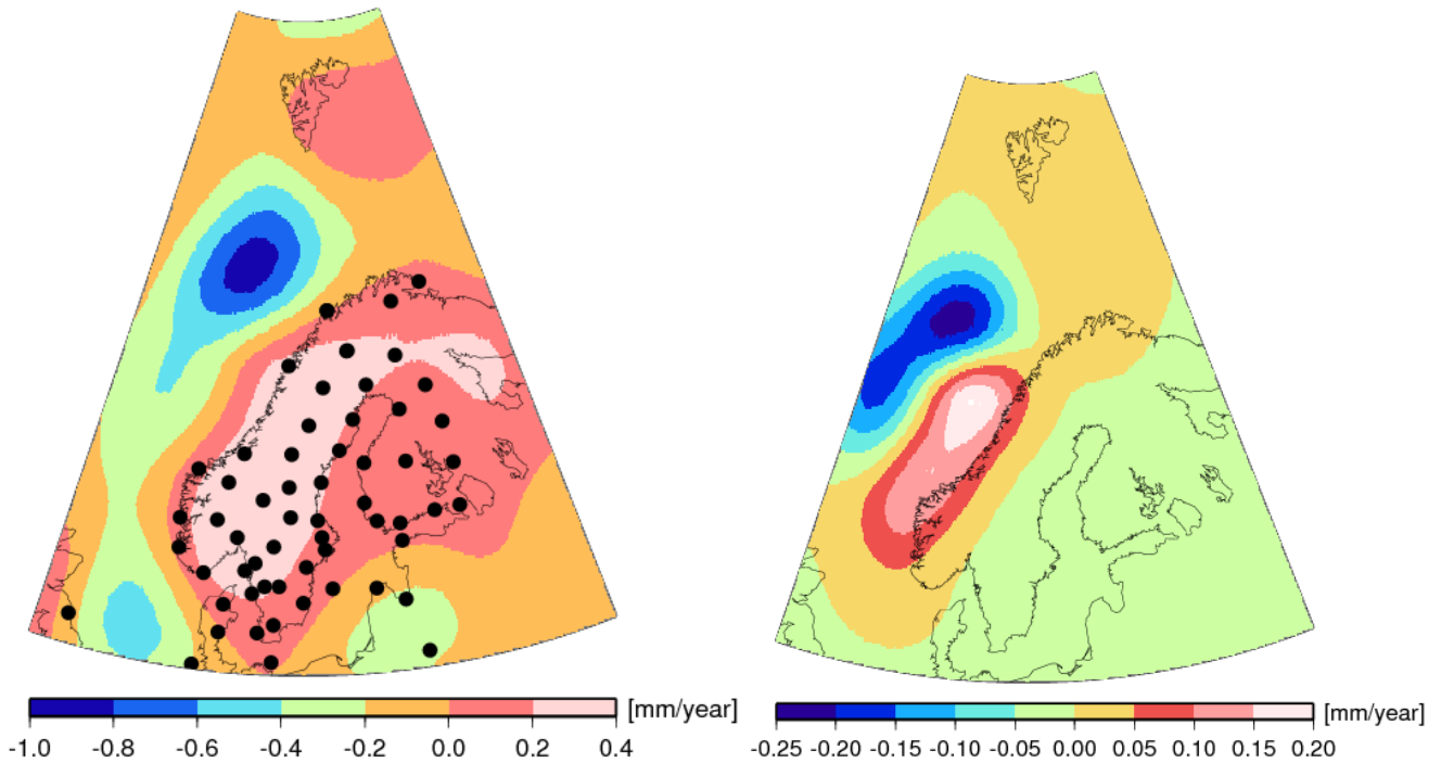
Figure 5: Uplift rates caused by sediment redistribution according to GISR models Amantov 12 (left) and Sed1 (right). Dots denote locations of GPS sites of Lidberg et al. (2010). Note the different color scales. Earth model M4-16-80 is used for both cases.
