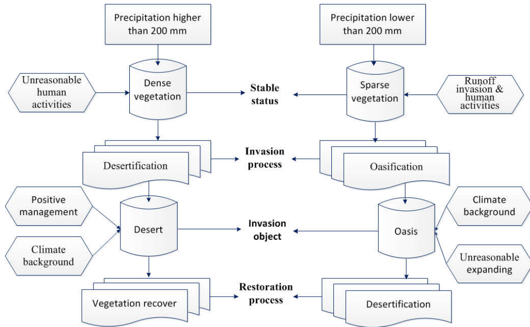
Figure 3 Schematic diagram to describe the desertification and oasisification processes in semi-arid and dry semihumid regions (a), and in arid or hyper-arid regions (b)
