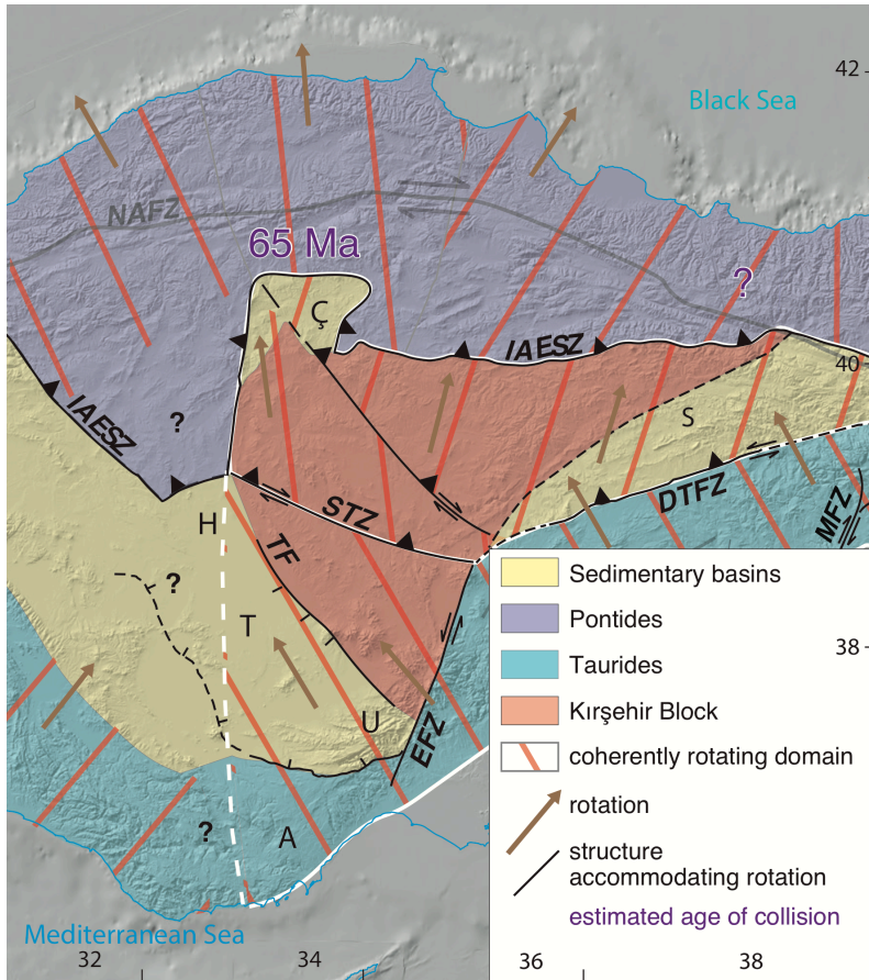
5 Figure 8: Coherently rotating domains within the Anatolian orogen and tectonic structures accommodating differential rotations. NAFZ - North Anatolian Fault Zone, IAESZ - Izmir-Ankara-Erzincan Suture Zone, STZ - Savcılı Thrust Zone, DTFZ - Deliler-Tecer Fault Zone, TF - Tuzgölü Fault, EFZ - Ecemiş Fault zone, Malatya Fault Zone (MFZ). Basins: U - Ulukışla, T - Tuzgölü, H - Haymana, A - Adana. Orange hatching indicates the amount of vertical axis rotation of each domain, whereby the hatching is rotated from N-S according to the paleomagnetic results summarized in Table 1 .
