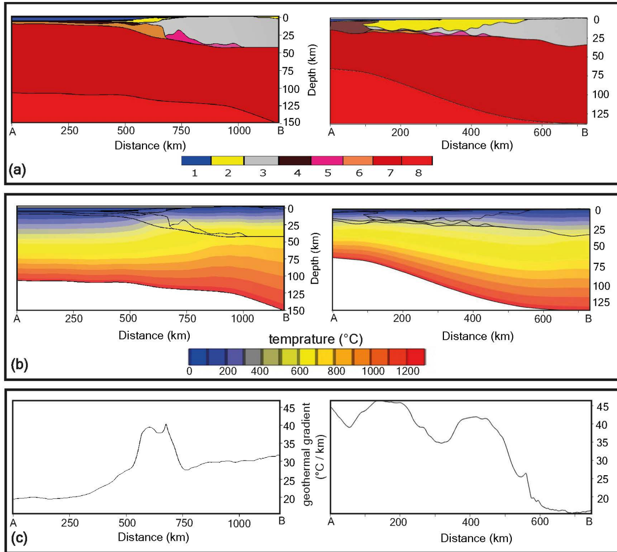
Figure 11. Structural-thermal cross section and corresponding average geothermal gradient at SW African passive margin (left) and Norwegian continental margin (right) after Scheck-Wenderoth et al. (2007); Scheck-Wenderoth and Maystrenko (2008); Maystrenko et al. (2013): (a) Structural crustal cross section along A–B profile (Fig. 4a and Fig. 7a). Numbers near color legend for individual layers: 1) water, 2) sediments, 3) crystalline continental crust, 4) oceanic crust, 5) high-density continental crust, 6) high-velocity high-density lower crustal layer, 7) low density mantle, 8) normal density mantle. (b) Temperature distribution within the A–B cross section. (c) Calculated average geothermal gradient along the A–B cross section.
