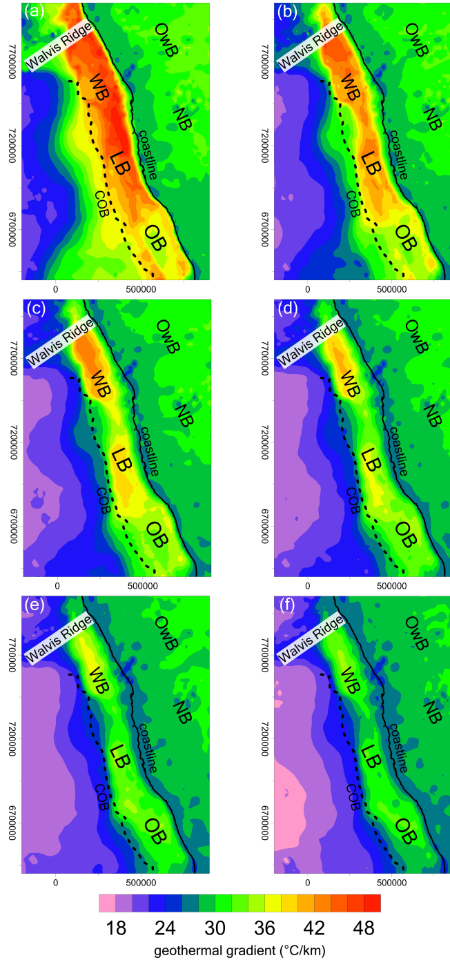
Figure 8. Geothermal gradient [ ^{\circ}\text{C}/\text{km} ] at SW African margin: the gradient calculated as the temperature differences between the uppermost surface (upper thermal boundary) and the corresponding temperature distribution at (a) 1, (b) 2, (c) 3, (d) 4, (e) 5, and (f) 6 km below the uppermost surface (COB: Continent-Ocean Boundary; Cretaceous-Cenozoic basins: WB: Walvis Basin, LB: Lüderitz Basin, OB: Orange Basin; Precambrian basins: OwB: Owambo Basin, NB: Nama Basin; UTM: WGS84, 33S).
