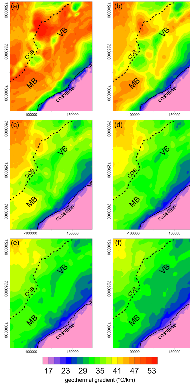
Figure 9. Geothermal gradient [ ^{\circ}\text{C}/\text{km} ] at Norwegian margin: the gradient calculated as the temperature differences between the uppermost surface (upper thermal boundary) and the corresponding temperature distribution at (a) 1, (b) 2, (c) 3, (d) 4, (e) 5, and (f) 6 km below the uppermost surface (COB: Continent-Ocean Boundary; Cretaceous-Cenozoic basins: VB: Vøring Basin, MB: Møre Basin; UTM: WGS84, 33N).
