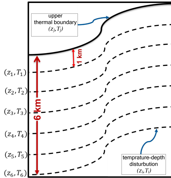
Figure 1. The geothermal gradient calculation: schematic of the temperature-depth distributions in 1 km homogeneous depth intervals down to 6 km below the upper thermal boundary surface to calculate the geothermal gradient between the uppermost surface ( z_j, T_j ) and the corresponding depth levels ( z_i, T_i ). The temperature-depth distribution maps are presented as figure 1 and 2 in the Supplement.
