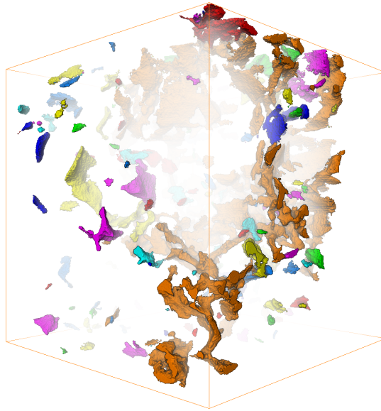
Figure 7. 3-dimensional rendering of cavities segmented from a nanotomographic dataset. Pores are coloured individually to highlight connectivity. This means that a single colour allows for the tracing out of pore connections. For example, note the large interconnected pore cluster in orange. Dimension of the cube is 700 \text{ voxel}^3 , with a voxel size of \sim 35 \text{ nm} . The top and base of the cube are parallel to the mylonitic foliation. The figure indicates the oblate shape of most cavities and proves that they are indeed 3-dimensional features.
