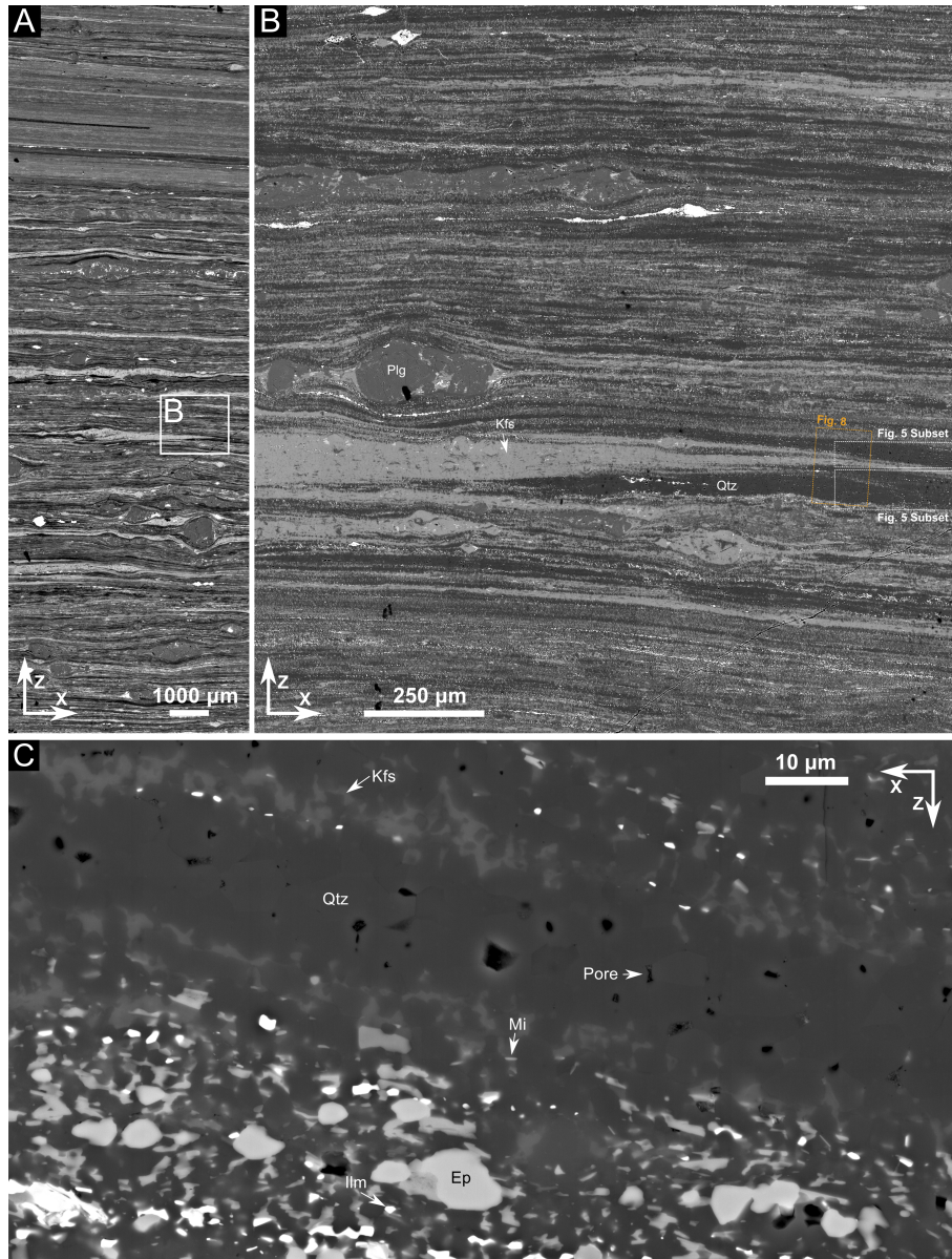
Figure 1. BSE images from the quartzo-feldspathic ultramylonite. Fig. 1a shows the overall strain gradient in the sample, with the highest strain domain found at the top of the image. Fig. 1b is a high-resolution BSE SEM mosaic of a representative area of the sample (41448 x 40282 pixels, scale of 1 px : 35.5 nm). All results presented for pore shape and orientation analysis are from the area of fig. 1b. The greyscale values identify minerals as follows: black = Porosity, dark grey = Qtz, grey= Plg, light grey = Kfs, bright = accessory phases. Fig. 1c presents the edge of a disaggregating quartz domain and highlights the minerals present in the poorly mixed polyphase domains.
