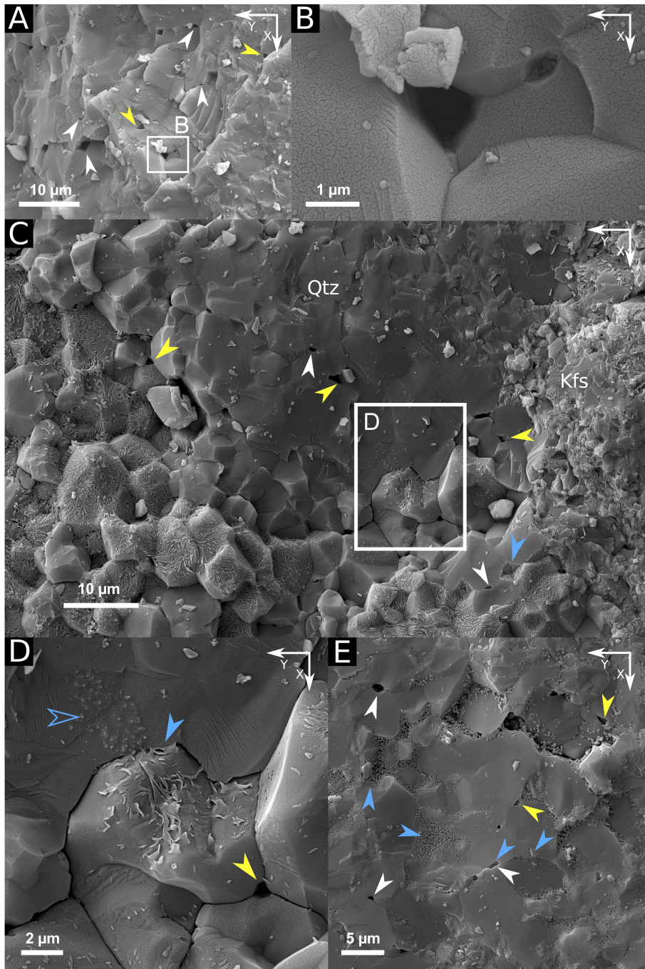
Figure 6. Secondary electron images from broken surfaces of quartz domains. White and yellow arrows point, respectively, to pores on grain-boundaries with a low angle to the YZ plane of finite strain and to pores at grain boundary trip junctions. Blue arrows highlight ‘precipitation’ features, with the empty blue arrow in fig. 6d identifying crystallites interpreted to be incipient precipitates found on a less dilatant grain boundary. Fig. 6a shows a thick, coherent, monomineralic quartz domain that has an abundance of pores. Fig. 6b highlights the difference between a pore found at a triple junction and a pore found in the middle of a grain boundary (see fig. 1c for comparison in XZ plane). Fig. 6c, d and e show the change in porosity and grain boundary features with increasing distance from a plagioclase porphyroclast (see text for more detail).
