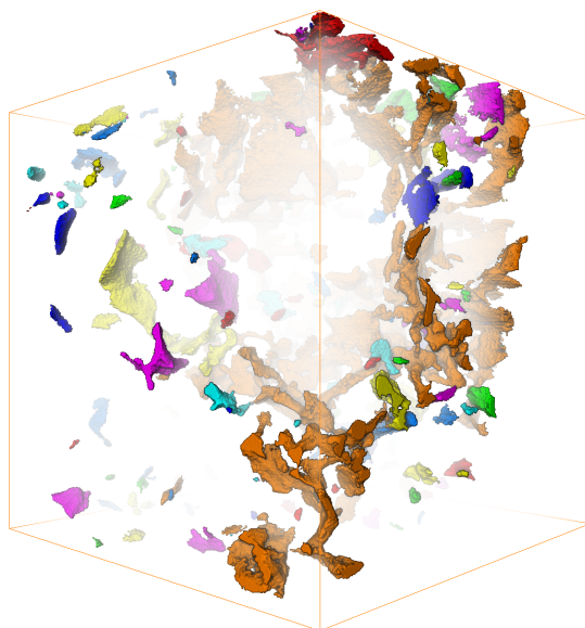
Figure 7. 3-dimensional rendering of cavities segmented from a nanotomographic dataset. Individual pores are coloured, note large interconnected pore cluster in orange. Dimension of the cube is 700 \text{ voxel}^3 , with a voxel size of \sim 35 \text{ nm} . The top and base of the cube are parallel to the mylonitic foliation. The figure indicates the oblate shape of most cavities and proves that they are indeed 3-dimensional features.
