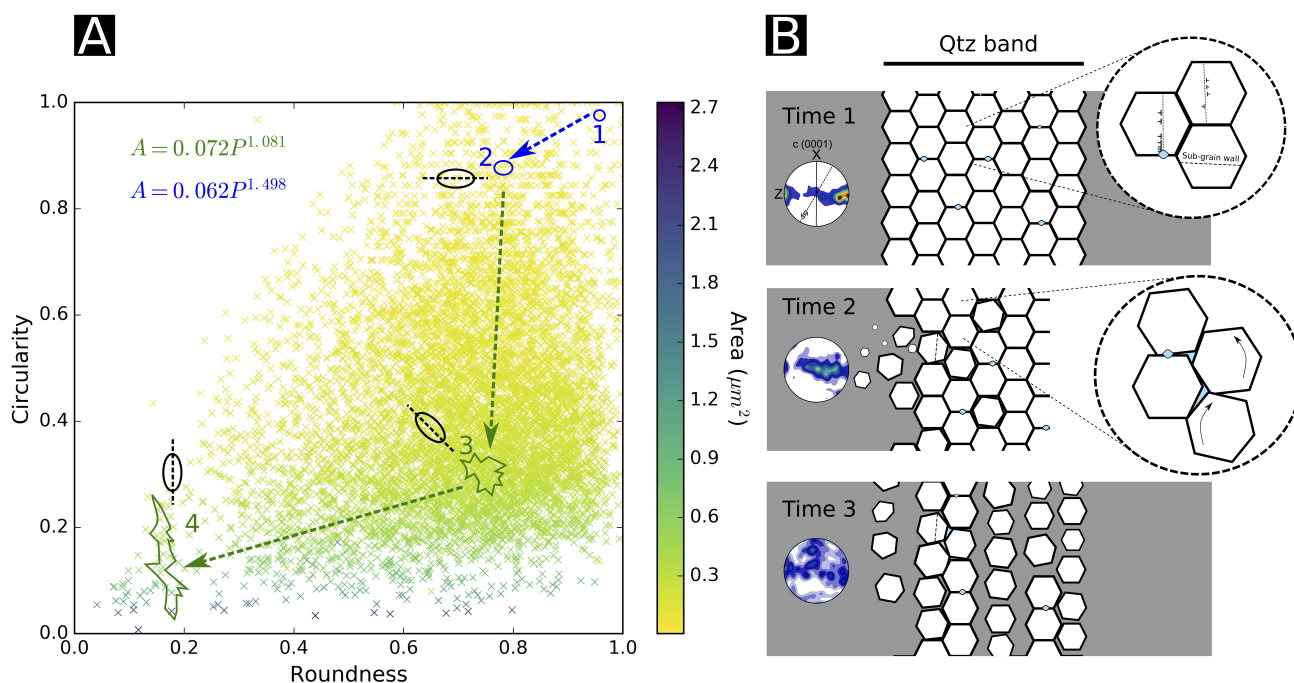
Figure 9. A model for synkinematic creep cavity formation by two different mechanism. Fig. 9a graphically represents the inferred trajectory of a creep cavity’s life cycle. Initially creep cavities grow from circular (1) to elliptical cavities (2). These cavities generally have long axes aligned in the Z direction (when viewed in the XZ plane). As cavities become larger they develop more complex shapes and rotate (3), ultimately elongating and becoming more aligned with the shear plane (4). Fig. 9b schematically integrates our observations of cavity evolution with the evolution of the microstructure and the associated micro-mechanisms. First cavities form, in quartz domains deforming by GSI creep, by the Zener-Stroh mechanism (fig. 9b, Time 1). As the grain boundary strength is weakened by the ingress of fluids into cavities, VGBS is promoted. This increase in the contribution of VGBS drives the production of new creep cavities of a more complex shape (fig. 9b, Time 2). It is the production of creep cavities that initiates the increased contribution of VGBS and ultimately prompts a switch to a GSS creep. See text for details.
