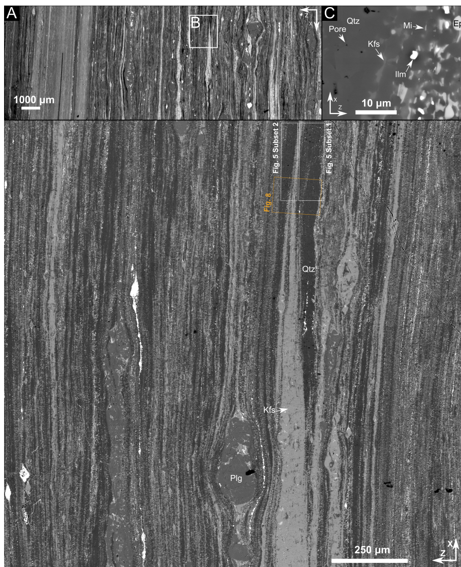
Figure 1. BSE images from the quartzofeldspathic ultramylonite. Fig. 1a shows the overall strain gradient in the sample, with the highest strain domain found on the left of the image. Fig. 1b is a high-resolution BSE SEM mosaic of a representative area of the sample (41448 x 40282 pixels, scale of 1 px : 35.5 nm). All results presented for pore shape and orientation analysis are from the area of fig. 1b. The greyscale values identify minerals as follows: black = Porosity, dark grey = Qtz, grey = Plg, light grey = Kfs, bright = accessory phases. Fig. 1c presents the edge of a disaggregating quartz domain and highlights the minerals present in the poorly mixed polyphase domains.
