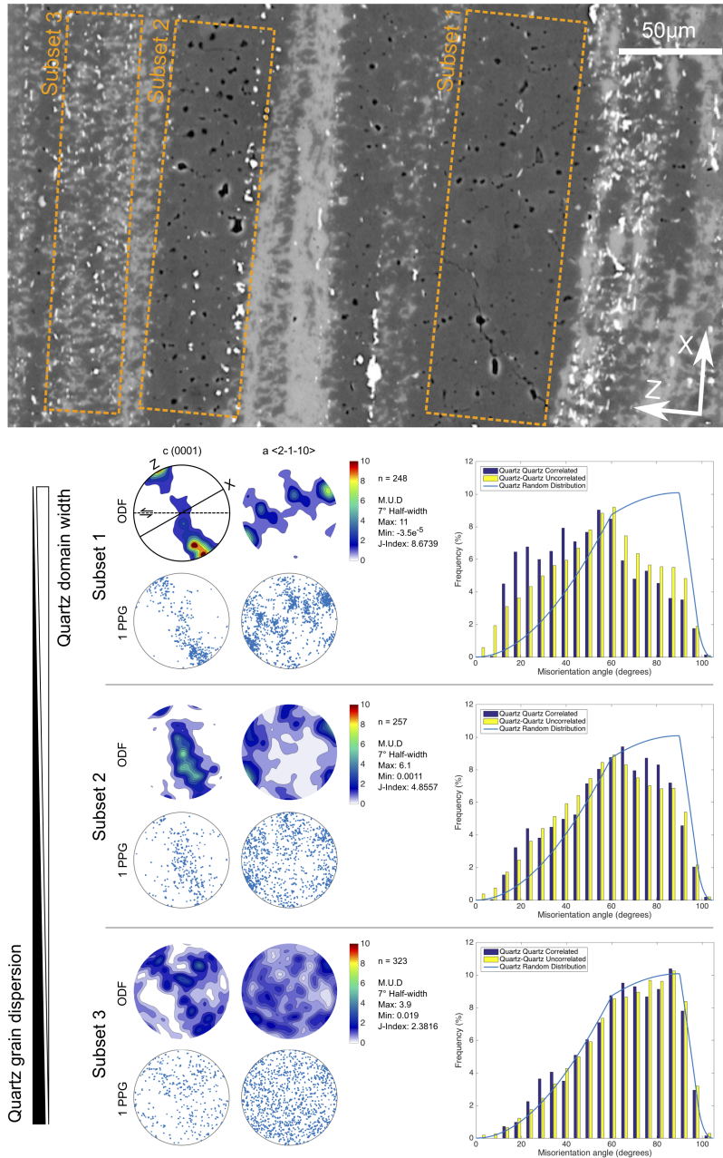
Figure 8. EBSD analyses of quartz domains. The EBSD analyses were performed in the same quartz bands used for subset image analysis (see fig. 1 and 5). EBSD data are presented in equivalent subsets corresponding to decreasing quartz domain width and increasing quartz dispersion. A clear CPO is observed in the pole figure analysis of subset 1 with two c(0001) maxima and two corresponding a\langle 2-1-10 \rangle maxima. As quartz domain thickness decreases there is a randomisation of the CPO, highlighted by the decrease in the J-Index and supported by the shift to a near random distribution of the misorientation angle histogram of subset 3.
