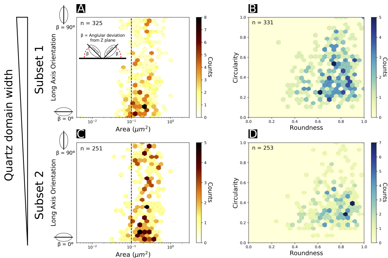
Figure 5. Pore analysis for subsets 1 and 2 shown in fig. 1b, corresponding to decreasing quartz domain width and increasing quartz dispersion. Fig 5a and c show that with decreasing quartz band thickness, there is an increase in the range of pore orientations observed. Fig. 5b and d demonstrate that this change is also concordant with a change in the pore shapes from roughly elliptical to more complex. More specifically, it can be seen in fig. 5b and d, that with decreasing domain width there is a loss of circular and elliptical pores.
