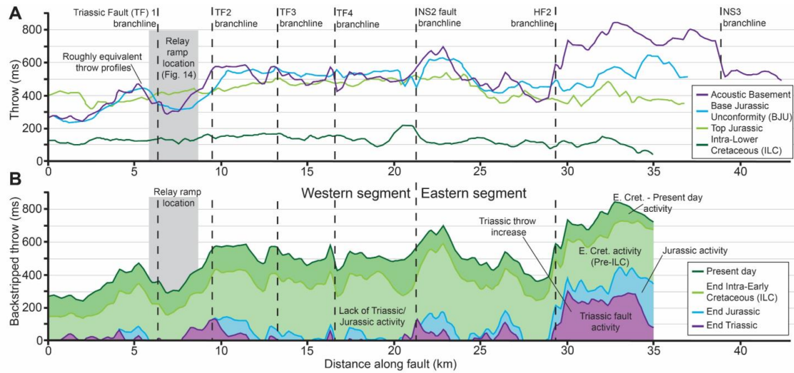
Figure 8. A) Throw-length profiles calculated for major stratigraphic horizons across the Fjerritslev South Fault showing the branchlines with cross-cutting faults. Note the similarity between the different stratigraphic horizons west of the HF2 branchline. B) Backstripped fault profile for the Fjerritslev South Fault showing Triassic activity east of the HF2 branchline but not elsewhere along the fault. Early Cretaceous fault activity is observed along the length of the fault.
