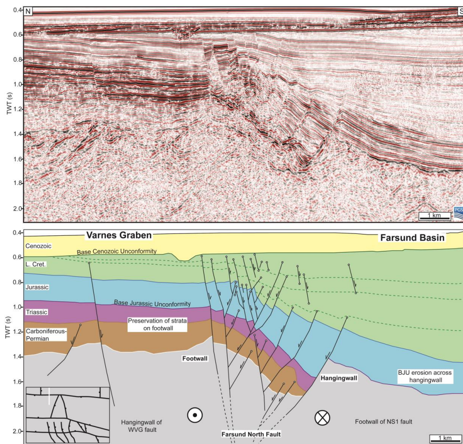
Figure 11. Interpreted and uninterpreted N-S oriented seismic section across the Farsund North Fault. Preservation of Carboniferous-Permian and Triassic strata across the footwall of the Farsund North Fault with concomitant erosion across the hanging wall represents the same hanging wall-footwall juxtaposition demonstrated in Fig. 10. See Fig. 1c, 10 for location.
