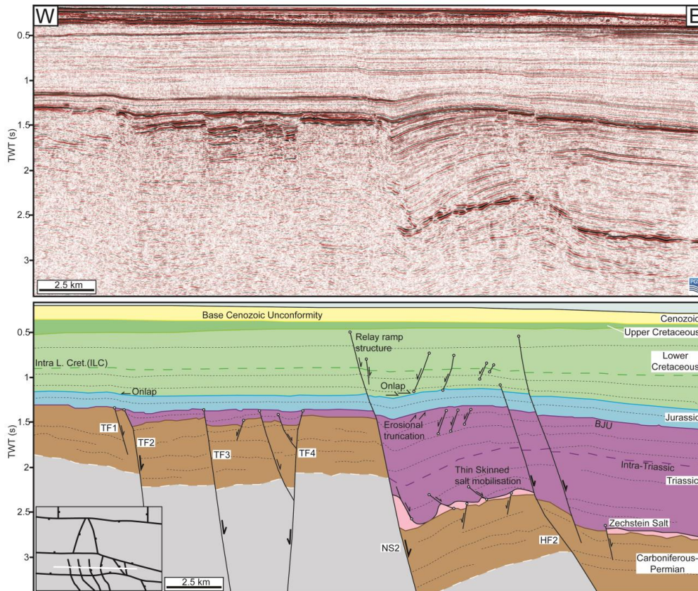
Figure 5. Uninterpreted and interpreted E-W oriented seismic section across the Farsund Basin. Triassic thickness changes are observed across N-S striking faults, with other stratigraphic intervals appearing largely isopachous. See Fig. 1c for location.
