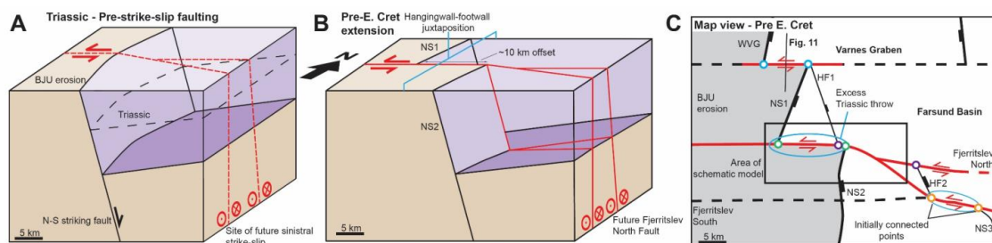
Figure 10. A) Schematic diagram showing Triassic activity along N-S striking faults. B) Schematic diagram showing the resultant fault geometries and associated hanging wall-footwall juxtaposition as a result of the sinistral offset of the N-S striking fault. C) Map showing the geometry of the strike-slip system within the Farsund Basin prior to the Early Cretaceous. Black box shows the location of the schematic model showing hanging wall-footwall juxtaposition, with blue ovals showing areas of excess Triassic throw (See Fig. 7, 8).
