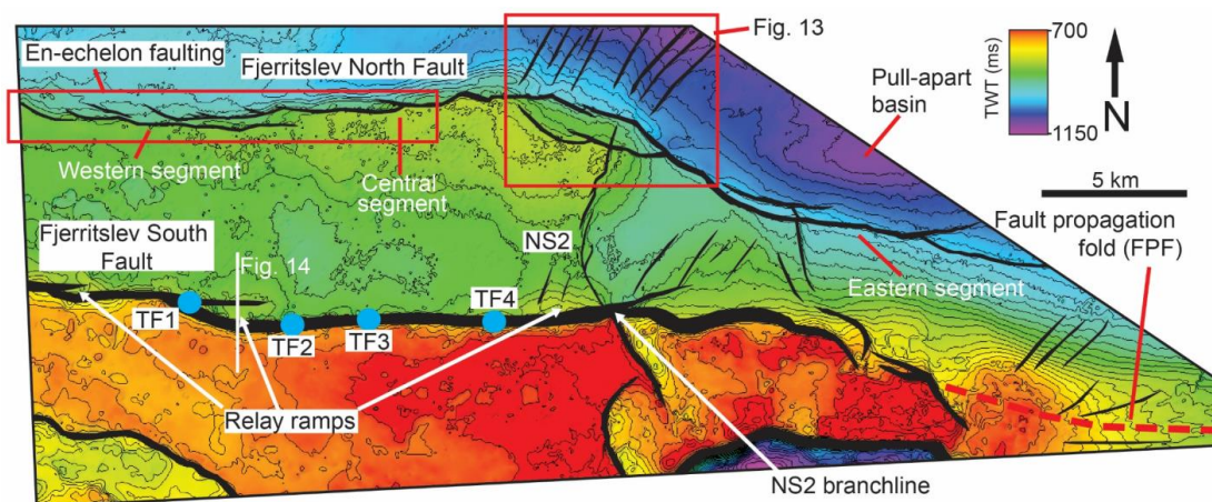
Figure 12. Two-way time structure map of the Intra-Lower Cretaceous horizon (see Fig. 4, 5 for surface in section). The Fjerritslev North Fault shows clear en-echelon segmentation along its western segment and a deepening of the surface in its hanging wall to the northeast. Intersections of underlying Triassic N-S striking faults with the Fjerritslev South Fault at deeper stratigraphic levels are indicated by blue circles.
