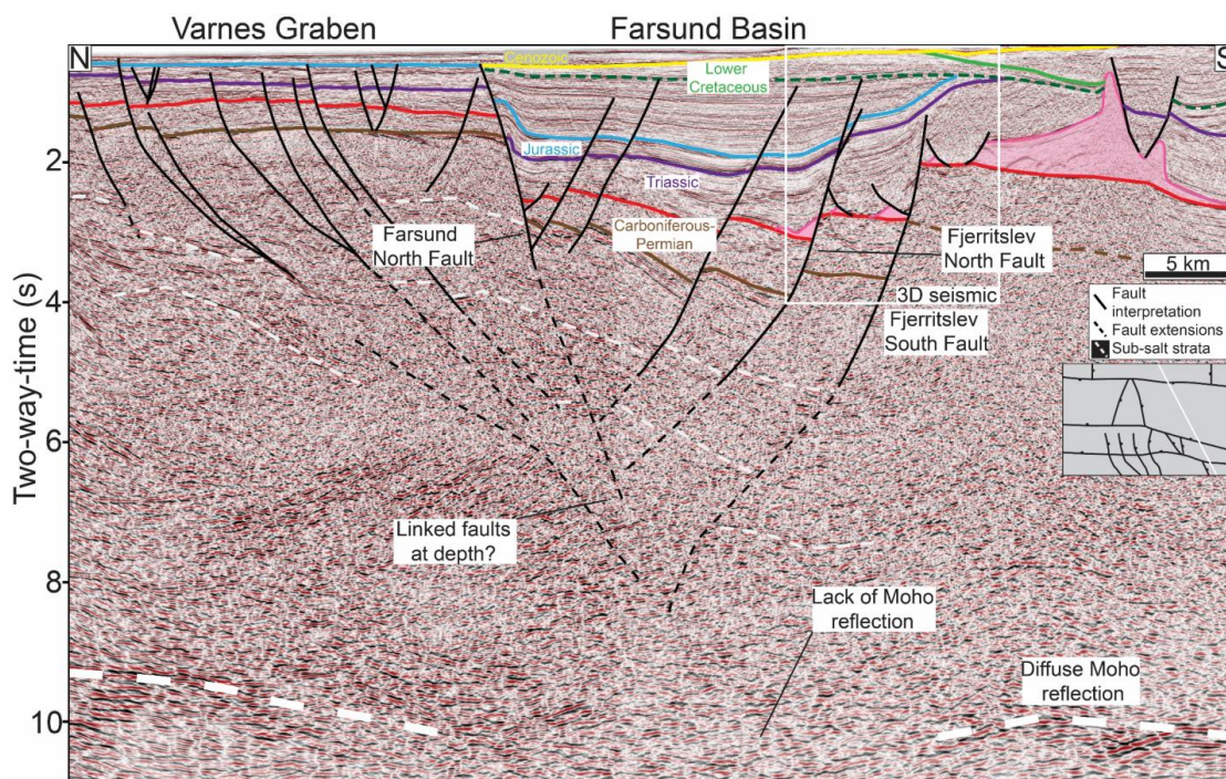
Figure 2. Interpreted N-S oriented seismic section across the Farsund Basin showing the linked and crustal-scale nature of the E-W oriented Basin bounding faults. The lack of Moho reflection directly beneath the basin may imply that the fault cross-cut the Moho in this area and extend through the crust. See Fig. 1c for location.
