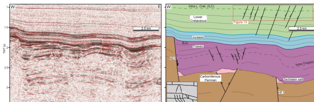
1005 Figure 9. Interpreted and uninterpreted E-W oriented seismic section located across NS1 and within the hanging wall of the Fjerritslev North Fault. Triassic activity occurs across NS1, with little Early Cretaceous activity observed. Note the geometric similarities between NS1 and HF1 on this section, and NS2 and HF2 on Fig. 5. See Fig. 1c for location.
