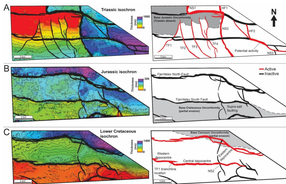
Figure 6. A) Isochron showing thickness of the Triassic interval and the associated faults active during this interval based on sediment thickness changes and depocentres. B) Isochron of Jurassic strata showing thickness and the faults that appear to have been active during this interval. C) Isochron of Lower Cretaceous strata showing the faults that appeared to be active during this interval.
