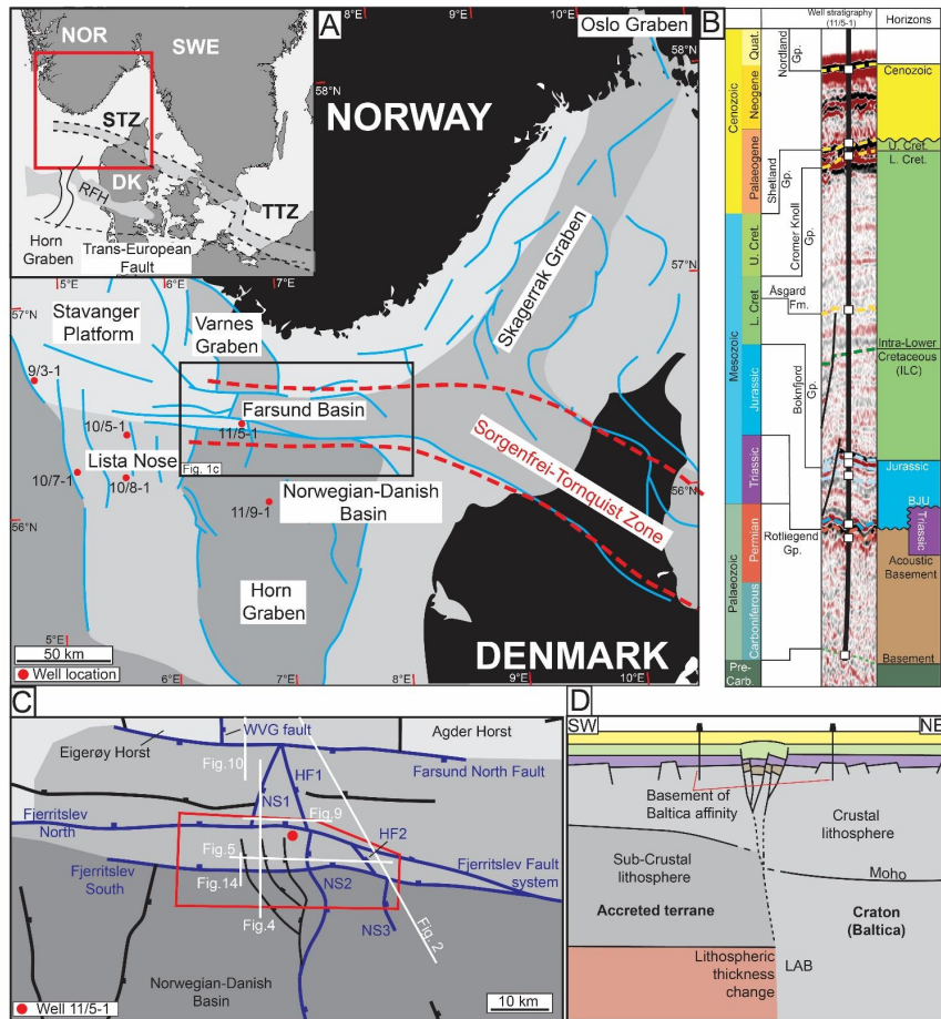
Figure 1. A) Regional map of the study area showing the relation to the major structural elements and fault networks. Well locations used to constrain ages of stratigraphic horizons are shown in red. Inset – Regional map of the area showing the location and geometry of the Tornquist Zone, along with major crustal-scale structural elements. B) Stratigraphic column showing the stratigraphy encountered in well 11/5-1 (located within the 3D volume), and the major tectonic events to have affected the region. C) Map showing the faults networks present across the Farsund Basin (those referred to in the text shown in blue), the location of the 3D seismic volume, and the main figures used throughout the study. D) Schematic cross-section showing the Sorgenfrei-Tornquist Zone as defined at both upper crustal and sub-crustal depths, and the potential relationship between the two.
