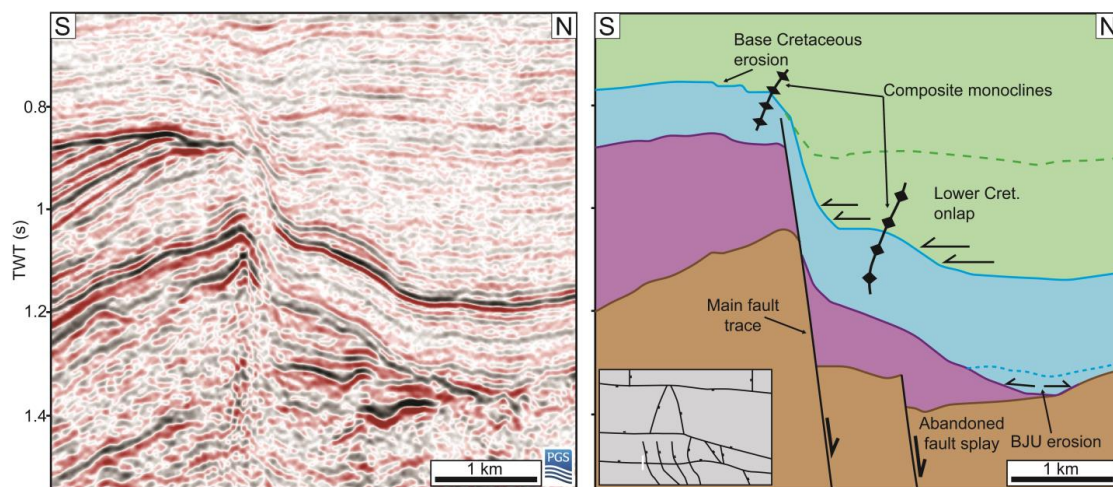
Figure 14. Interpreted and uninterpreted N-S oriented seismic section across the Fjerritslev South Fault. Section shows the presence of a composite monocline and associated underlying relay ramp.
