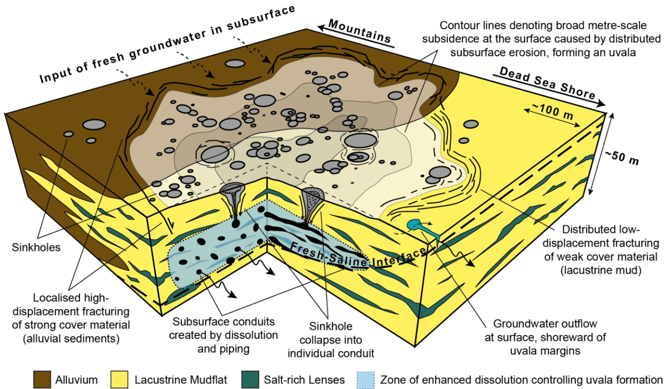
Figure 10: schematic depiction of the observed landforms and inferred subsurface processes governing the formation of sinkholes and uvalas in the evaporite karst setting of the Dead Sea.
