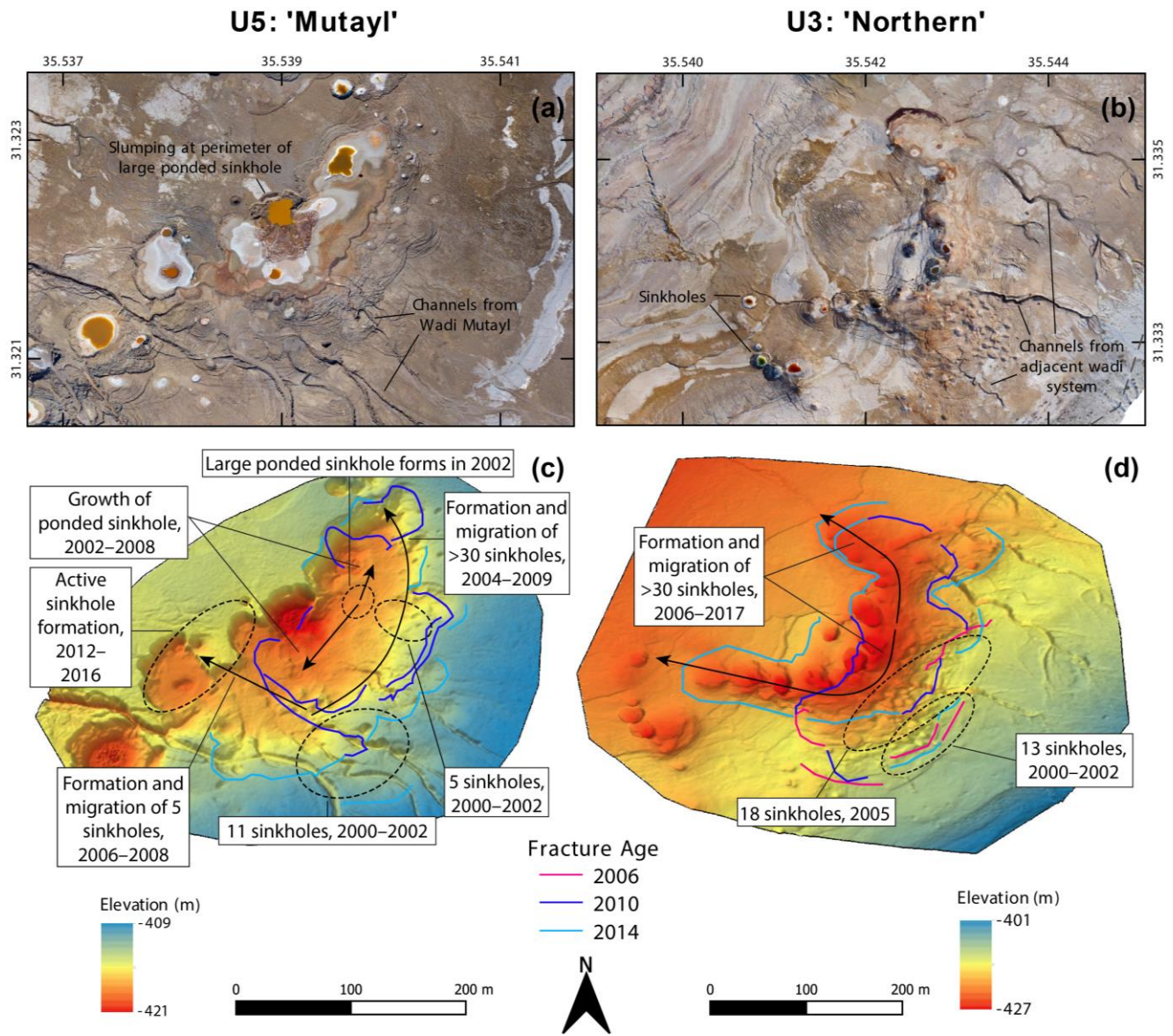
Figure 7: Structural development of uvalas U5 and U3 with unclear connection to subsurface water flow. See figure 4 for locations. (a) and (b) show orthophoto images from 2016; (c) and (d) show oblique 3D views of the depressions derived from the 2016 DSM. The main depression-bounding fractures are shown, whose years of formation of (i.e. when first visible in imagery) are coloured in four-year intervals.
