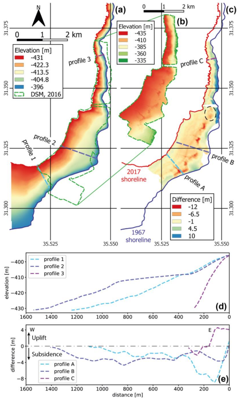
775 Figure 3: (a) bathymetric contour map of the relief of the former lakebed (top left), with an inset (b) of the 2016 DSM relief and elevation profiles 1-3 (as in Figure 3) plotted second from bottom. (c) map of elevation difference between the former lakebed bathymetry and the 2016 topography. (d) plot of elevation vs distance along profiles 1-3 as labelled in (a). (e) plot of elevation difference vs distance along profiles A-C as labelled in (c). Areas of significant subsidence are identifiable by the large negative difference (see 0-300m along profile A). There is subsidence of between 0-6m on the kilometre-scale in the southern part of the study area (profiles A and B), with subsidence of 0-3m on a smaller scale in the northern part of the study area (profile C). The dashed black ellipse indicates a zone of developing uvala-like subsidence referred to in section 4.4.
