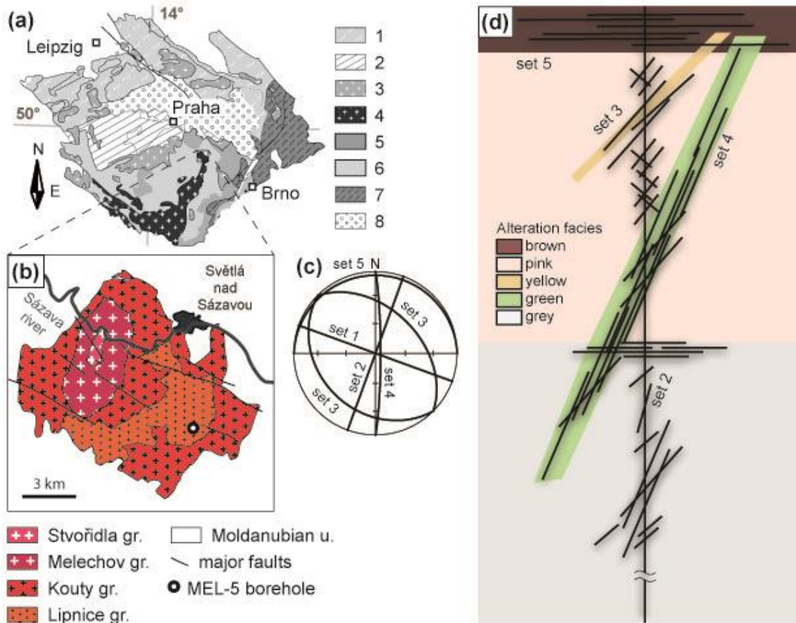
Figure 1: Maps showing the location of the sampled borehole. (a) simplified geological map of the Bohemian Massif (modified after Franke 2000), 1 - Saxothuringian and Lugian, 2 - Teplá-Barrandian, 3 - Variscan granitoids, 4 - Moldanubian Batholith, 5 - Gföhl assemblage, 6 - Drosendorf and Ostrong assemblage, 7 - Brunovistulian, 8 - Cretaceous sedimentary cover, (b) geological map of the Melechov pluton (modified after Machek 2011), gr., granite, u., unit-, (c) stereoplot (Schmidt projection) of the fracture sets recognized within the Melechov pluton, based on Lexa & Schulmann (2006) and Staněk (2013), (d) interpretative schematic sketch of the fracture sets and their structural relationship with respect to the alteration facies distribution within the borehole.
