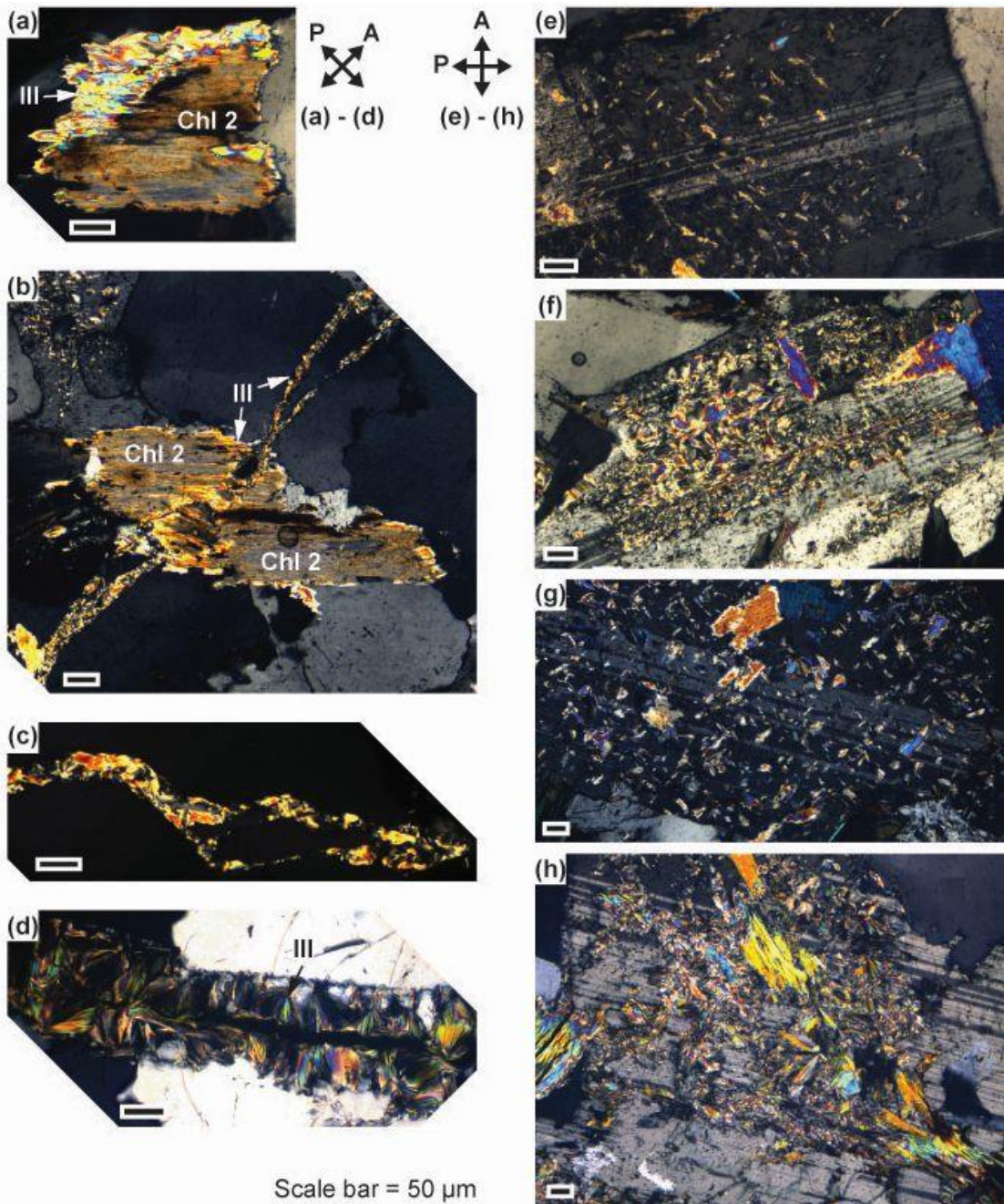
5 Figure 6: Polarized light photomicrographs showing microstructural position of illite. The double-headed arrows show polarization direction of polarizer (P) and analyzer (A). Partial chlorite (Chl 2) illitization unrelated (a) and related (b) to illite-filled crack (c) in green granite, (d) illite-filled crack in yellow granite, (e) isolated grains of illite in the core of plagioclase in fresh granite, (f) connected fan-shaped aggregates of illite aligned with plagioclase cleavage in green granite, (g) isolated grains of illite homogeneously distributed in plagioclase in brown granite, (h) aggregates of illite in plagioclase in yellow granite. Ill, illite.
