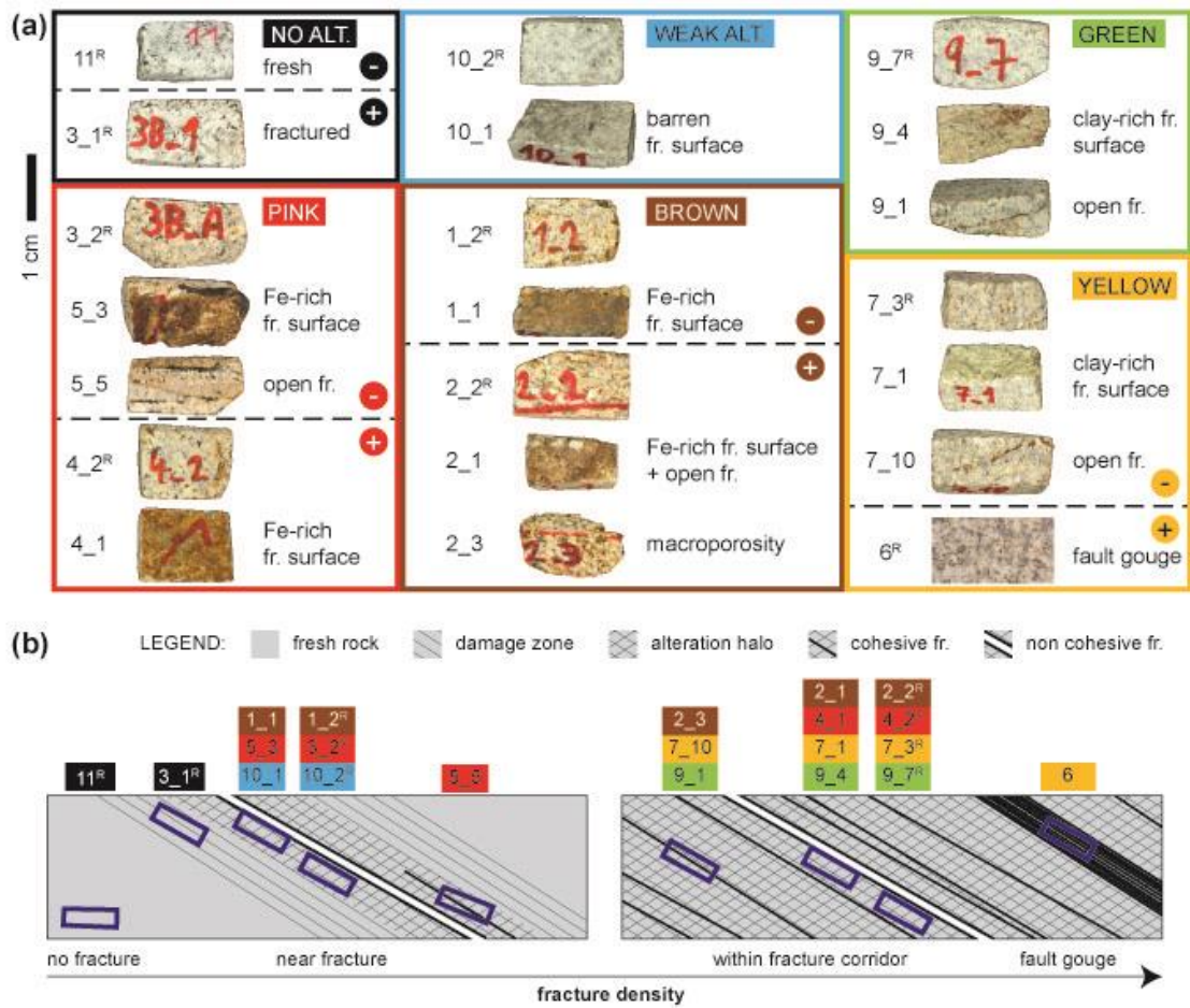
Figure 43: Photographs and parametric description of specimens tested by mercury porosimetry grouped by alteration facies . The dashed lines delimit subgroups of specimens from lower (minus symbol) and higher (plus symbol) fracture density zones. (b) Schematic sketch of rock cores and sampled materials showing in a simplified way the position of the specimens within the core samples. Specimens indexed with “R” were selected as representative of the matrix of the facies. Alt., alteration, fr., fracture, coh., cohesive.
