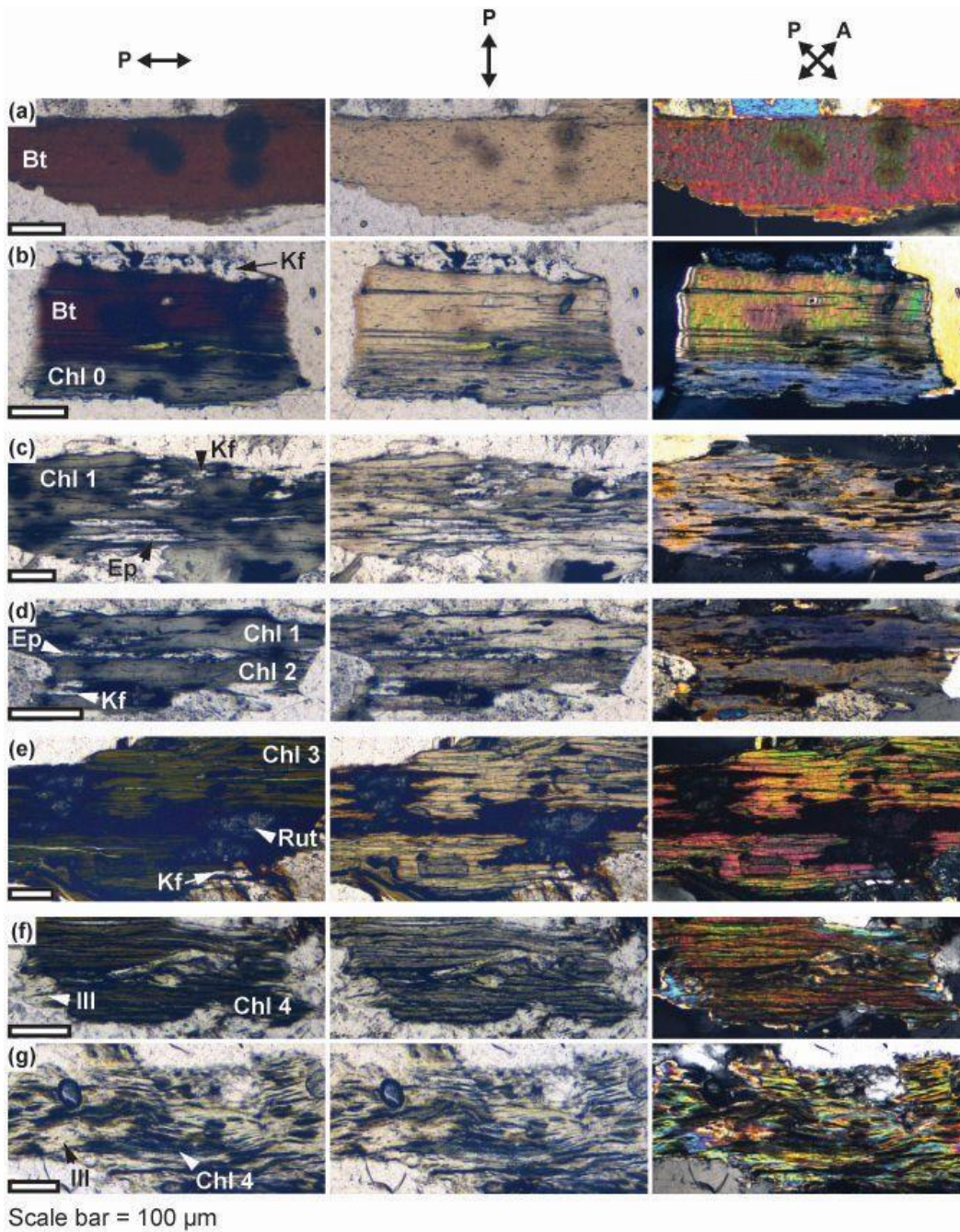
Figure 5: Polarized light photomicrographs showing optical properties of biotite and of its alteration products. The double-headed arrows show polarization direction of polarizer (P) and analyzer (A) for each column. (a) biotite and (b) biotite partially replaced by chlorite (Chl 0) in fresh granite, (c) chlorite (Chl 1) in weakly altered granite, (d) chlorite (Chl 1 and Chl 2) in green granite, (e) chlorite (Chl 3) in brown granite, (f, g) chlorite (Chl 4) and illite in yellow granite. Bt, biotite, Kf, K-feldspar, Ep, epidote, Rut, rutile, Ill, illite.
