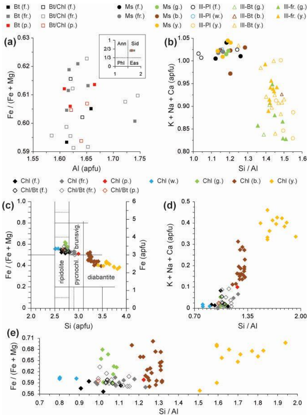
Figure 8: Chemical composition of analyzed minerals. (a) biotite (Bt) and biotite lamella in chloritized biotite (Bt/Chl), (b) muscovite (Ms), illite in plagioclase (Ill-Pl), in pseudomorph after biotite (Ill-Bt) and in fracture (Ill-fr.), (c, d, e) chlorite (Chl) and chlorite lamellae in chloritized biotite (Chl/Bt), (c) classification diagram after Hey (1954). Atoms per formula unit (apfu) calculated based on 11O (a, b) and 14O (c, d, e). Facies: f., fresh, fr., fractured, p., pink, g., green, b., brown, y., yellow, w., weakly altered. Ann, annite, Sid, siderophyllite, Phl, phlogopite, Eas, eastonite, brunsvig., brunsvigite, pycnochl., pycnochlorite.
