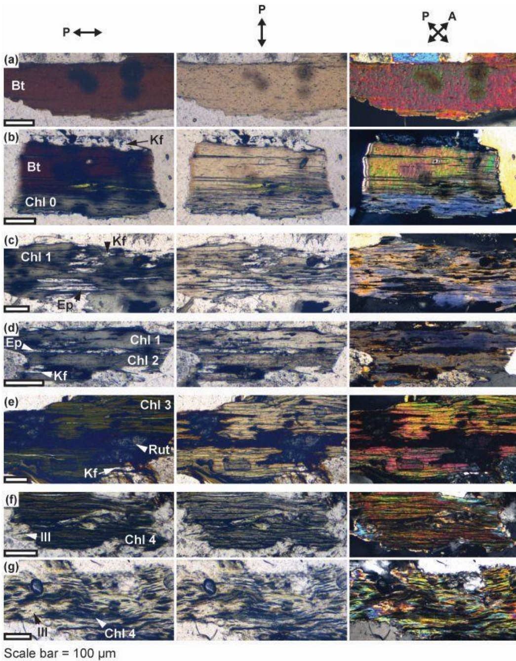
5 | Figure 5: Polarized light photomicrographs showing optical properties of biotite and of its alteration products. The double-headed arrows show polarization direction of polarizer (P) and analyzer (A) for each column. (a) biotite and (b) biotite partially replaced by chlorite (Chl 0) in fresh granite, (c) chlorite (Chl 1) in weakly altered granite, (d) chlorite (Chl 1 and Chl 2) in green granite, (e) chlorite (Chl 3) in brown granite, (f, g) chlorite (Chl 4) and illite in yellow granite. Bt, biotite, Kf, K-feldspar, Ep, epidote, Rut, rutile, Ill, illite.
