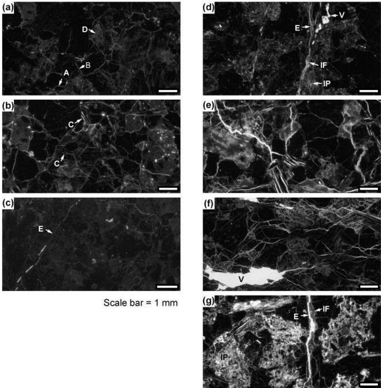
Figure 7: UV-fluorescent light photomicrographs showing microstructural position of connected porosity. Representative situations for fresh granite and pink granite near single fracture (a), for fractured and weakly altered granite (b), for pink granite in fracture corridor (c), for green granite (d), for brown granite near single fracture (e), for brown granite in fracture corridor (f) and for yellow granite in fracture corridor (g). D, distributed porosity in plagioclase, B, grain boundary crack, A, intragranular crack, C, cleavage crack, E, intergranular crack, V, cavity, IF, illite infills in fracture, IP, illite aggregate in plagioclase.
