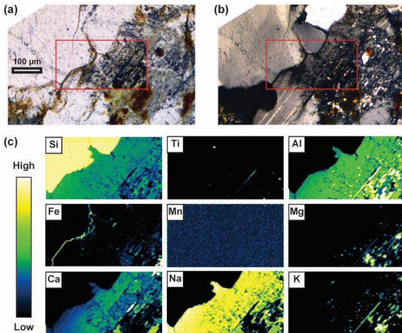
Figure 9: Microphotographs and elemental maps showing the Fe-rich material filling fractures in the pink granite. (a) polarised light, (b) cross-polarised light, (c) elemental maps for the region delimited by the red rectangle in (a) and (b).
