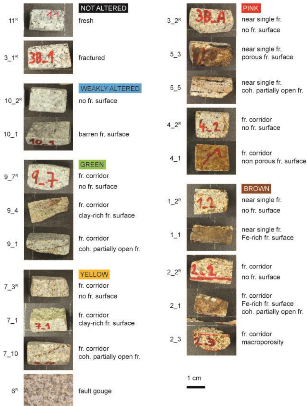
Figure 4: Photographs and parametric description of specimens tested by mercury porosimetry. Specimens indexed with “R” were selected as representative of the matrix of the facies. fr., fracture, coh., cohesive.
