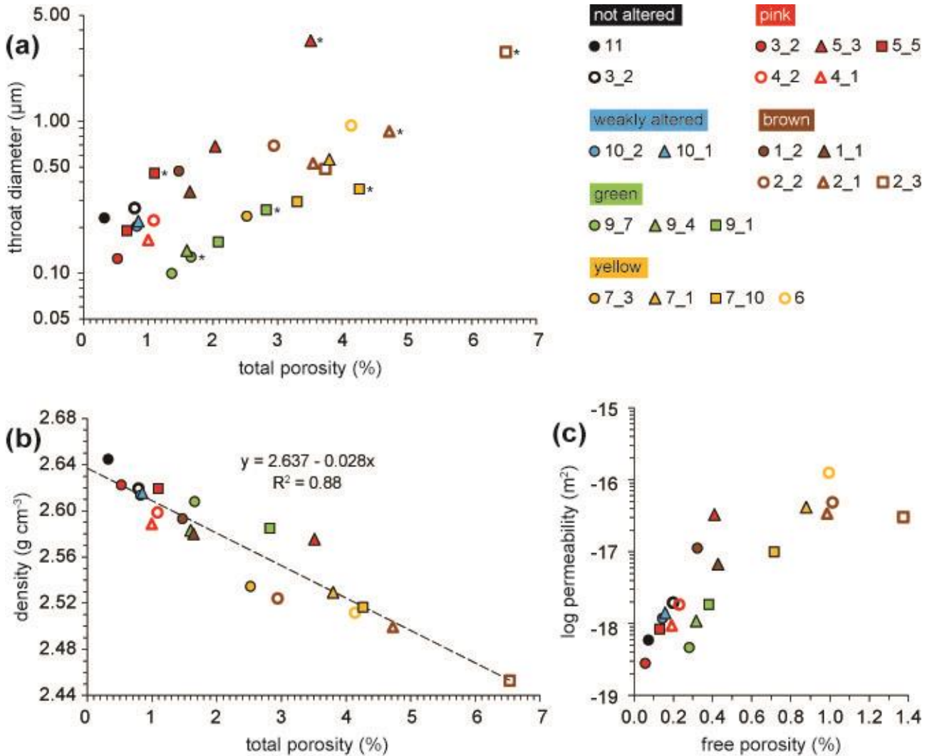
5 Figure 11: Plots of measured throat diameter, porosity and density and calculated permeability. (a) volumetric median throat diameter versus total porosity. For all specimens the values were calculated for throat diameter interval 0.005 - 5 \mu\text{m} and for specimens with macroscopic voids also for interval 0.005 - 300 \mu\text{m} (denoted by asterisk to the right from the marker). (b) bulk density versus total porosity. Total porosity calculated for throat diameter interval 0.005 - 5 \mu\text{m} and 0.005 - 300 \mu\text{m} for specimens without and with macroscopic voids, respectively. (c) permeability calculated after Katz & Thompson (1986, 1987) from the total porosity and median throat diameter (calculated for throat diameter interval 0.005 - 5 \mu\text{m} ) versus free porosity measured by mercury reintrusion (failed for specimen 7_3).
