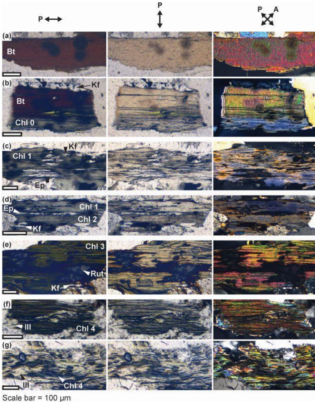
5 Figure 5: Polarised light photomicrographs showing optical properties of biotite and of its alteration products. The double-headed arrows show polarisation direction of polariser (P) and analyser (A) for each column. (a) biotite and (b) biotite partially replaced by chlorite (Chl 0) in fresh granite, (c) chlorite (Chl 1) in weakly altered granite, (d) chlorite (Chl 1 and Chl 2) in green granite, (e) chlorite (Chl 3) in brown granite, (f, g) chlorite (Chl 4) and illite in yellow granite. Bt, biotite, Kf, K-feldspar, Ep, epidote, Rut, rutile, Ill, illite.
