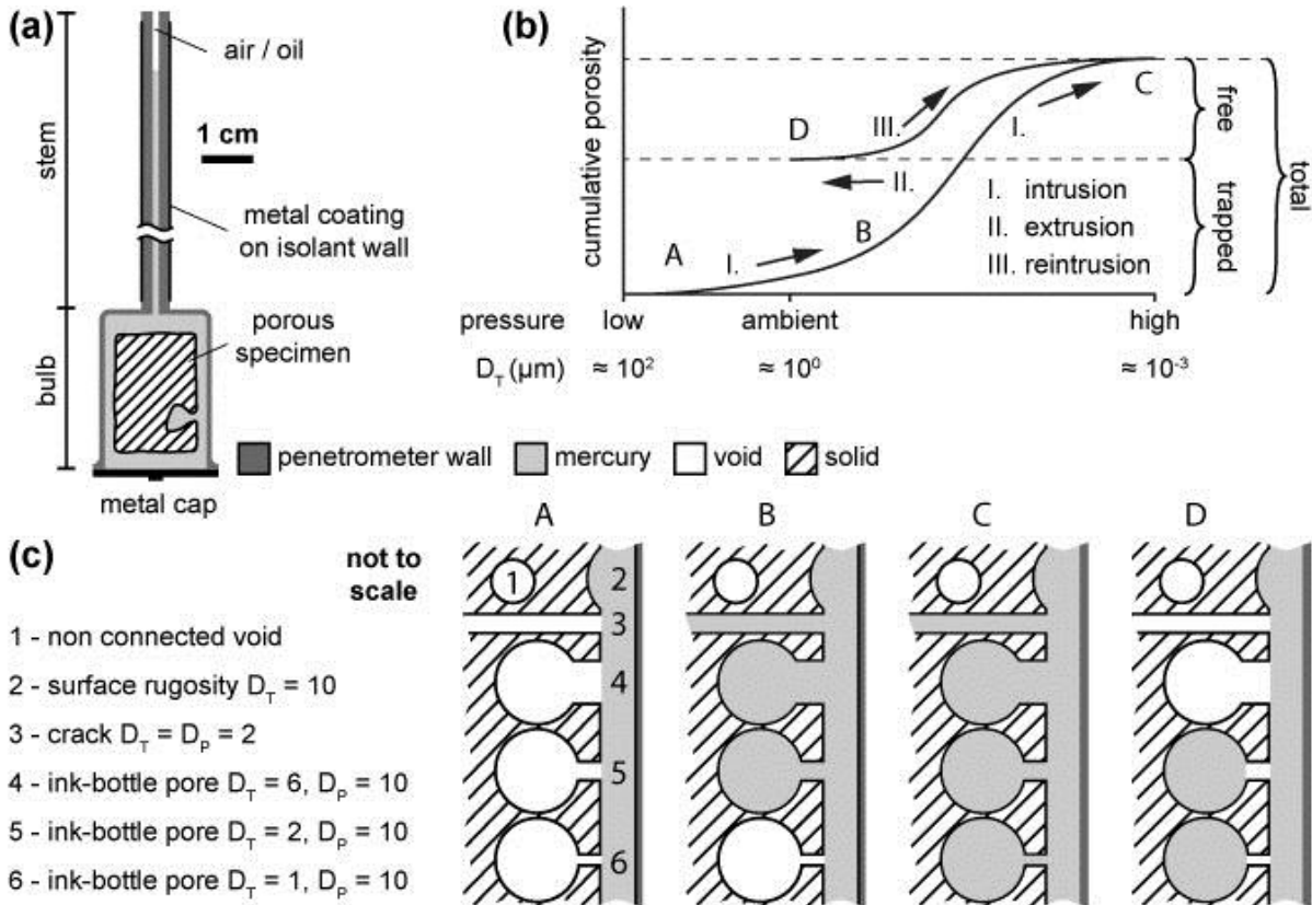
Figure 3: Mercury porosimetry. (a) schematic drawing of a penetrometer (specimen holder), (b) plot of an idealised cumulative porosimetric curve to explain the measurement of connected total, trapped and free porosity by mercury reintrusion, A-D relate to (c), (c) schematic drawings of void spaces in a rock specimen to explain the phenomenon of mercury entrapment with respect to different arrangements of throats in relation to pores. D_T , throat diameter, D_p , pore diameter.
