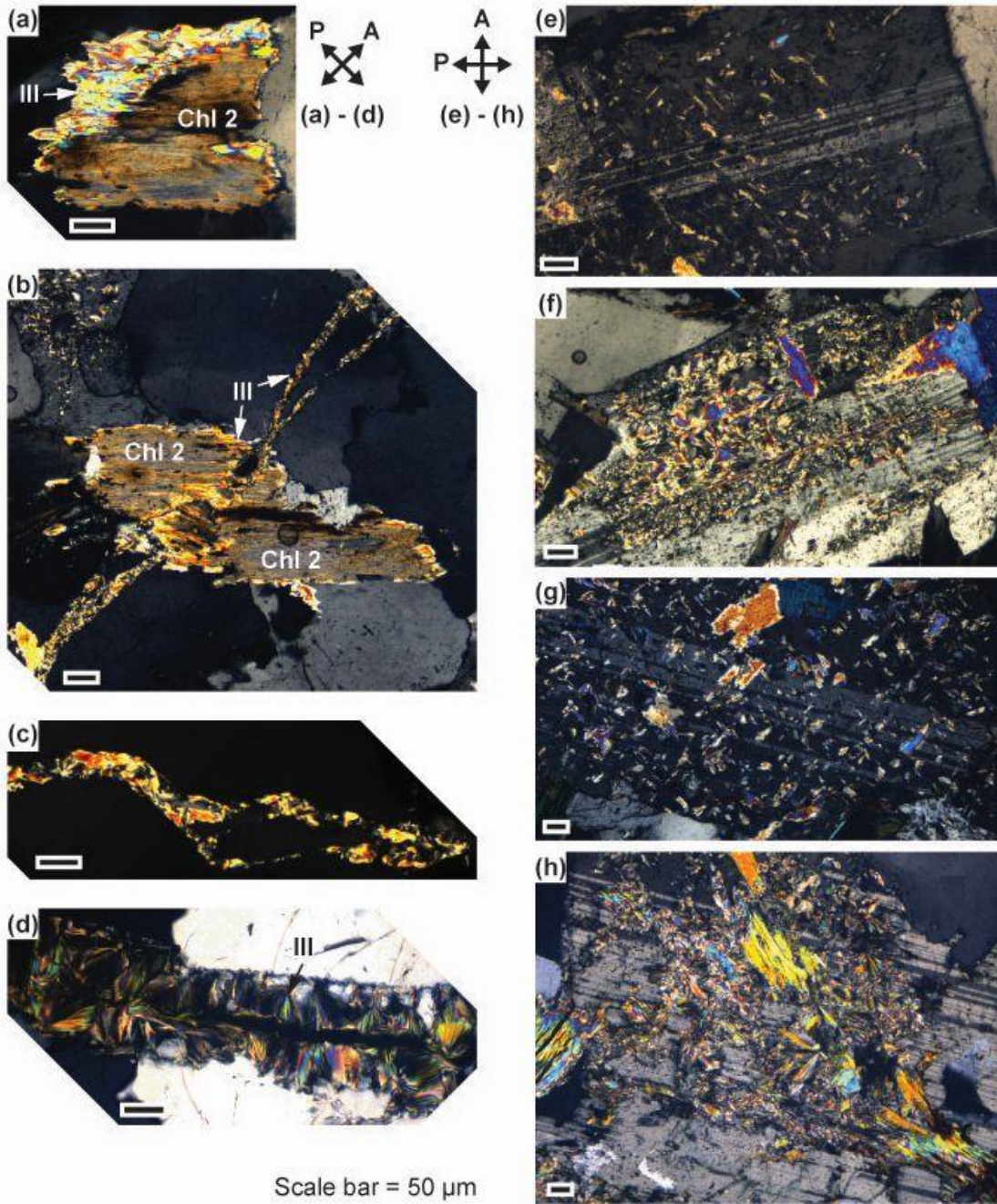
Figure 6: Polarised light photomicrographs showing microstructural position of illite. The double-headed arrows show polarisation direction of polariser (P) and analyser (A). Partial chlorite (Chl 2) illitisation unrelated (a) and related (b) to illite-filled crack (c) in green granite, (d) illite-filled crack in yellow granite, (e) isolated grains of illite in the core of plagioclase in fresh granite, (f) connected fan-shaped aggregates of illite aligned with plagioclase cleavage in green granite, (g) isolated grains of illite homogeneously distributed in plagioclase in brown granite, (h) aggregates of illite in plagioclase in yellow granite. Ill, illite.
