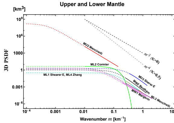
Figure 4. 3D PSDF vs. wavenumber for the upper and lower mantle. See labels in Table 3.
