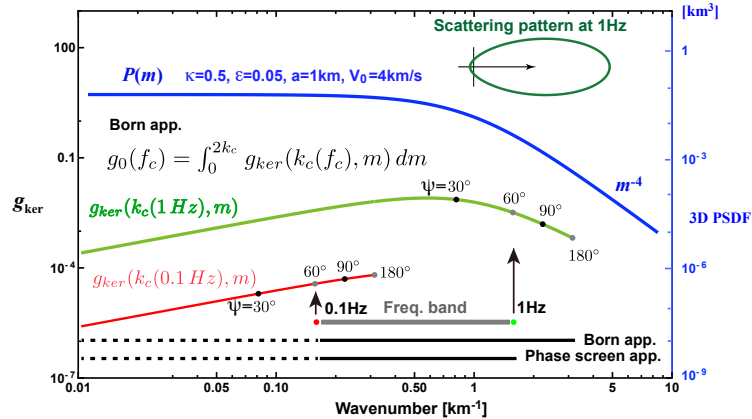
Figure 7. Plot of P(m) (blue, right scale) and the spectral kernel of the scattering coefficient g_{ker}(k_c(f_c), m) at f_c=0.1 Hz (red, left scale) and 1 Hz (green, left scale) according to the Born approximation. Scattering angles are marked by dots on each trace. For the case of frequency band between 0.1 and 1 Hz, the phase screen approximation based on the parabolic approximation covers the wavenumber range from 0 to the upper bound (line at the bottom), however, the Born approximation covers the range from 0 to twice the upper bound (line next to the bottom). We use those line styles in Figures 3~5 and 9.
