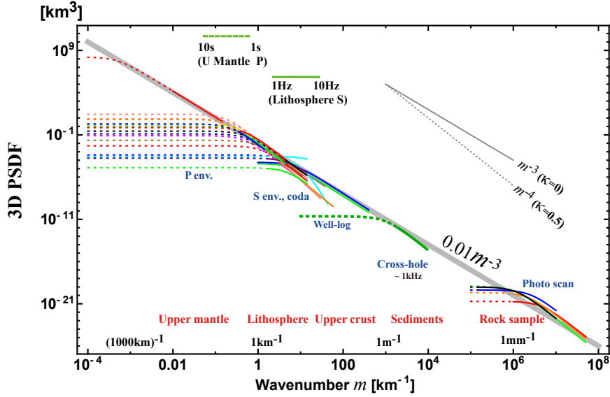
Figure 9. 3D PSDF vs. wavenumber for the crust and the upper mantle. Data of Gaussian-type, anisotropy type, strong heterogeneity, the lower mantle, and the whole mantle are excluded. The light gray straight line visually well fits to most of spectral envelopes.
