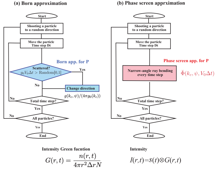
Figure 8. Flowchart of the Monte Carlo simulation code according to the RTT for the scalar wavelet intensity in uniform random media. (a) RTT with the Born approximation. (b) RTT with the phase screen approximation.
