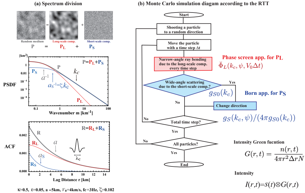
Figure 10. Spectrum division method. (a) Division of P into two components, P_S and P_L , with respect to the center wavenumber of a wavelet k_c as a reference, where \zeta is a tuning parameter. (b) Flow-chart of the Monte Carlo simulation according to the RTT with the spectrum division method. Modified from Sato and Emoto (2018).
