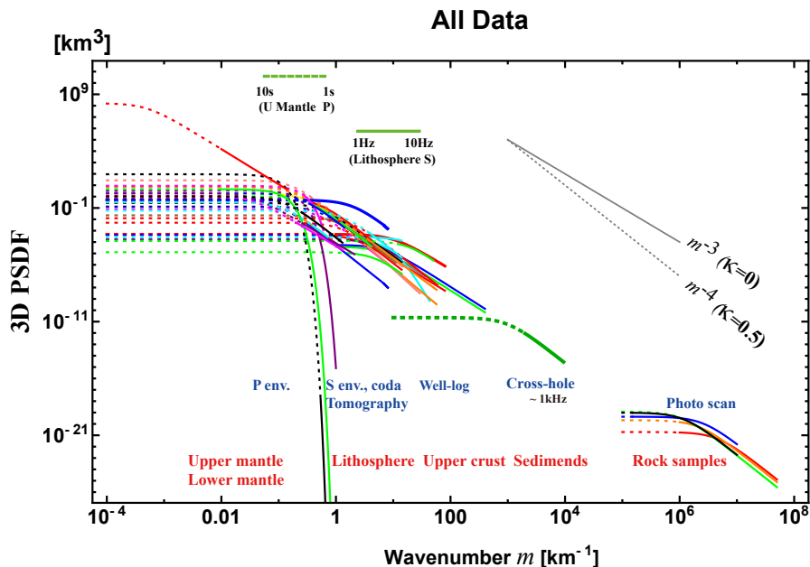
Figure 5. 3D PSDF vs. wavenumber for all the data.
