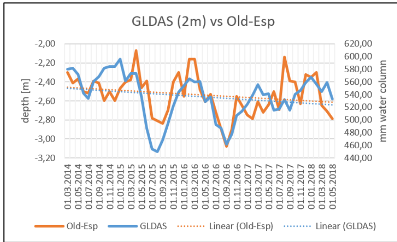
Fig. 1. Groundwater level recorded at Oldisleben-Espersstedt and compared to soil water content from GLDAS, monthly samples.
