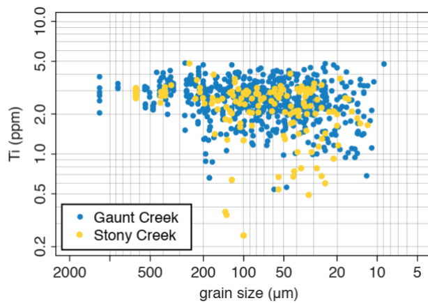
Figure 6. Plot of Ti concentration vs. grain size for all data. Grains >\sim 250\ \mu\text{m} have a relatively homogeneous Ti concentration \sim 2\text{--}4\ \text{ppm} which we interpret to predate Alpine Fault deformation. Smaller grains ( <200\ \mu\text{m} ) were at least partly formed by dynamic recrystallization during late stages of deformation, exhumation, and cooling. Despite very large strains ( \gamma = 12\text{--}120 ) at high temperature, less than half of the small recrystallized grains have Ti concentrations significantly lower than relict values of 2\text{--}4\ \text{ppm} . We interpret that most deformation was associated with pressure-temperature conditions where Ti concentrations of 2\text{--}4\ \text{ppm} were stable, specifically that mylonite and protomylonite deformation occurred along a cooling path that followed a constant-Ti isopleth (see text for details). Stony Creek analyses include data from Cross et al (2015).
