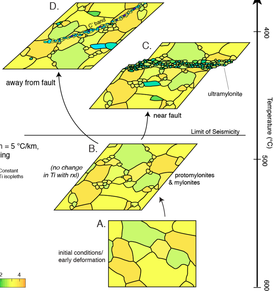
Figure 12. Simplified illustration of interpreted microstructural and Ti-in-quartz evolution. “Phase 1” deformation begins with Ti-in-quartz concentrations at 2-4 ppm (A). Strain associated with protomylonite and mylonite formation (B) involves recrystallization with no change in Ti-in-quartz concentrations due to exhumation along a constant-Ti isopleth (e.g. Fig. 11). During “phase 2,” newly recrystallized quartz grains tend to have lower Ti concentrations as a result of cooling along a much steeper segment of the geothermal gradient (Fig. 11). Near the fault (C), ultramylonites form with Ti-in-quartz concentrations of 1-2 ppm. The latest quartz recrystallization occurs away from the fault in protomylonites and mylonites in C’ bands (D). Sporadic recrystallization of some medium-sized grains with Ti-in-quartz concentrations below 2 ppm occurs in some rocks during phase 2.
