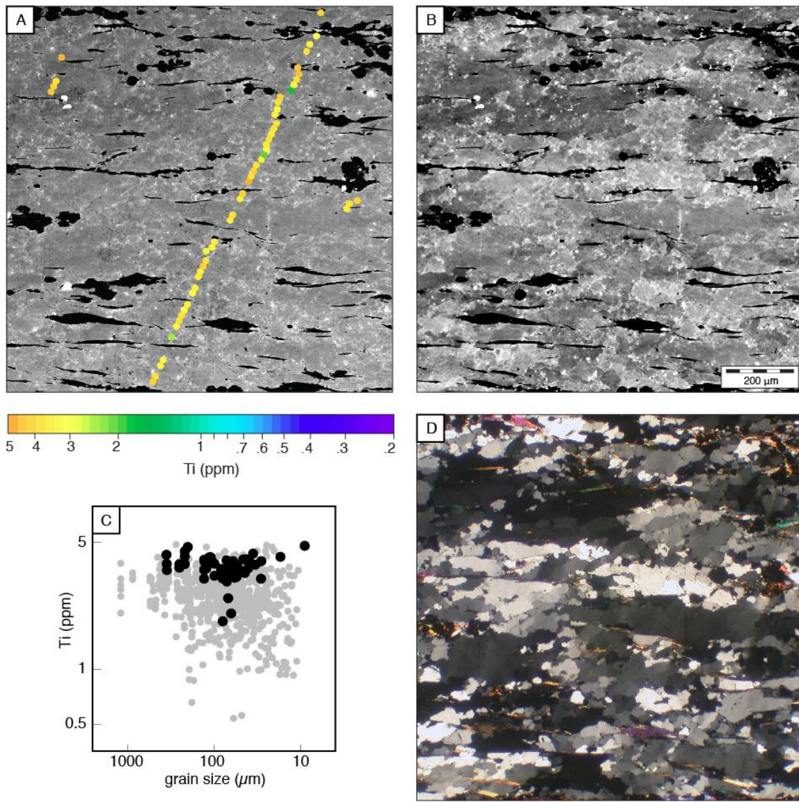
Figure 4. (A.) Panchromatic (200-960 nm) cathodoluminescence (CL) image of protomylonite metachert sample 77900 showing uniformity of Ti concentrations at analysis points. (B) 470 nm wavelength cathodoluminescence (CL) image. (C) Ti-in-quartz data for this sample (black) against a backdrop of data from other Gaunt Creek samples—no variation in Ti content with grain size is observed. (D) Cross-polarized photomicrograph of the same area. As typical of many samples, Ti-in-quartz contents vary between ~2 and 3 ppm, with no apparent spatial pattern. The blue spectrum peak (~470 nm, 2.65 eV) is dependent on quartz c-axis orientation, since dark grains in panel (B) are also dark in panel (D). The Ti peak at ~415 nm (Wark and Spear, 2005) was not detected in this sample, probably due to the low concentrations of Ti in the sample.
