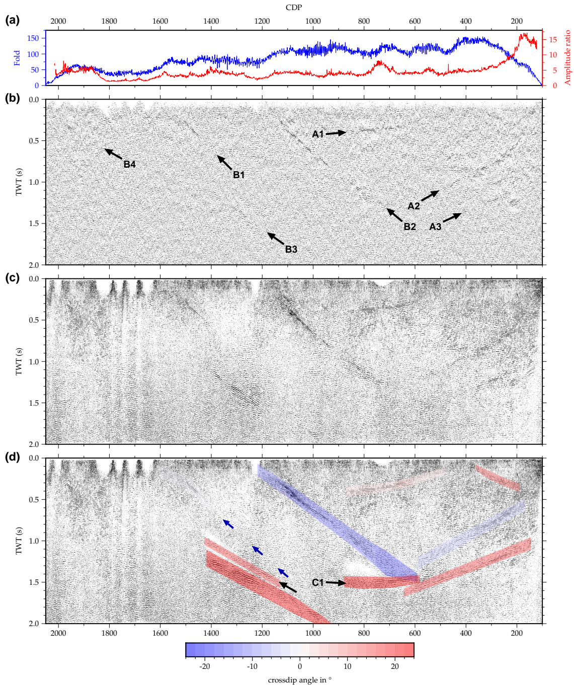
Figure 9. Comparison between the original processing of the Burträsk dataset and the reprocessing at different stages: (a) Fold distribution along the profile and mean amplitude ratio between the 200 ms of data and the background noise; (b) original stack; (c) reprocessed stack without crossdip correction; (d) reprocessed stack with crossdip correction overlain by the crossdip angles used in the correction. The small blue arrows indicate a possible continuation of reflection B1.
