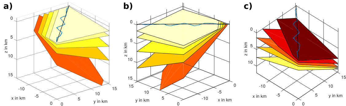
Figure 4. Reflector geometry used in the synthetic modeling. Model 1 (a) comprises reflectors with 5^\circ , 10^\circ , 20^\circ , 30^\circ and 45^\circ crossline dip from top to bottom. Model 2 (b) consists of a series of reflectors with 5^\circ , 10^\circ , 20^\circ , 30^\circ and 45^\circ inline dip. Model 3 (c) features reflectors with inline dips of 8.5^\circ , 16.1^\circ , 22.2^\circ , 26.6^\circ and 29.1^\circ and crossline dips of 29.1^\circ , 26.6^\circ , 22.2^\circ , 16.1^\circ and 8.5^\circ . The blue line represents the acquisition line and the black line the CDP line of the Burträsk dataset.
