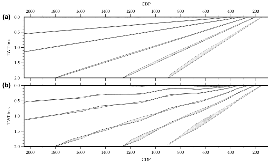
Figure 6. Results of the second synthetic model with reflectors dipping in the inline direction. The top panel (a) shows a stack without crossdip correction that exhibits the normal smearing due to inline dip. The bottom panel (b) shows a stack with a constant crossdip correction of -10^\circ applied. The reflections get clearly distorted due to the falsely applied crossdip correction. In most areas, smearing is increased but locally, reflections focus slightly.
