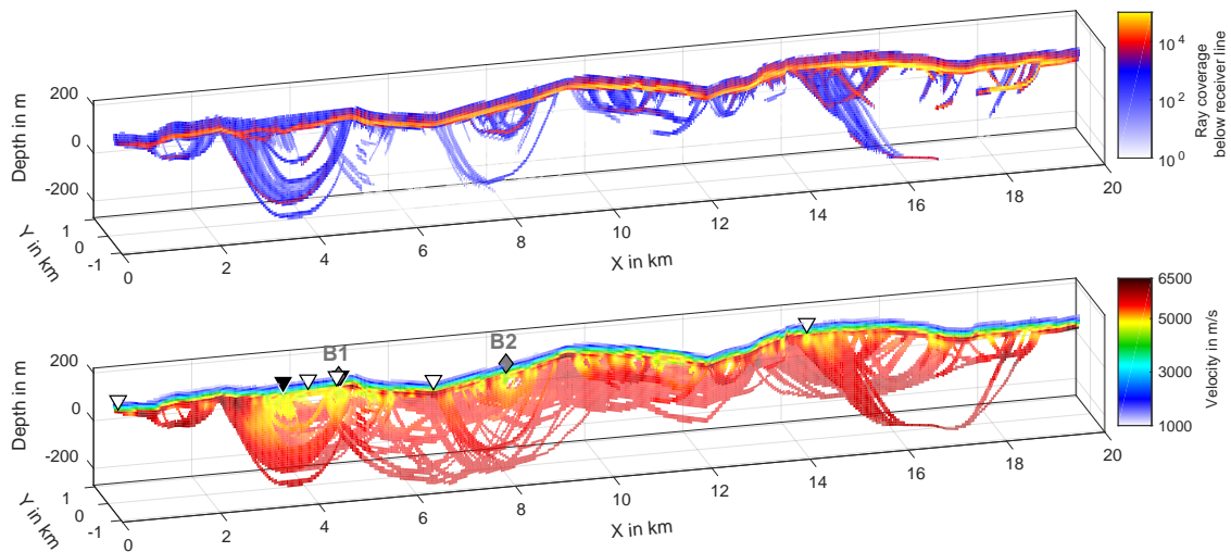
Figure 11. 2D slice of the ray coverage and the velocity model from the first break tomography. The upper panel shows the ray coverage in a 100 m wide zone below the receiver line. The lower panel displays the velocity below the receiver line in bright colors. In areas without velocity information below the receiver line, the average of the velocity model in the y direction is plotted in dim colors. The black triangles mark the location of the fault scarp, the white triangles indicate deformation zones and the grey diamonds correspond to the surface projection of reflections B1 and B2. The vertical exaggeration of the model section is 5.
