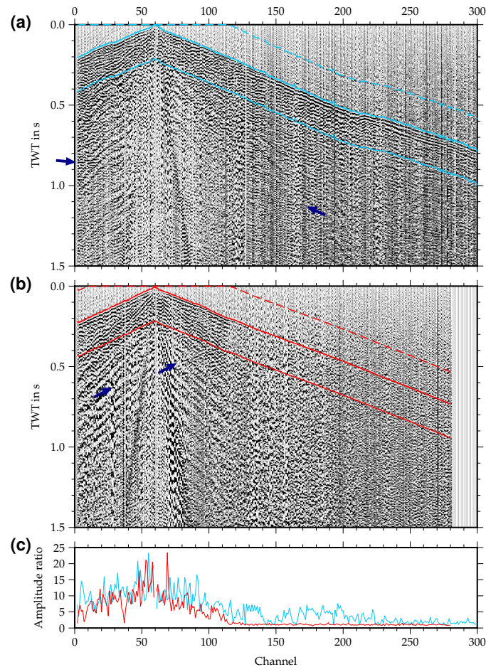
Figure 8. Unprocessed shot gathers illustrating variations in the background noise level. The upper shotgather (a) displays very clear first arrivals along the whole spread whereas the lower shotgather (b) is dominated by noise for larger offsets. The light blue and red lines mark the windows used for estimating the amplitude ratio between background noise and first arrival (c). The dark blue arrows indicate reflections.
