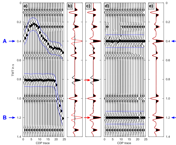
Figure 3. Synthetic CDP gather illustrating the principle of the crossdip correction. Panel (a) shows a NMO corrected CDP gather including two reflections with 10^\circ crossdip. The cross-offset distribution corresponds to the cross-offset distribution of CDPs 350 and 1350 of the Burträsk data. The comparison of the uncorrected stack (wiggles) with the theoretical stack (red line) in panel (b) indicates that reflection A is missing and reflection B is shifted. In the slant stack (c), reflection A is correctly imaged but reflection B appears twice in the trace. After crossdip correction, the energy is aligned at the correct time in the CDP gather (d) and in the corrected stack (e), both reflections are correctly imaged.
