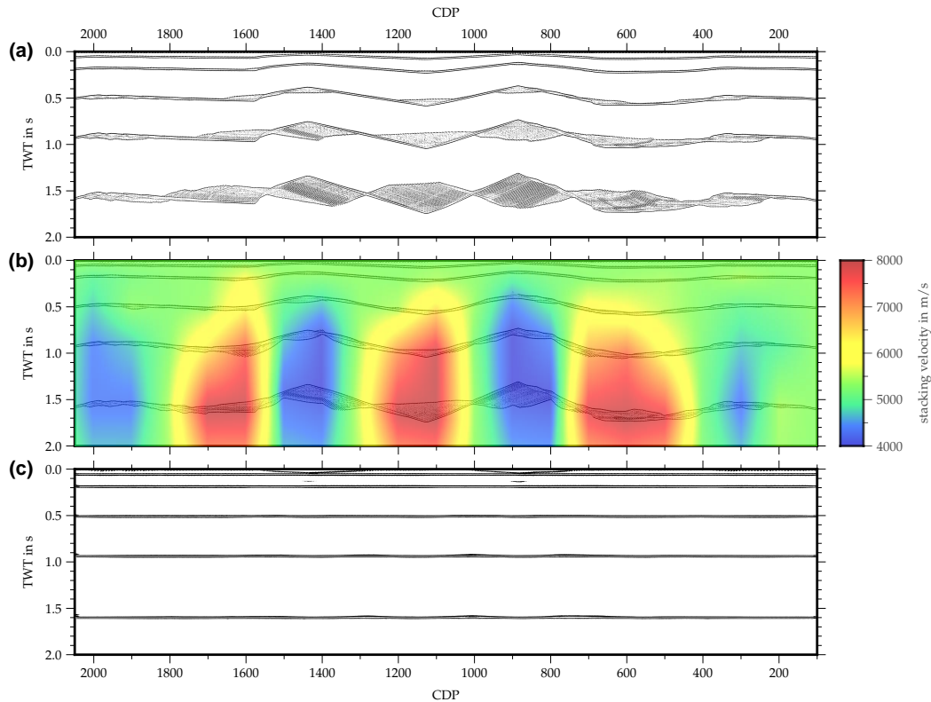
Figure 5. Results of the first synthetic model with reflectors dipping in the crossline direction. The reflections in the stacked section without crossdip correction (a) are heavily deformed and smeared. Using the optimum stacking velocities instead of the model velocity (b) reduces the smearing locally, but the reflections remain distorted. After crossdip correction, the reflections become focused and flattened (c).
