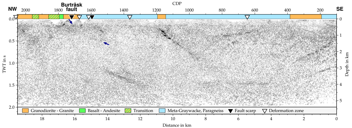
Figure 10. Migrated section along the Buträsk profile. For comparison, the surface geology is plotted on top of the section and the location of the fault scarp and deformation zones are marked. The small blue arrows highlight a very weak reflection that might be associated to the fault scarp. The vertical exaggeration of the section is approximately 1.
