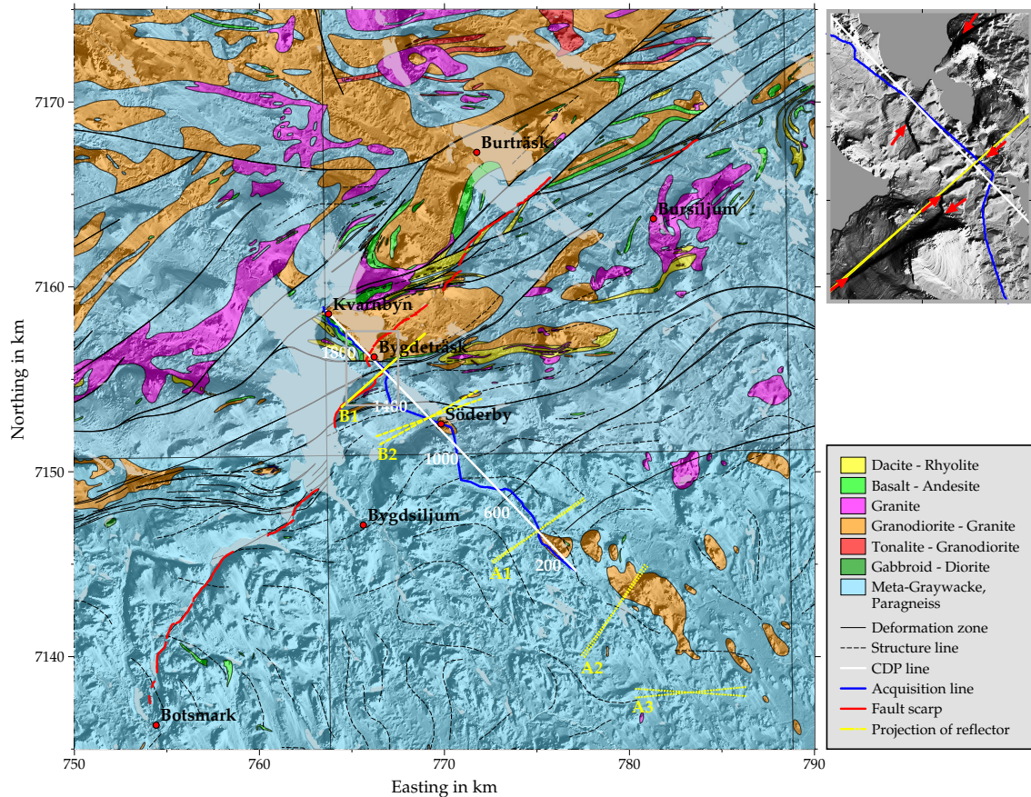
Figure 2. Geological map of the survey area and location of the Burträsk profile. The yellow lines mark the surface projection of reflector planes corresponding to the most prominent reflections in the seismic data with solid lines used for well constrained surface locations and dotted lines for poorly constrained locations. Note that the actual reflection points are shifted laterally for reflectors with a large crossdip component. The map inset shows an enlargement of the fault scarp and the red arrows indicate the location of the fault scarp. The location of the map is indicated in Fig. 1. Geological map ©Geological Survey of Sweden; elevation data ©Lantmäteriet.
