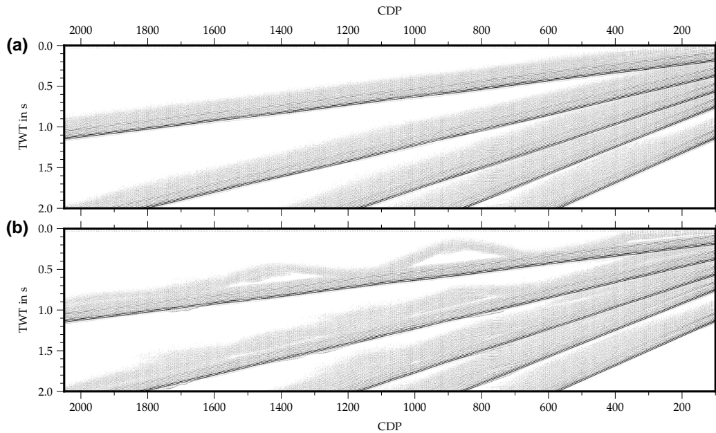
Figure 7. Results of the third synthetic model with reflectors dipping in the inline and crossline direction. Comparison of the stacked section with crossdip correction before DMO correction (a) and with crossdip correction applied after DMO correction (b). In both cases, the reflections become focused and flattened but in the second case, artifacts are stronger.
