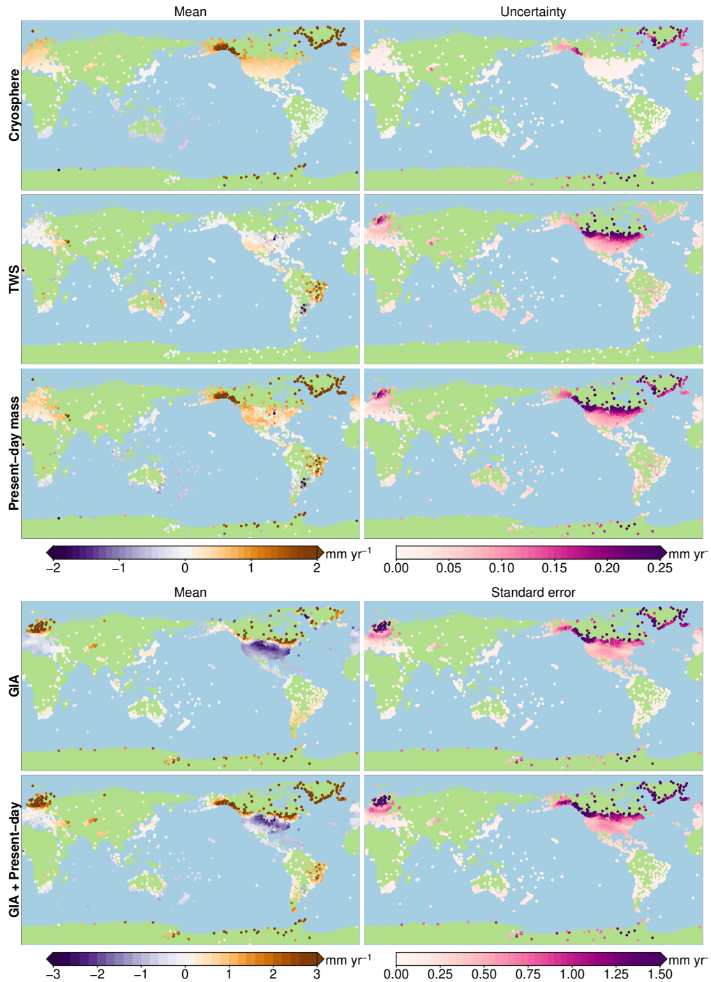
Figure 9. The modelled linear trends due to deformation computed over the time span of the individual GNSS record. The left panels show the mean trend, and the right panels the uncertainty from the large ensemble. Note that the color scales for the top three rows differs from the color scale of the bottom two rows.
