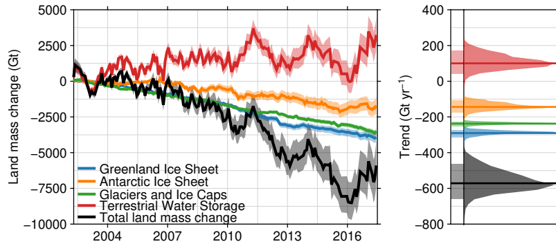
Figure 5. Total land mass changes as observed by GRACE, corrected for GIA. The left panel shows the expectation (thick line) and 90% confidence intervals (shade) of the mass change time series for each process and the total land mass change. Negative values denote land mass loss. The right panel shows the expected value (thick line), 90% confidence interval (left shade) and PDF (right shade) of the resulting linear trend.
