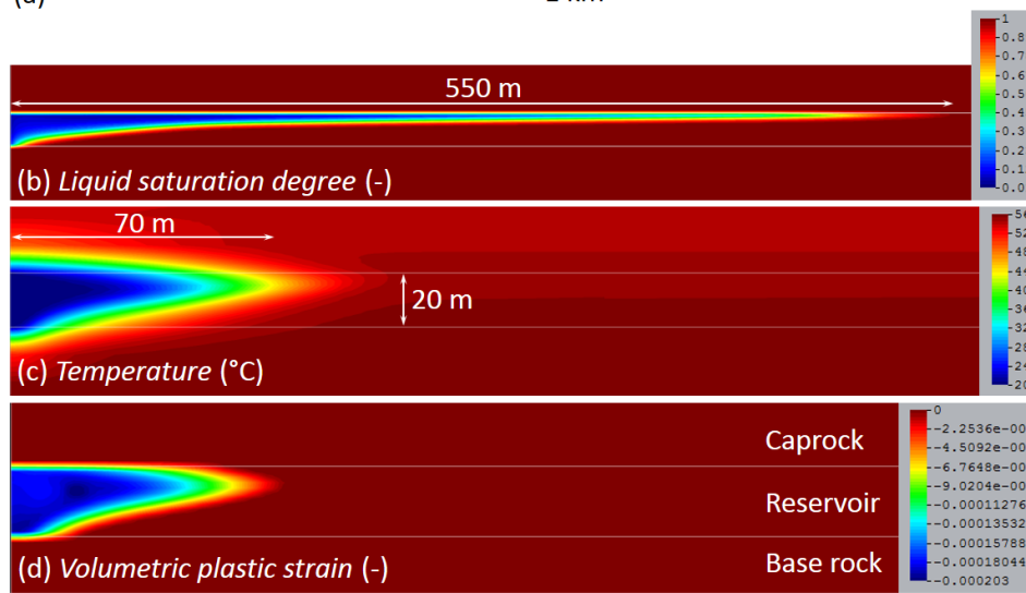
Figure 5: (a) Model setup, (b) Liquid saturation degree, (c) temperature distribution and (d) volumetric plastic strain after 2 years of injecting 0.2 \text{ Mt/yr} of \text{CO}_2 at 20 \text{ °C} through a vertical well. While (c) and (d) are plotted at the same scale, (b) is plotted at a smaller scale.
