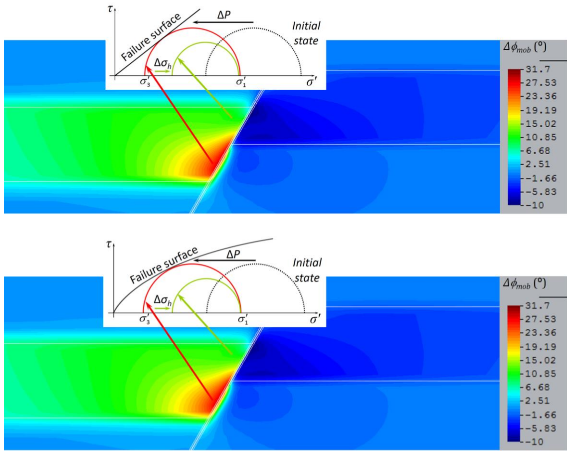
Figure 8: Distribution of stability changes induced by the pressure and stress changes shown in Figure 7, measured in terms of the mobilized friction angle changes , \Delta\phi_{mob} . The inset shows the Mohr circles before and after reservoir pressurization.
