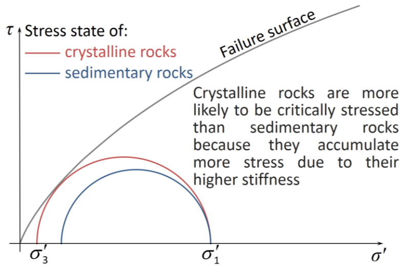
Figure 3: Schematic representation of the stress state of crystalline and sedimentary rocks, showing that sedimentary rocks, which are the rocks where CO 2 will be stored, are usually not critically generally less stressed than the crystalline basement .
