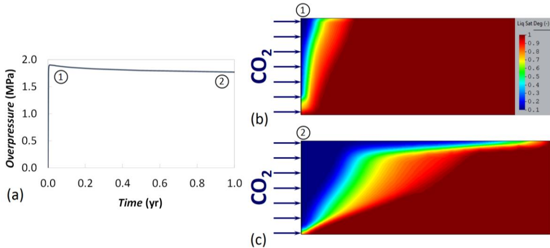
Figure 4: (a) CO 2 pressure evolution when injecting 1 Mt/yr of CO 2 through a vertical well in a 100-m thick aquifer with an intrinsic permeability of 10^{-13} m 2 and a radius of 100 km, (b) the CO 2 plume shape at the beginning of injection, coinciding with the peak in injection pressure (see number 1 in (a)), and (c) the CO 2 plume once gravity override dominates and the capillary fringe has been developed, leading to a slight pressure drop (see number 2 in (a)). The color bar displaying the liquid saturation degree in (b) applies for both (b) and (c).
