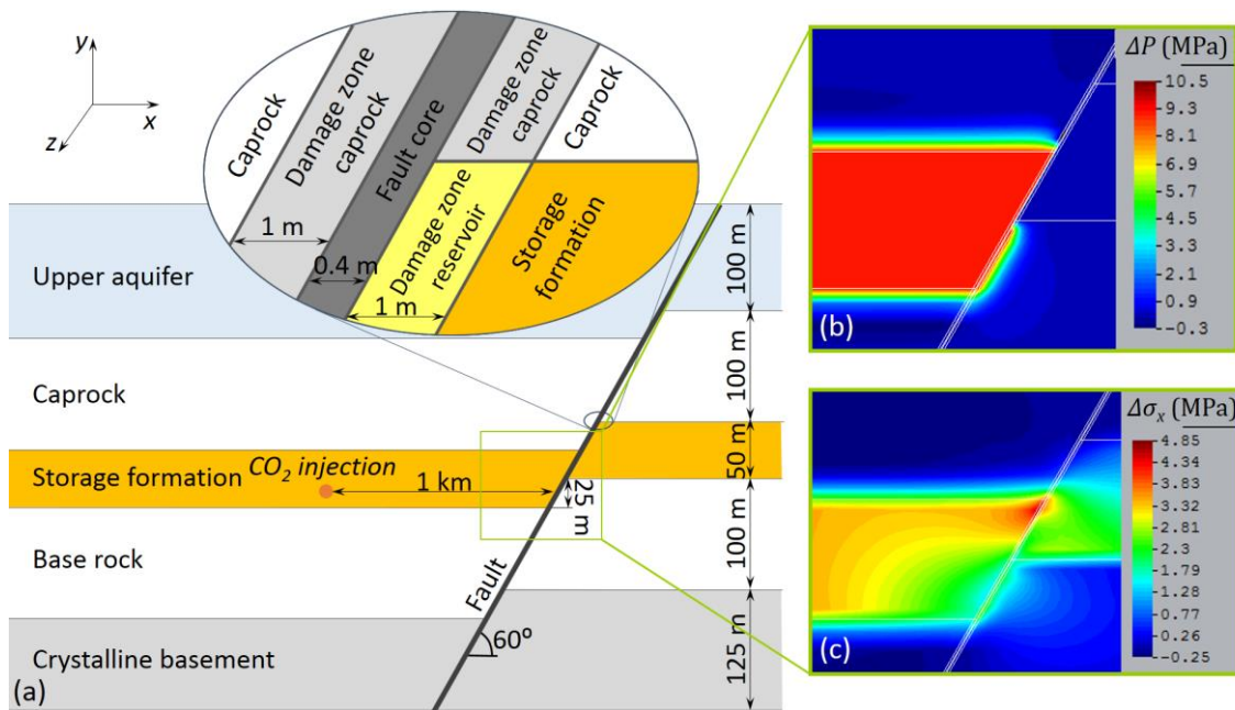
Figure 7: (a) Geological setting in a normal faulting stress regime (plane strain model), including a low permeability fault that leads to (b) reservoir pressurization, \Delta P , and (c) horizontal total stress changes in the in-plane direction, \Delta\sigma_x , when CO 2 is injected in the
