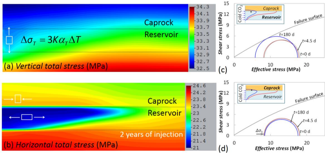
Figure 6: Total stresses in the (a) vertical and (b) horizontal direction after 2 years of injecting 0.2 Mt/yr of CO 2 at 20 °C through a vertical well, indicating the sign of the induced stresses. Thermal stresses, \Delta\sigma_T , are proportional to the bulk modulus, K , the thermal expansion coefficient, \alpha_T , and the temperature difference, \Delta T . The changes in the Mohr circles at a point placed 25 m away from the injection well in (c) the reservoir (2 m below the reservoir-caprock interface) and (d) the caprock (2 m above the reservoir-caprock interface) are also represented.
