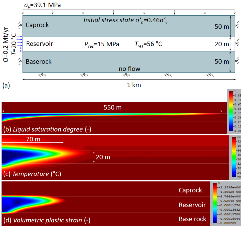
Figure 5: (a) Model setup, (b) liquid saturation degree, (c) temperature distribution and (d) volumetric plastic strain after 2 years of injecting 0.2 Mt/yr of \text{CO}_2 at 20 \text{ }^\circ\text{C} through a vertical well. While (c) and (d) are plotted at the same scale, (b) is plotted at a smaller
