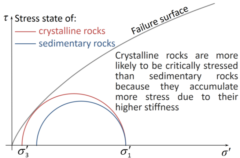
Figure 3: Schematic representation of the stress state of crystalline and sedimentary rocks, showing that sedimentary rocks, which are the rocks where CO 2 will be stored, are generally less stressed than the crystalline basement.
