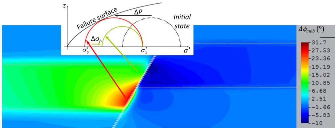
Figure 8: Distribution of stability changes induced by the pressure and stress changes shown in Figure 7, measured in terms of the mobilized friction angle changes, \Delta\phi_{mob} . The inset shows the Mohr circles before and after reservoir pressurization.
