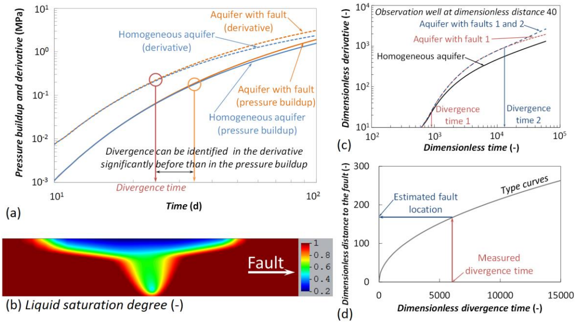
Figure 10: (a) Concept of the continuous characterization technique proposed by Vilarrasa et al. (2017c) to detect and locate low permeability faults using diagnostic plots; (b) asymmetric CO 2 plume as a result of the additional pressurization caused by a low-permeability fault, which displaces CO 2 towards the opposite direction of the fault; (c) detection of multiple faults by updating the conceptual model of the site and comparing field measurements with predictive simulations; and (d) estimation of the fault location from the measured divergence time in the derivative of the pressure evolution using type curves.
