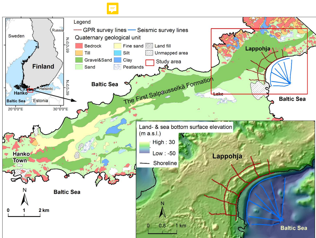
Figure 1: Quaternary geological map of the study area and location of survey lines in south Finland, northern Baltic Sea. Red lines indicate the GPR survey lines. Blue lines indicate the offshore seismic survey lines.
