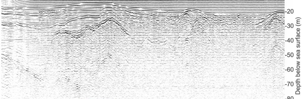
c: 250 - 1300 Hz reflection seismic
