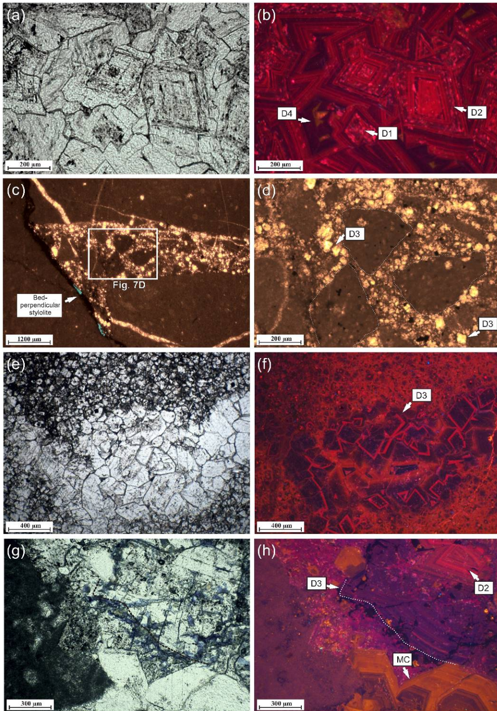
Figure 7: a, b) Photomicrographs of respectively, transmitted light and corresponding cathodoluminescence image showing the zoned rhombs of D2 with the remnants of D1 preserved in their cloudy core sampled from dolomitized Calcare Massiccio
