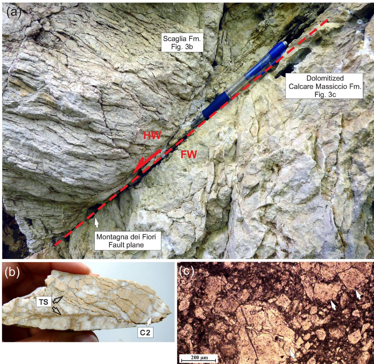
Figure 3: a) Field photograph showing the deformed Scaglia Formation in the hanging wall (HW) and brecciated, dolomitized Calcare Massiccio Formation in the footwall (FW) of the Montagna dei Fiori Fault. The red arrow indicates the sense of fault movement. b) A hand specimen from the deformed Scaglia formation showing abundant pressure solution seams (TS), indicated by arrows, cross-cutting calcite veins (C2). c) A transmitted light photomicrograph of the dolomitized, brecciated Calcare Massiccio Formation. Note all the breccia fragments are composed of dolomite (D4 here).
