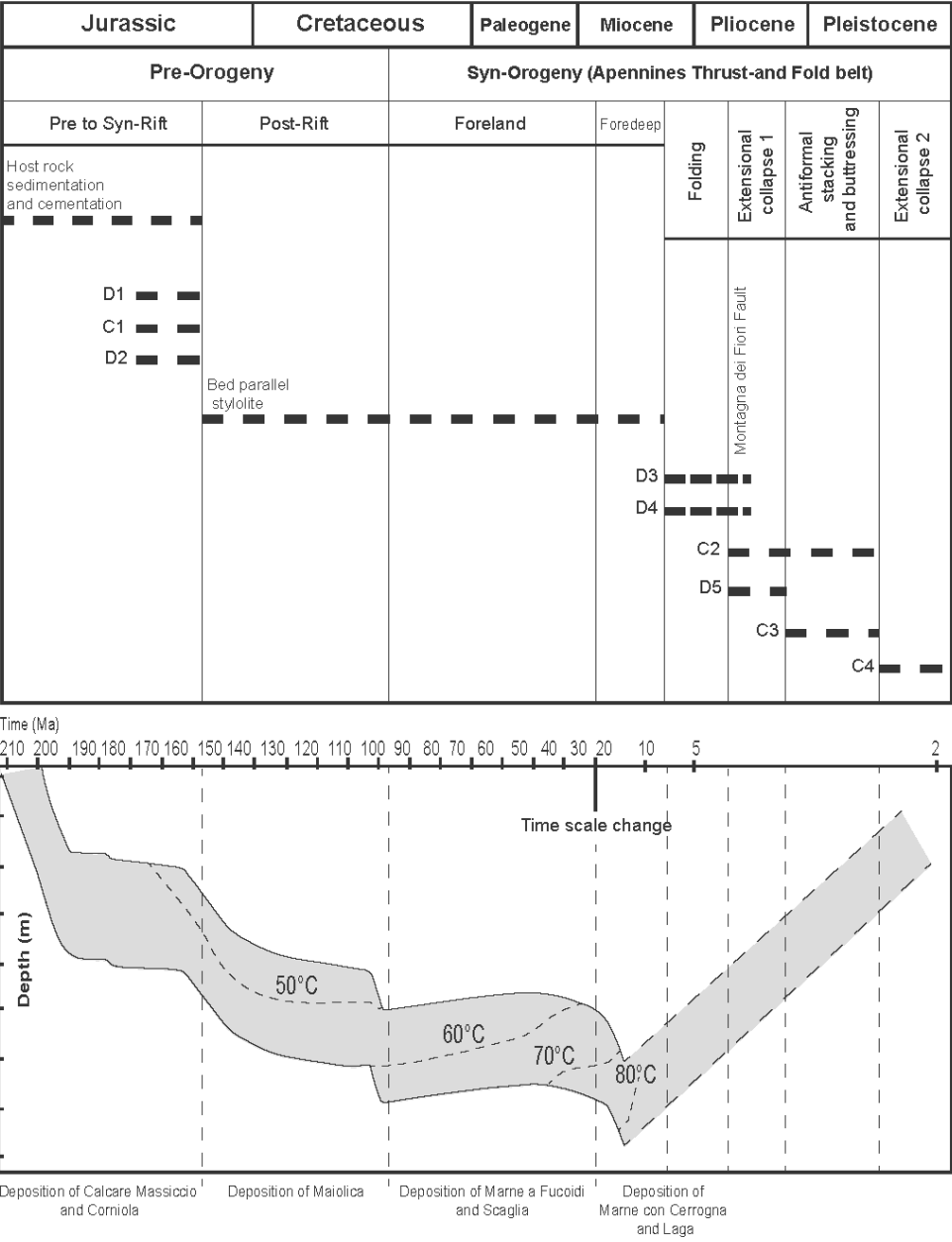
Figure 14: Generalized paragenesis of diagenetic phases in relation to deformational stages and burial history of the Calcare Massiccio Formation in the Montagna dei Fiori Anticline. The deformational stages are from Storti et al. (2018), and the burial curve is based on Ronchi et al. (2003). The burial curve was made based on paleo-depth, paleo-temperatures, sedimentation rate and paleo-heat flow.
