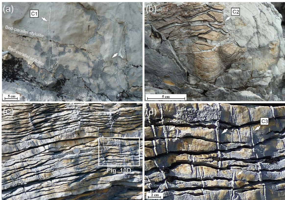
Figure 10: Field photographs showing the major calcite vein settings observed in Montagna dei Fiori: a) Cross-sectional view of bed normal Calcite vein 1 (C1) abutting bed-parallel stylolites in folded beds of the Calcare Massiccio Formation. b) Plan view of the Calcite vein 2 (C2) intensely affecting the deformed Scaglia (Rossa) Formation. c, d) Cross-sectional view of the Scaglia Formation, intensely affected by pressure solution seams of tectonic origin crossed-over by populations of bed-perpendicular Calcite veins (C3) in en echelon extensional arrays.
