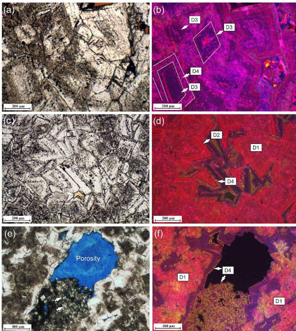
Figure 8: Photomicrographs of respectively, transmitted light and corresponding cathodoluminescence image of dolomite types: a, b) The cross-cutting relationship between D3 and D4 sampled from dolomitized Corniola Formation in Osso-caprino road. Note the presence of D3 within the core of dolomite crystals overgrown by D4. c, d) Successions of dolomite types sampled from dolomitized Calcare Massiccio Formation in field site f. Note the green CL color of D4 crystals. Typically, luminescent dolomites are known to show yellow, orange to red colors (Machel et al., 1991). Green luminescence in carbonates including dolomite have been attributed by a number of researchers to the incorporation of three valent rare earth elements (REE) such as Dy^{3+} and U^{3+} as luminescence activators within their crystal lattice (Luczaj and Goldstein, 2000). Another possibility is the emplacement of Mn^{2+} , with yellow luminescence, in Ca^{2+} sites with blue luminescence in the dolomite crystal lattice instead of preferential incorporation in the Mg^{2+} site (Sommer, 1972b; Amieux, 1982; Walker et al., 1989; Habermann et al., 1999). Accordingly, non-stoichiometric,
