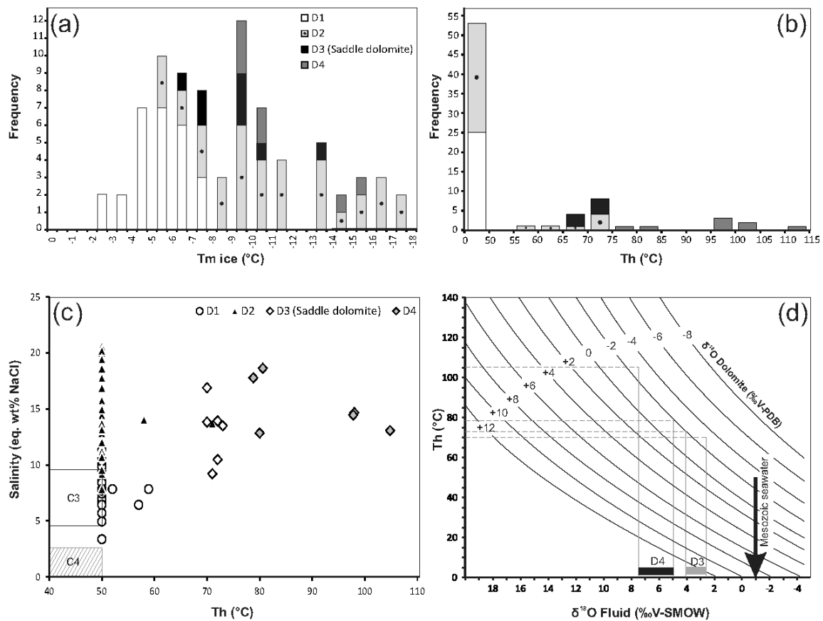
Figure 13: Overview of microthermometry analysis of primary inclusions in Montagna dei Fiori: a) Frequency distribution of the Tmice (°C) in dolomite types. b) Frequency distribution of the Th (°C) in dolomite types. c) Salinity (eq. wt. % NaCl) versus Th (°C) of dolomite and calcite phases. d) Isotopic fractionation diagram from Land (1983) used to determine the isotopic composition (‰ V-SMOW) of parental fluids in equilibrium with dolomites in Montagna dei Fiori.
