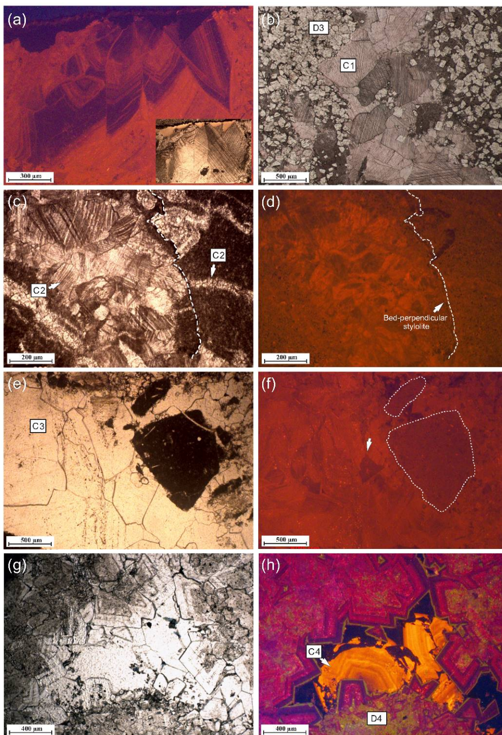
Figure 11: a) Cathodoluminescence and transmitted light (in set) image showing blocky to elongated crystals of C1 with zoned CL pattern in the Corano Quarry site. b) Transmitted light image showing intensely twinned C1 crystals overprinted by euhedral to
