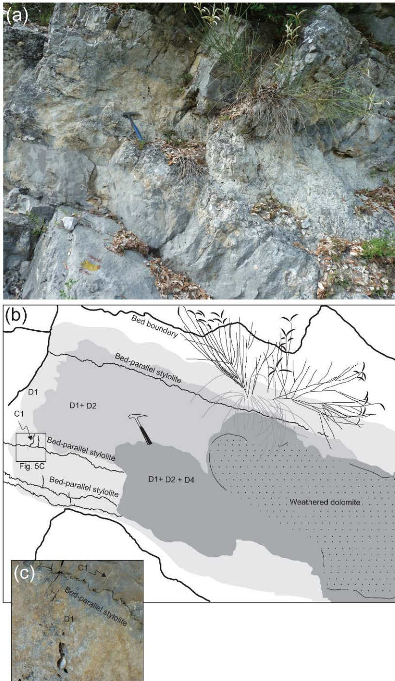
Figure 5: Field photograph (a) and a simplified sketch (b) in field site d showing a dolomitic pocket (grey color) and its relation with bed-parallel stylolites within the Calcare Massiccio Formation (hammer is 40 cm long). Note C1 is the only calcite cement here.
