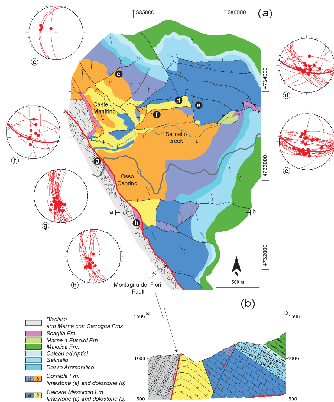
Figure 2: a, b) Geological map of the central sector of the Montagna dei Fiori Anticline, and cross-section oriented parallel (a-b) to the hinge line representing the tectono-stratigraphic architecture of the faulted anticline (modified after Storti et al., 2017a). The stereonets (Schmidt equal area projection lower hemisphere) provide the attitude of the extensional faults. The locations of the corresponding field sites are indicated by letters. c) At this location, well exposed N-S striking extensional fault zones offset the dolomitized Corniola Formation. The fault zone is characterized by near-horizontal stylolites localized in the footwall damage zone
