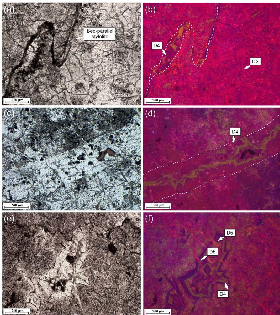
Figure 9: Photomicrographs showing respectively, transmitted light and corresponding cathodoluminescence image of D4 and D5 in relation to stylolites and fracturing: a, b) D4, exploiting a bed-parallel stylolite that crossed-cuts D1 and D2 sampled from dolomitized Calcare Massiccio Formation in field site d. c, d) A sub-horizontal fracture cemented by D4 sampled from dolomitized Corniola Formation in field site f. e, f) D5 microveins (arrows) intersecting all the predating dolomite types in the footwall brecciated zone of the Montagna dei Fiori Fault, sampled from dolomitized Calcare Massiccio Formation in Castel Manfrino site.
