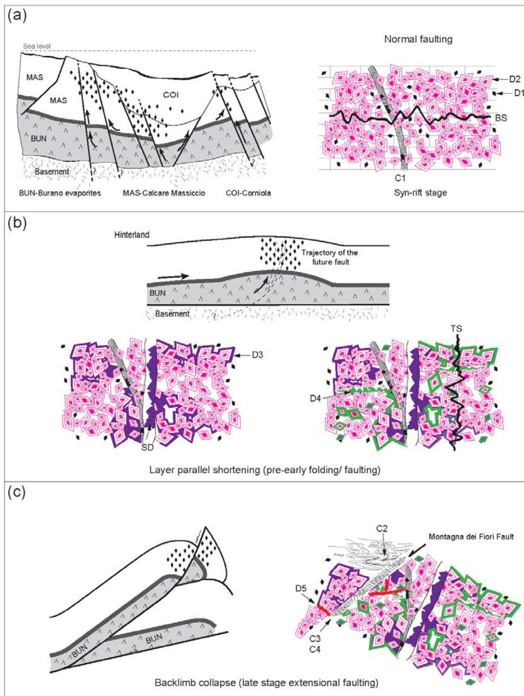
Figure 15: Sketch showing the successive fault-related diagenetic phases, of most importantly dolomitization, recorded in the carbonate succession exposed at the core of the Montagna dei Fiori Anticline (not scaled). Different diagenetic phases are indicated
