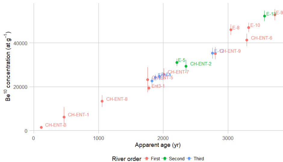
Figure 2: 10 Be concentrations in the Entle catchment against apparent age (yr).
