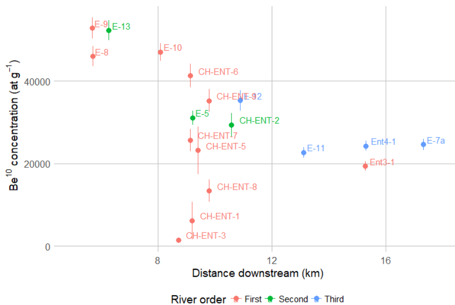
Figure 1: ^{10}\text{Be} concentrations in the Entle catchment against downstream distance.
