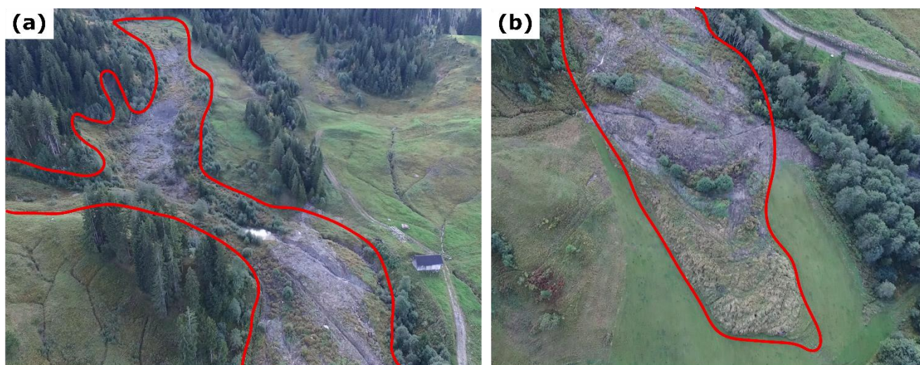
15 Figure 3: Illustration of the Schimbrig earthflow acting as a source of sediment in the river catchment. (a) Upper part with surface subsidence. (b) Toe of the earthflow with surface bulging. The location of the Schimbrig earthflow is depicted in Figure 2.
