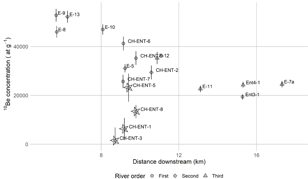
Figure 5: 10 Be concentrations (at g -1 ) along the river network of the Entle catchment. Downstream distance is computed from the river source to the outlet of the Entle catchment. Samples from the earthflow-affected Schimbrig catchment are marked with a star.
