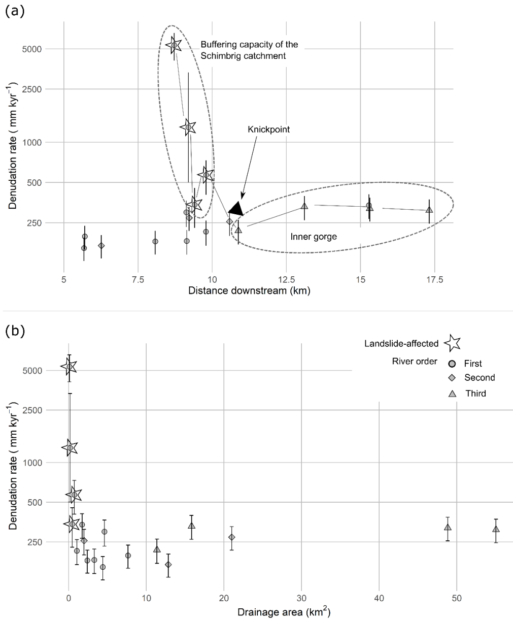
5 Figure 6: CRN-derived denudation rates ( \text{mm kyr}^{-1} ) in the Entle catchment against (a) downstream distance and (b) drainage area. Downstream distance is computed from the river source to the outlet of the Entle catchment. Samples from the earthflow-affected Schimbrig catchment are marked with a star . The grey line connects the points that are hydrologically connected, and part of the same fluvial system (Schimbrig, Rossloch, Kleine Entle and Grosse Entle rivers). Denudation rate values on the y-axis are shown on a logarithmic scale.
