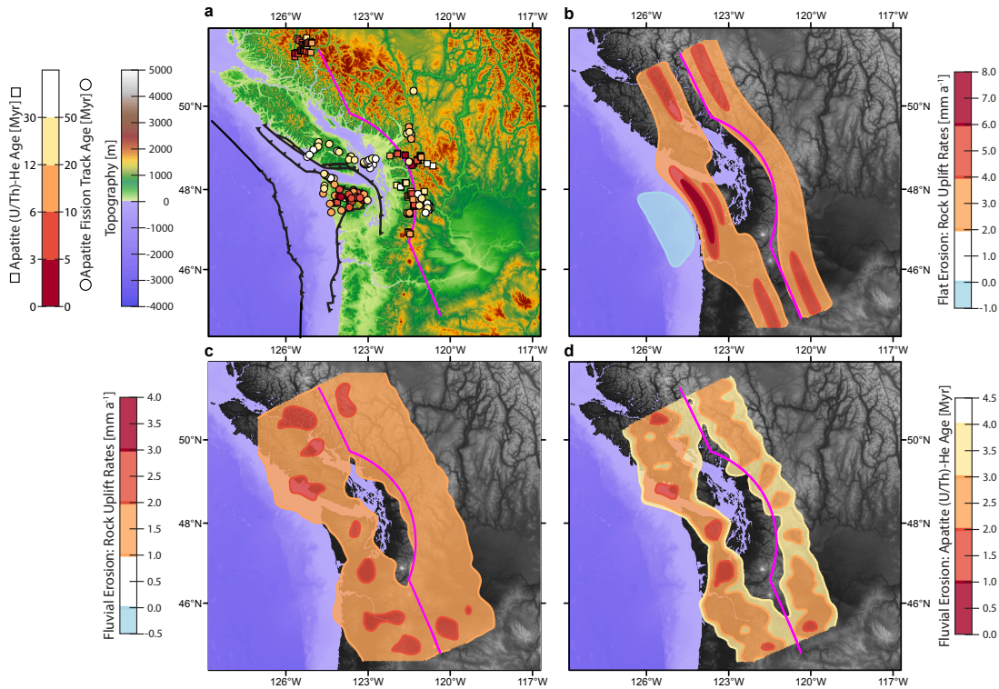
Figure 9. Comparison of Cascadia topography with model results: a Apatite (U/Th)-He (squares; Batt et al. (2001); Ehlers et al. (2006); Reiners et al. (2002, 2003); Simon-Labrie et al. (2014)) and Apatite Fission track cooling ages (circles, Brandon et al. (1998); England et al. (1997); Currie and Grist (1996); Reiners et al. (2002); Johnson et al. (1986)). Major structures from Brandon et al. (1998). b Flat erosion (model 5) rock uplift rates. c Fluvial erosion (model 11) rock uplift rates. and d Fluvial erosion (model 11) predicted Apatite (U/Th)-He cooling ages. Model S-line in magenta for orientation. The region of increased uplift above the indenter for the flat erosion model coincides with the location of the Olympic mountains. The fluvial erosion model shows smaller variations in rock uplift rates and cooling ages that are roughly the same size as the extent of young cooling ages in the Olympics.
