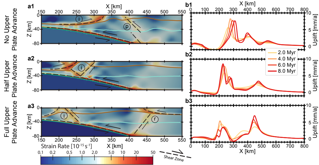
Figure 5. Temporal evolution of the no, half, and full upper plate advance indenter geometry models (4–6). a Strain rates on the y = 400 km cross-section at 8 Myr modeling time (cf. Fig. 4 showing same slices at 4 Myr). b Time slices of surface rock uplift rates along y = 400 km. No upper plate advance (model 3; top panels) scenario shows an indenter detachment in dynamic steady state, which slowly migrates to the right. In the half advance scenario (model 4; central panels), uplift above the indenter likewise saturates, but its position is stable and additional shear zones form in the last stage. Lastly, the full advance case (model 6; bottom panels) exhibits most uplift at the right uplift band, which continuously increases, whereas the indenter uplift ceases again after reaching a peak at 4 Myr simulation time.
