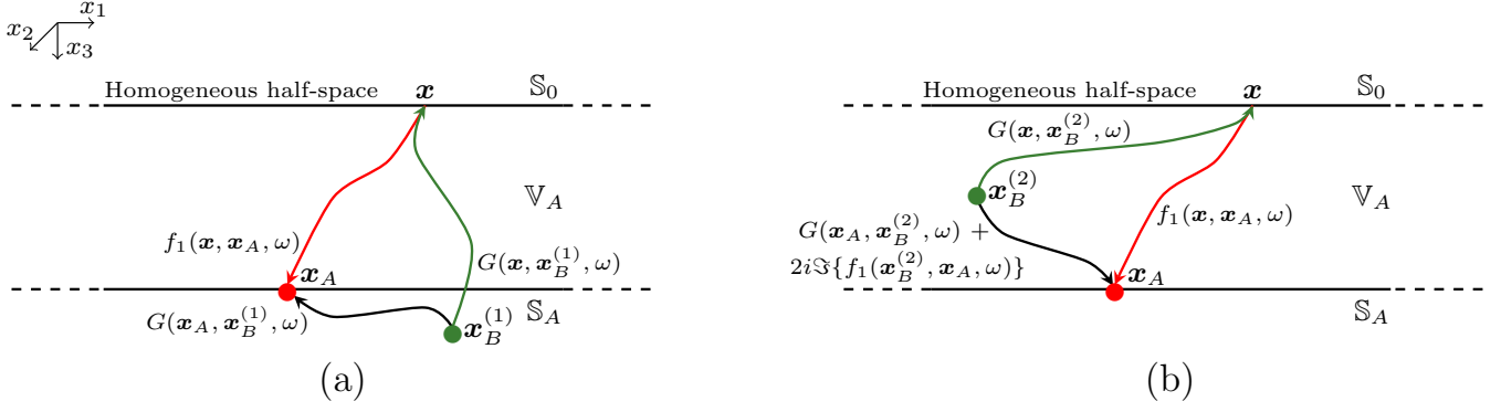
Figure 2. Setup for the single-sided Green's function representation for (a) a case where the source of the Green's function is located below the focal location and (b) a case where the source of the Green's function is located above the focal location. The rays in this figure indicate full Green's functions and focusing functions, including multiple scattering.
