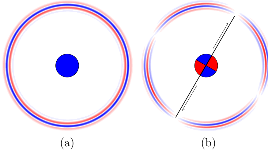
Figure 4. Comparison of the wavefields caused by (a) a monopole point source and (b) a double-couple point source tilted at an angle of 30 degrees. For both types of sources the radiation pattern of the source is shown in the center. The wavefields have been convolved with a 30 Hz Ricker wavelet.
