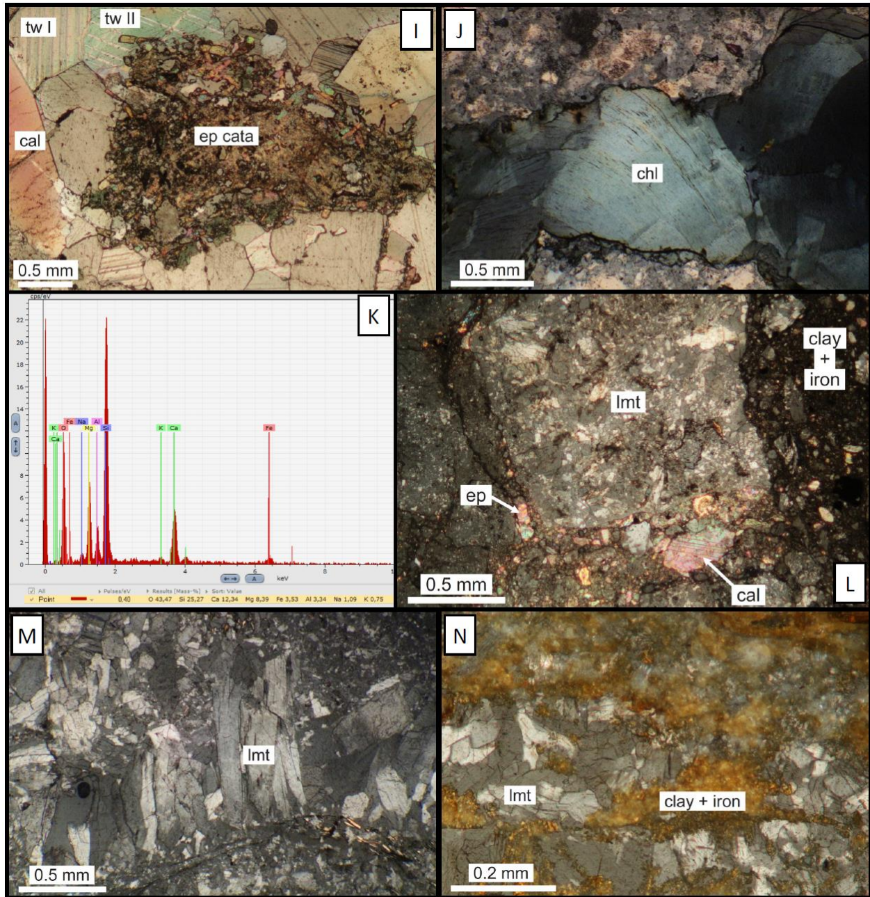
Figure 3: Microscope photographs of cataclasite and host-rock in NW Finnmark. (a) Precambrian S-C foliation made of muscovite (ms) microcrystals surrounding K-feldspar (Kfs) sigma-clasts; (b) Cataclasite vein (dashed green) in Precambrian basement rocks seemingly offset by iron- and clay-rich fractures that formed parallel to existing S-C foliation deformation planes (dotted pink). The amount of offset across iron-rich fractures is shown by a dextrally (red) offset, sheared quartz grain (yellow) and is lower than the apparent offset of the cataclastic vein in green; (c) Calcite-filled (cal) fracture in Precambrian basement rocks cross-cutting a vein of recrystallized quartz (qz) and a muscovite-bearing (ms) ductile microshear. Calcite cement crystals typically show type II (tw II; lower right inset) and type IV (tw IV; upper left inset) twinnings; (d) Preserved biotite (bt) foliation in Caledonian host rocks near a cataclastic (cata) brittle fault. Approaching the fault, biotite is increasingly recrystallized into chlorite (chl); (e) Highly fractured garnet crystal (grt) in Caledonian host rock cross-cut by epidote- (ep; type 1) and quartz-rich cataclasites (qz cata; type 2), which are both truncated by calcite-filled veins (cal; type 3). Both cataclasites and calcite veins are truncated by a third cataclasite made up with a matrix of angular, poorly sorted clasts of laumontite (lmt; type 4) cross-cut by late clay and iron-bearing veins (type 5); (f) Caledonian S-C foliation made of muscovite (ms) microcrystals surrounding K-feldspar (Kfs) sigma-clasts that have partly recrystallized into quartz (qz); (g) Cataclastic fault-rock showing the remains of preexisting S, C and C' foliation
