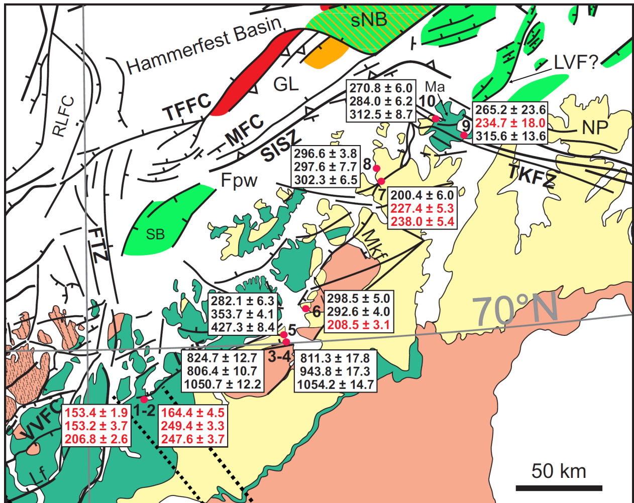
1480 Figure 4: Structural map of the study area showing the obtained K–Ar ages for each sample in Ma, including from top to bottom finest, intermediate and coarsest grainsize fraction ages. Ages in red are considered erroneous (see main text). Map modified after Indrevær et al., (2013) and Koehl et al. (2018). Legend and abbreviations as in Figure 1.
