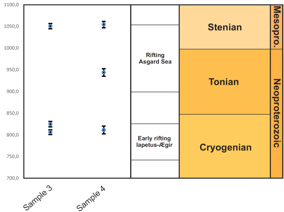
Figure 5: Graph displaying the obtained Precambrian ages for brittle faults in the Alta–Kvænangen tectonic window. The vertical axis is time in Ma and the horizontal axis shows the dated sample numbers, which locations are displayed in Figure 1 and Figure 4. Columns to the right show extensional tectonic events related to the formation of the NW Baltoscandian basins during the opening of the Asgard Sea (Siedlecka et al., 2004; Nystuen et al., 2008; Cawood et al., 2010; Cawood and Pisarevsky, 2017) and to the earliest phase of rifting of the Iapetus Ocean–Ægir Sea (Li et al., 1999, 2008; Torsvik and Rehnström, 2001; Hartz and Torsvik, 2002), and associated geological Periods and Eras.
