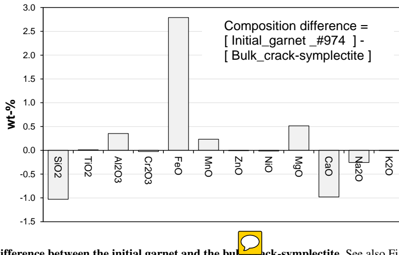
Figure 10. Composition difference between the initial garnet and the bulk crack-symplectite. See also Fig. 5e and Fig. 4d.
