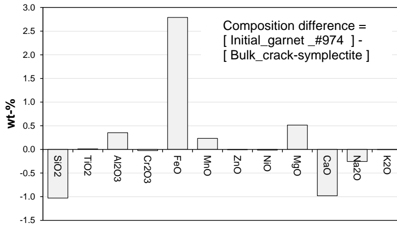
Figure 10. Composition difference between the initial garnet and the bulk crack-symplectite. See also Fig. 5e and Fig. 4d.
