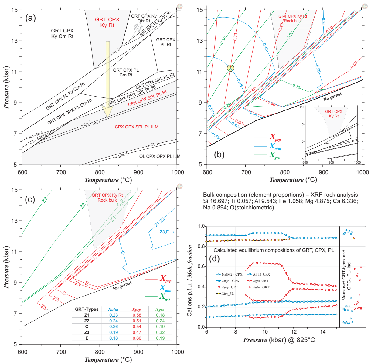
Figure 11. PT diagrams and comp osition of phases in sample UM8. (a) Equilibrium assemblage PT diagram (pseudosection) based on the rock bulk rock composition reproducing well the observed primary assemblage GRT+CPX+Ky+Rt and the later formed crack-symplectite assemblage CPX+OPX+ SPL+PL+ILM. The arrow denotes schematically the transition by isothermal decompression from the former to the latter assemblage. (b) Isopleths of the modeled ternary garnet equilibrium composition. The shaded area corresponds to the stability field of the primary assemblage. The yellow circle emphasizes the necessity of a common intersection point of the isopleths in case of a preserved equilibrium composition. The inlayed PT diagram is an extension of figure (a) up to 20 kbar. (c) Implied isopleths of the measured GRT-types and their proximity to the stability field of the primary assemblage denoted by the shaded area. The inlayed table summarizes the composition of the GRT-types. (d) Comparison of the measured GRT-types, clinopyroxene and plagioclase inclusions with their calculated equilibrium mineral compositions in the range 15–6 kbar at 825 °C.
