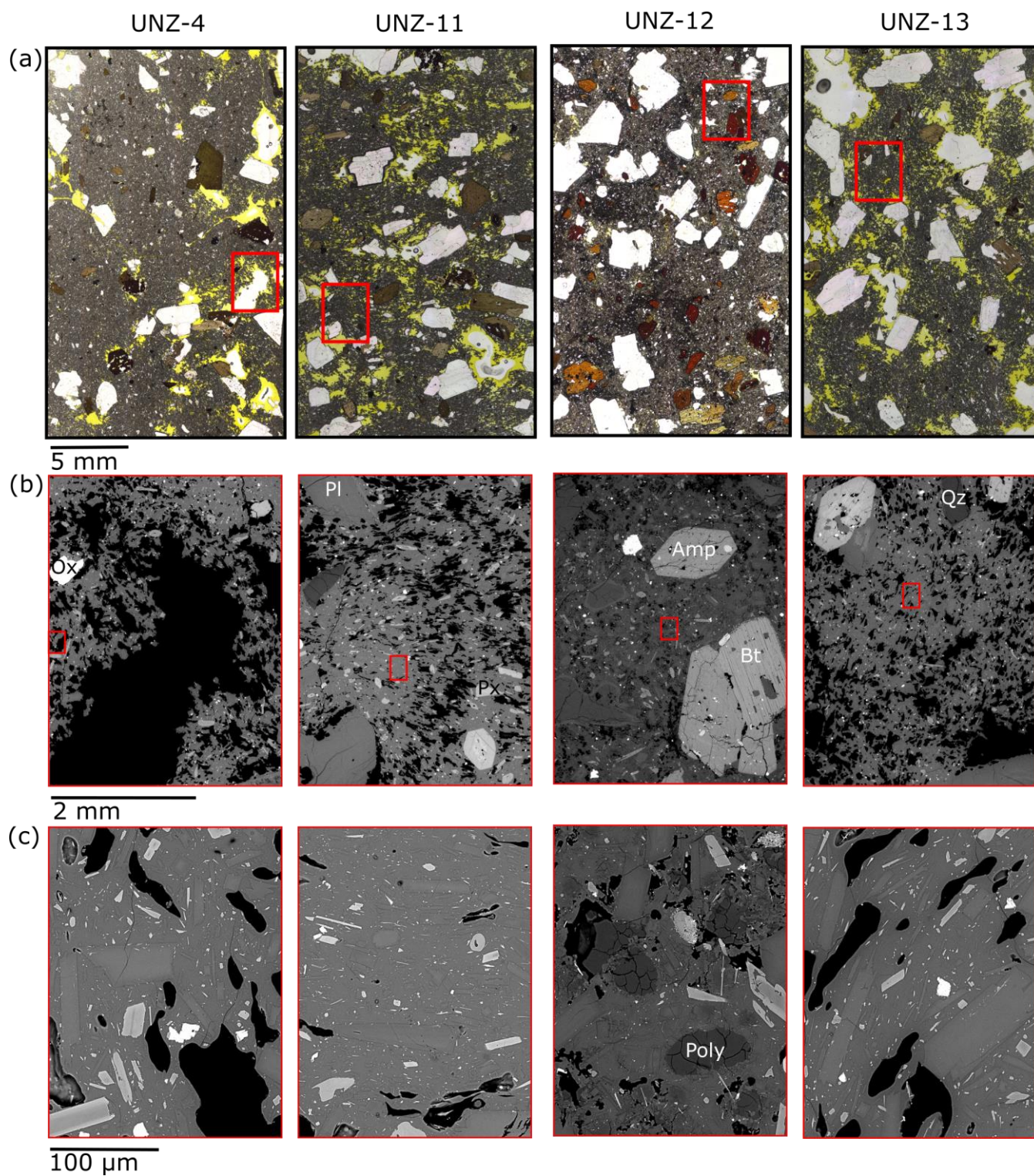
1075 Figure 3. Plane–polarised light (a) and backscattered electron images (b,c) of undeformed samples UNZ-4,-11, -12 and -13. (b) is a zoom into the red box in (a), and (c) is a zoom in of the red box in (b), displaying the groundmass textures. Amp: Amphibole, Bt: Biotite, Ox: Oxides, Pl: Plagioclase, Px: Pyroxene, Qz, Quartz, Poly: Silica polymorph. Images are orientated so that the later applied principal stress, \sigma_1 , is in the vertical direction. [Note the scale that is below each set of images.]
