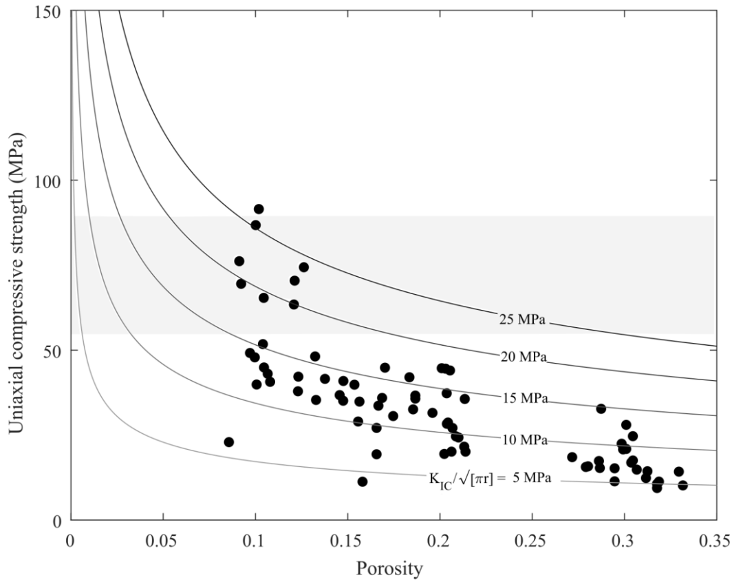
1130 Figure 11 Plot of uniaxial compressive stress against porosity showing the ambient temperature mechanical data (black dots), along- side contours of various values of \frac{K_{IC}}{\sqrt{\pi r}} (5–25 MPa) from the pore-emanating crack model (Eq. 2). The range of UCS given by the wing-crack model is also plotted as a shaded region. The mechanical data are cross-cut by the contours, suggesting a change in the dominant porous structure. At porosities > 0.25 the UCS given by the pore-emanating crack model with \frac{K_{IC}}{\sqrt{\pi r}} = 5\text{--}10 MPa seems to fit the data well. For porosities ranging from 0.12–0.2 the UCS given by the pore-emanating crack model with \frac{K_{IC}}{\sqrt{\pi r}} = 10\text{--}15 MPa encloses 1135 the data. The UCS for the densest rocks in the study (~0.08–0.12) would suggest yet a higher \frac{K_{IC}}{\sqrt{\pi r}} of 20–25 MPa. For porosities < 0.1 the UCS given by the wing-crack model is similar to the mechanical data ( \sigma = 54.2\text{--}89.7 MPa).
