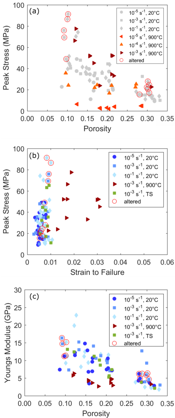
Figure 10. Strength and Young's Moduli of Unzen rocks and lavas at different conditions. Shades of blue represent tests carried out at ambient temperatures, shades of red indicate those performed at 900 °C, and green depicts thermally stressed samples which were tested in ambient conditions. The red rings circle the samples which were deemed visibly altered at collection. (a) Peak stress with porosity for all completed experiments. Low temperature tests, as seen in Figure 5 (a), are faded to grey. (b) Peak stress with strain at the point of sample failure (i.e. the strain at peak stress) for all experiments with a brittle response. (c) Young's modulus as a function of porosity for all samples that had a brittle response, calculated using the slope of the linear portion of the stress-strain curve (see Fig. S6).
