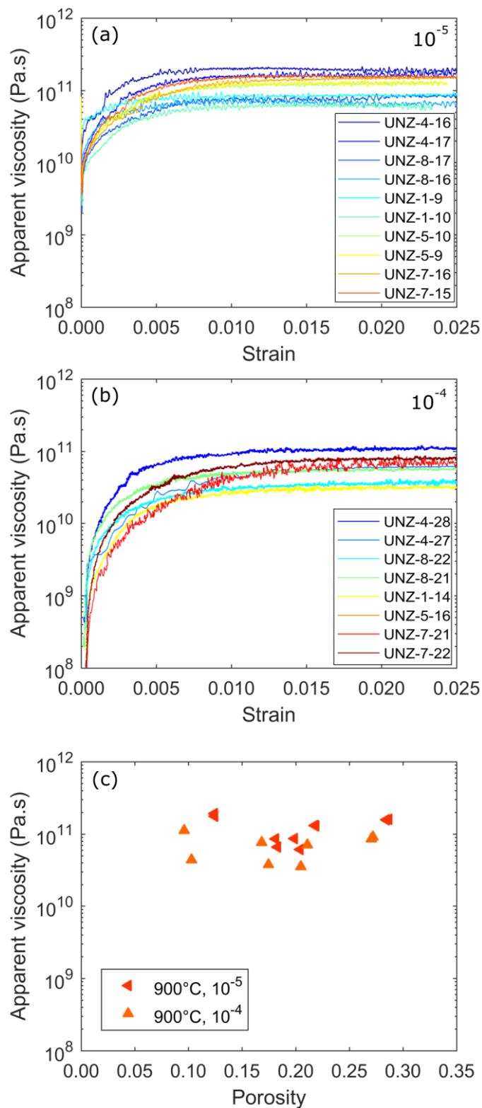
1115 Figure 9. Apparent viscosities of porous lavas at 900 °C for strain rates of (a) 10^{-5} \text{ s}^{-1} and (b) 10^{-4} \text{ s}^{-1} ; colours warm from blue to red with increasing sample porosity. (c) Compilation of apparent viscosities as a function of porosity for samples tested at strain rates of 10^{-4} \text{ s}^{-1} and 10^{-5} \text{ s}^{-1} . Viscosities decrease between strain rates of 10^{-5} to 10^{-4} \text{ s}^{-1} , an example of shear thinning in the Unzen samples. Porosity has no control on the apparent viscosities of the samples tested here.
