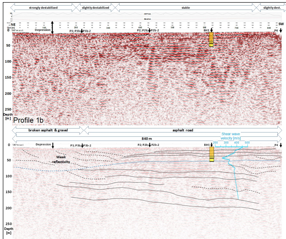
Figure 7: Resulting depth section of profile 1b after post stack FD time migration (top) and interpretation
