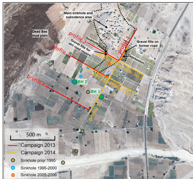
260 Figure 4: Map of the shear wave reflection seismic profiles acquired in 2013 (red lines) and 2014 (yellow lines). Green circles denote the locations of the boreholes made in 1994 (according to report of El-Isa et al. (1995)). Older refilled sinkholes are denoted by brown circles (after El-Isa et al. (1995)), blue circles (after Sawarieh et al. (2000)), and orange circle (after Bodet et al. (2010)). The dotted black polygon marks the updated outline of the main sinkhole and subsidence area after Al-Halbouni et al. (2017).
