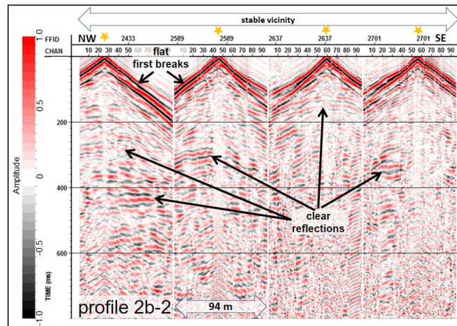
305 Figure 6: Examples of recorded shot gathers (AGC of 220 ms window, amplitude scaling and bandpass filter (18-20-78-82 Hz) applied) in time domain along profile 2b-2 (labelling as in Fig. 5). Good signal quality of first breaks and reflections mirrors a rather unaffected signal propagation in the subsurface, which correlates to the sinkhole-unaffected vicinity at surface. Reflection signals up to 400 ms in time represent layer responses from 70 m depth (applying 350 \text{ ms}^{-1} shear wave propagation velocity).
