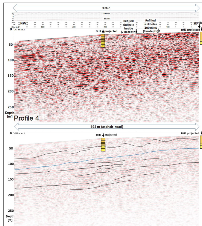
425 Figure 10: Depth section of profile 4 after post stack FD time migration (top) and interpretation of the main structure elements (bottom). For annotations see Fig. 7 . Lithology of boreholes BH1 and BH2 is projected from 200 m distance perpendicular into the profile. In contrast to profile 2, more gently NW- dipping events are present to 150 m depth, indicating less transportation energy of the alluvial material or an apparent structure dip. The top of the “silt and clay” layer in BH1 and BH2 is interpreted by the blue 430 line. Bowl shaped signatures close to the surface in the SE indicate sinkhole-caused subsidence and/or refilled channel side-cuts. Significant reflection amplitudes of a stronger reflector pattern close to the NW end at nearly 90 m depth may indicate an evaporite-rich lense included in the alluvium-lacustrine deposits.
