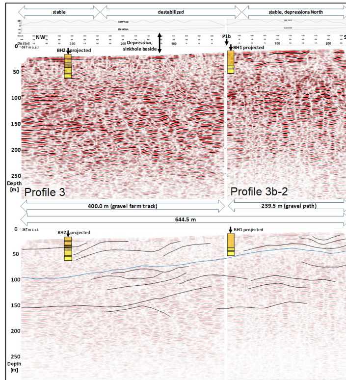
400 Figure 9: Combined depth sections of profiles 3 and 3b-2 after post stack FD time migration (top) and interpretation of the main structure elements (bottom). For annotations see Fig. 7 . Lithology of boreholes BH1 and BH2 are projected from 400 m distance perpendicular into the profile, therefore probably not showing the precise layer signature. The interpreted top of the “silt and clay” layer in BH1 and BH2 is shown by the blue line. The centre part of the profiling track was repeatedly affected by recent sinkhole activity directly beside in the NE. For farming access it was refilled with gravel along more than 250 m, which was subsequently again affected by sinkholes and subsidence. This may cause the weaker reflection signatures in the upper 50 m if compared to profile 2 ( Fig. 8 ). The main reflection pattern signature is similar to profile 2 and 2b-2, showing NW dipping events. In the SE of the profile a V-shaped structure is visible close to surface, filled with nearly horizontal reflection events, which is interpreted as a refilled channel side-cut. Due to the wide subsidence area NE of profile 3 the top of the “silt and clay” layer (blue line) was continued to NW starting from profile 1b instead using the projection of BH2. 405 410
