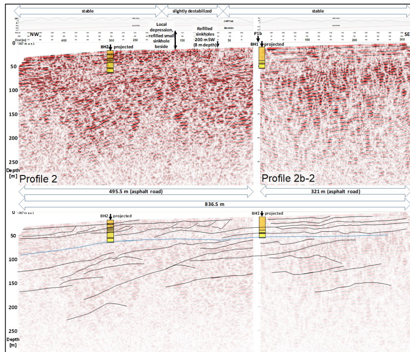
385 Figure 8: Resulting depth sections of combined profiles 2 and 2b-2 after post-stack FD time migration (top) and interpretation of the main structure elements (bottom). For annotations see Fig. 7. Lithology of boreholes BH1 and BH2 is projected perpendicular into the profile from 200 m distance, and therefore may not show the precise layering signature. Except the top 40 m the main characteristics down to 200 m show stacked sequences of NW-dipping reflectors, which are interpreted as NW-prograding alluvial fan sequences. The interpreted top of the “silt and clay” layer in BH1 and BH2 is shown by the blue line.
