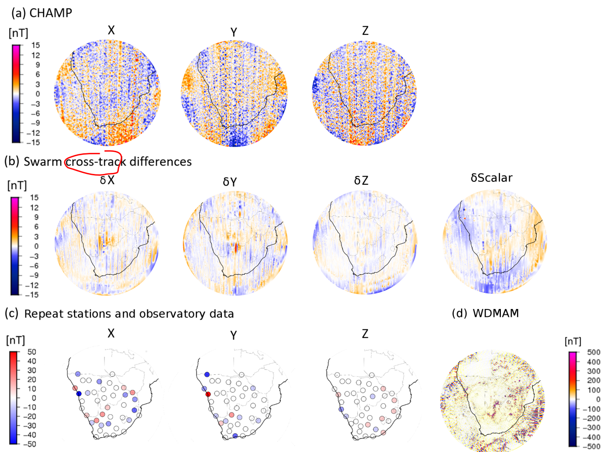
Figure 2. Residuals between our model and the input data for (a) the CHAMP vector measurements, (b) the Swarm cross-track differences of the vector and scalar measurements, (c) the repeat stations and observatory vector measurements and (d) the WDMAM grid points. Note the different colorscales.
