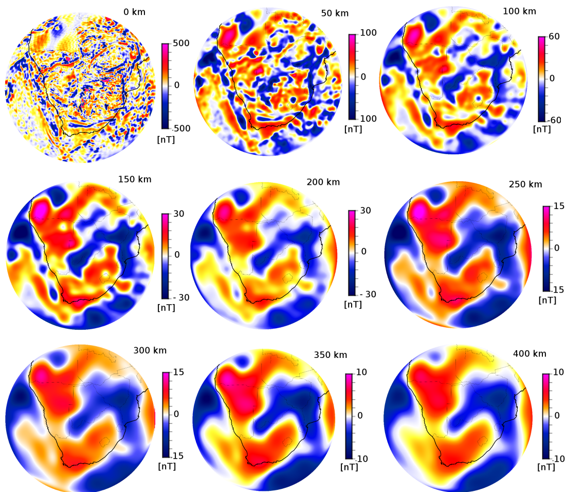
Figure 5. The Z component of our lithospheric field model plotted at different altitudes above the Earth's mean reference radius. Note the different colorscales.
