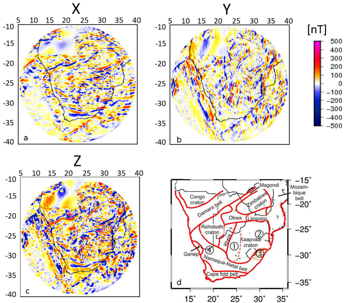
Figure 4. (a-c) The X, Y and Z component of our lithospheric field model plotted at the Earth's mean reference radius. (d) Outline of large-scale tectonic features, from Figure 8 by Korte and Mandea (2016).
