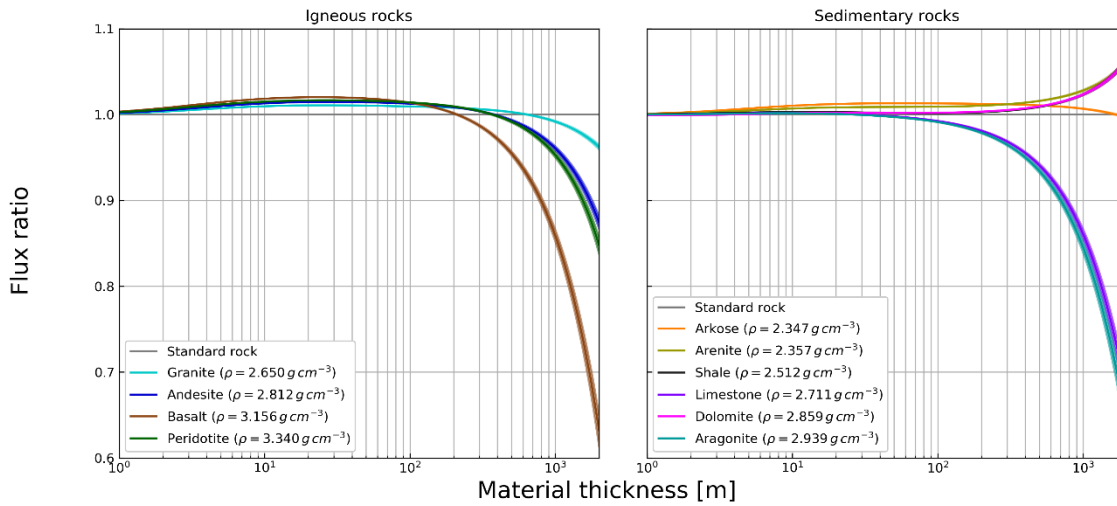
Figure 7: Ratio of the simulated rock fluxes to a standard rock muon flux with the same density as the rock ( \rho_{SR} = \rho_{Rock} ) for all the lithologies in Table 1 as a function of rock thickness.
