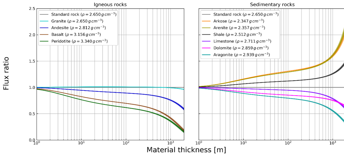
600 Figure 4: Ratio of the calculated rock fluxes to a standard rock ( \rho_{SR} = 2.650 \text{ g cm}^{-3} ) muon flux for the rocks reported in Table 1 as a function of rock thickness.
