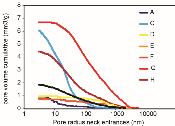
5 Figure 13. Results from multicycle MIP experiments. Pore radius of the neck entrances vs. cumulative pore volume.
