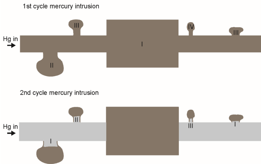
5 Figure 4. Conceptual model of 1st and 2nd MIP cycle. Numbers indicate the succession in pore filling, which is related to a stepwise increase in pressure, linked to a certain radius of a pore neck entrance. The second cycle indicates the remaining mercury from the first cycle.
