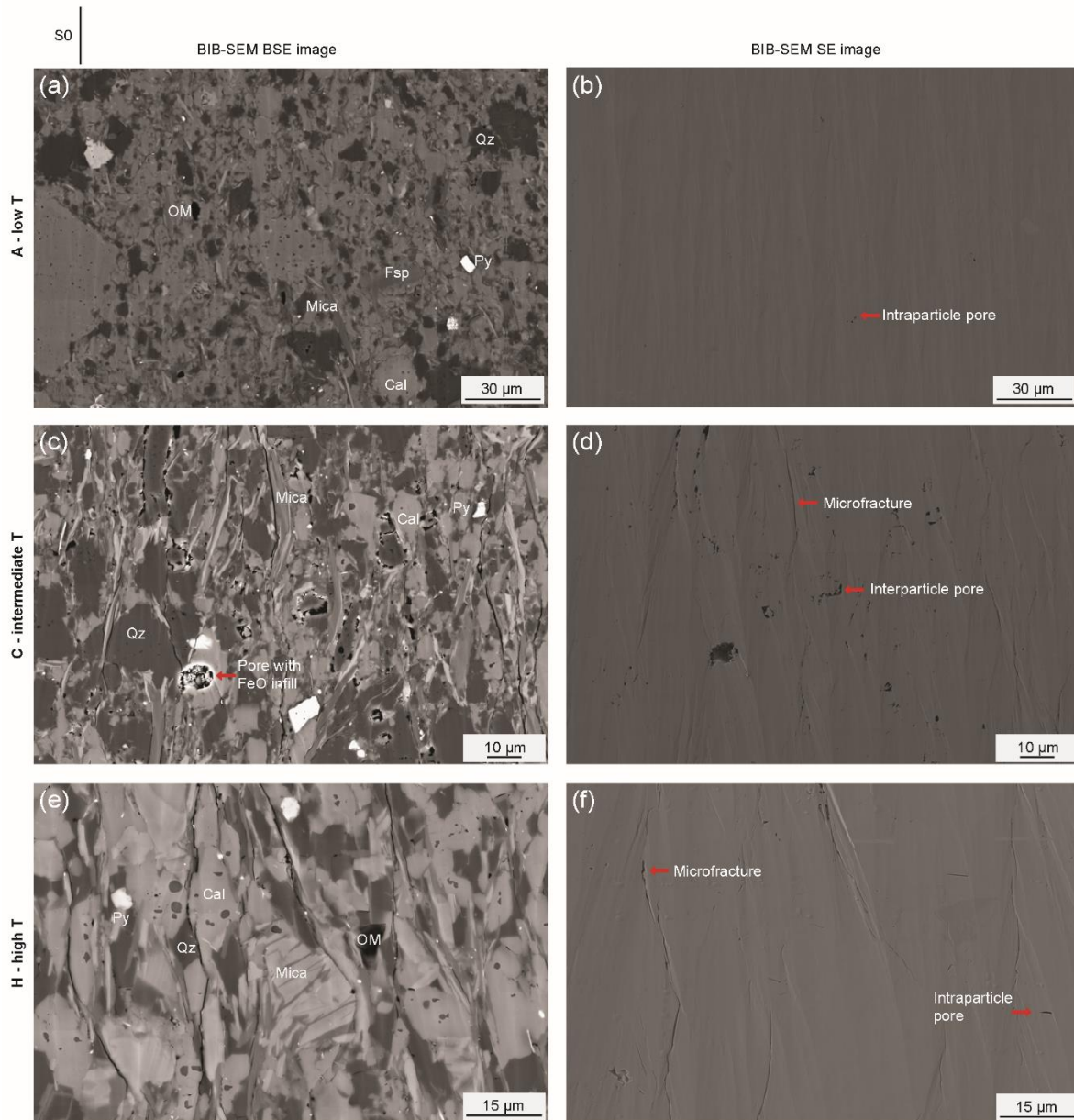
5 Figure 9. Microstructure and microstructural porosity imaged with BIB-SEM along the temperature gradient. a-b) Low temperature sample A shows smallest porosity, mainly present as intraparticle pores in quartz and dolomite. c-d) Intermediate temperature sample C shows microcracks along sheet-silicates and interparticle pores as effect of dissolution. e-f) High temperature sample H with a defined spaced cleavage shows more microcracks than the intermediate sample C. OM: organic matter, Qz: quartz, Py: pyrite, Fsp: feldspar, Cal: calcite, S0: bedding.
