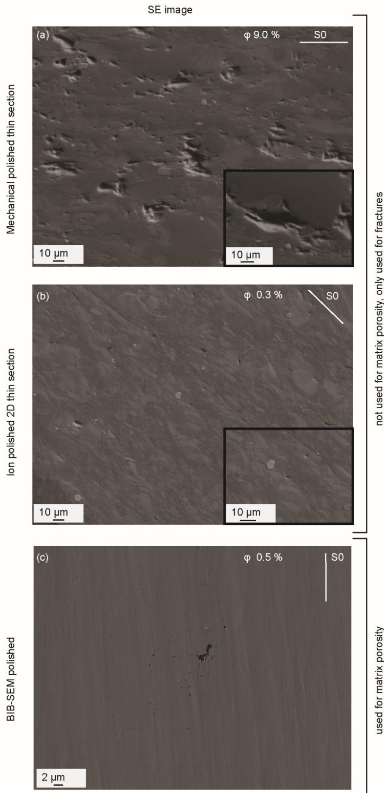
Figure 5. Differences in apparent porosity owing to applied sample polishing techniques in different samples a) Effect of conventional mechanical polishing of thin sections results in an overestimation of porosity owing to severe plugging of grains. b) Ion polished 2D surface of sample taken at 46°53'17.2"N 9°07'40.1"E shows a significantly smaller pore volume compared to the mechanical polishing technique. c) Smoothest surfaces with least induced pores created with BIB-SEM polishing. S0: bedding.
