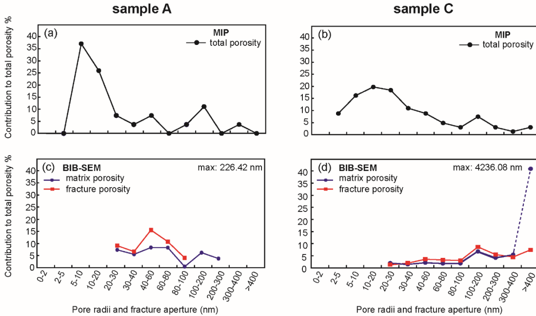
Figure 12. Pore size distributions from MIP compared to image analysis of BIB-SEM images. The pore radius is calculated from the pore area and for the fracture aperture, the minor axis of the calculated fit ellipse is used. a-b) Pore size distributions of MIP results of sample A and C. c-d) Pore size distributions of BIB-SEM analysed sub-samples divided in matrix and fracture porosity. MIP and BIB-SEM distributions show same general trend with peak at the 100–200 nm pore radii. Dashed line: large pore sizes (>300 nm) disturb distributions because of heterogeneity effect.
