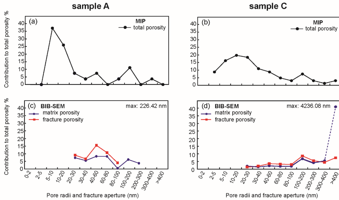
Figure 12. Pore size radii and fracture aperture distributions from MIP compared to image analysis of BIB-SEM images. The pore radius is calculated from the pore area and for the fracture aperture, the minor axis of the calculated fit ellipse is used. a-b) Pore size distributions of MIP results of sample A and C. c-d) Pore size distributions of BIB-SEM analysed sub-samples divided in matrix and fracture porosity. MIP and BIB-SEM distributions show same general trend with peak at the 100–200 nm pore radii. Dashed line: large pore sizes (>300 nm) disturb distributions because of heterogeneity effect.
