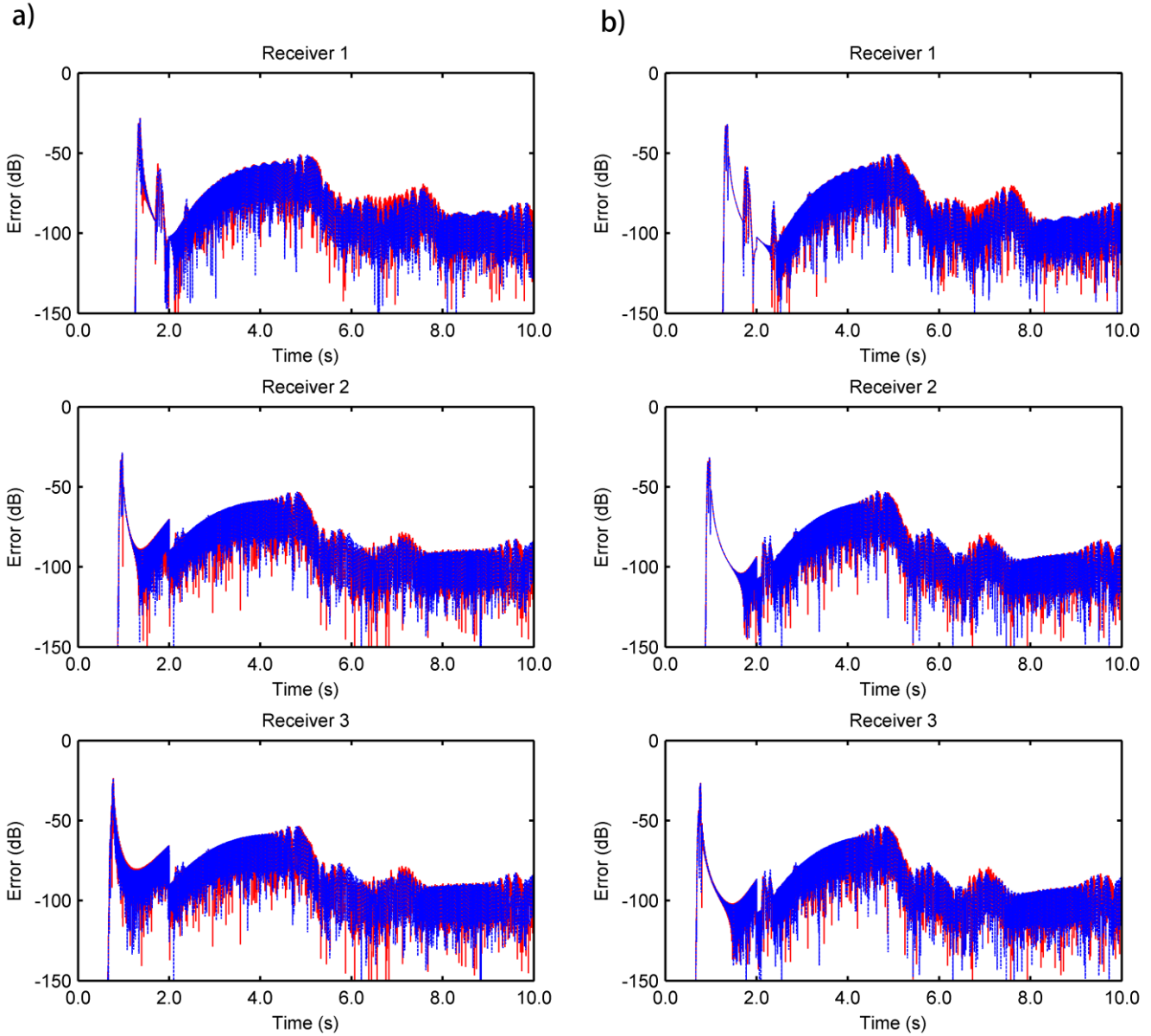
2 Figure 8. Comparison of the relative errors between the analytical solutions and the proposed method 3 (fourth-order CG scheme) (red solid line) or the classic SG PML method (fourth-order SG scheme) (blue dotted 4 line) at different receiving points and different grid spacings. (a) d = 12 m, receiving points 1, 2, and 3; (b) d = 5 10 m, receiving points 1, 2, and 3.
