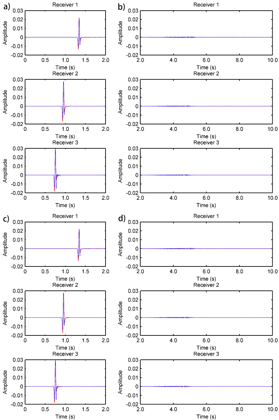
5 Figure 6. Comparison of the analytical solution (red solid line) with the proposed (fourth-order CG scheme) 6 and classic SG PML methods (fourth-order SG scheme) (blue dotted line) at different receiving points and d = 12 7 m. (a) Proposed method at receivers 1, 2, and 3 during the first two seconds; (b) proposed method at receivers 1, 2,
