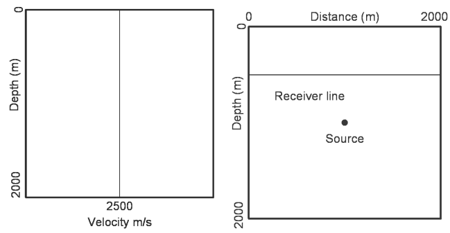
3 4 Figure 11. Velocity profiles with depth and the location of source and receiving points.
