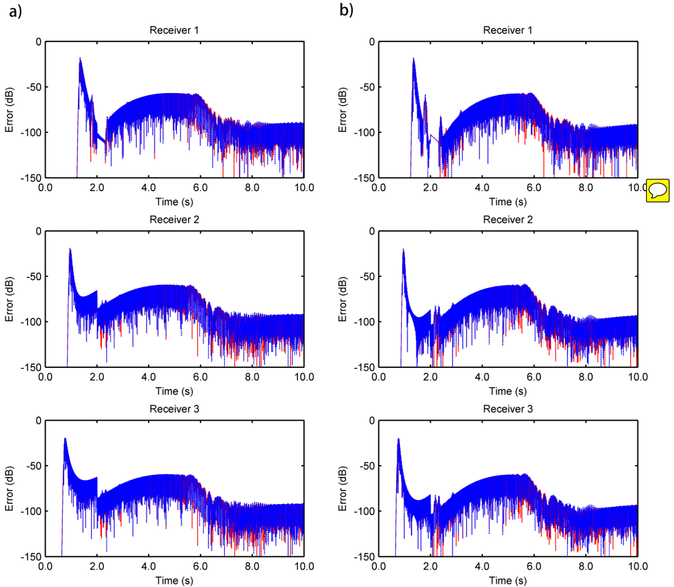
2 Figure 5. Comparison of the relative errors between the analytical solutions and the proposed method 3 (second-order CG scheme) (red solid line) or the classic SG PML method (second-order SG scheme) (blue 4 dotted line) at different receiving points and different grid spacings. (a) d = 12 m, receiving points 1, 2, and 3; 5 (b) d = 10 m, receiving points 1, 2, and 3.
