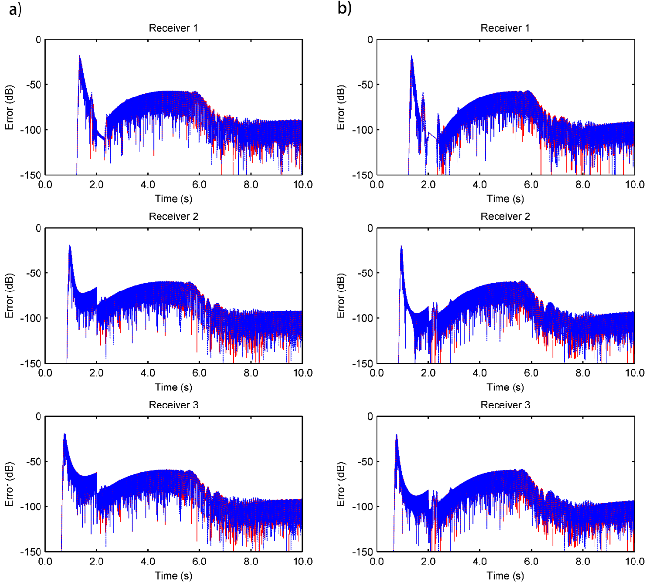
Figure 5. Comparison of the relative errors between the analytical solutions and the proposed method (second-order CG scheme) (red solid line) or the classic SG PML method (second-order SG scheme) (blue dotted line) at different receiving points and different grid spacings. (a) d = 12 m, receiving points 1, 2, and 3; (b) d = 10 m, receiving points 1, 2, and 3.
