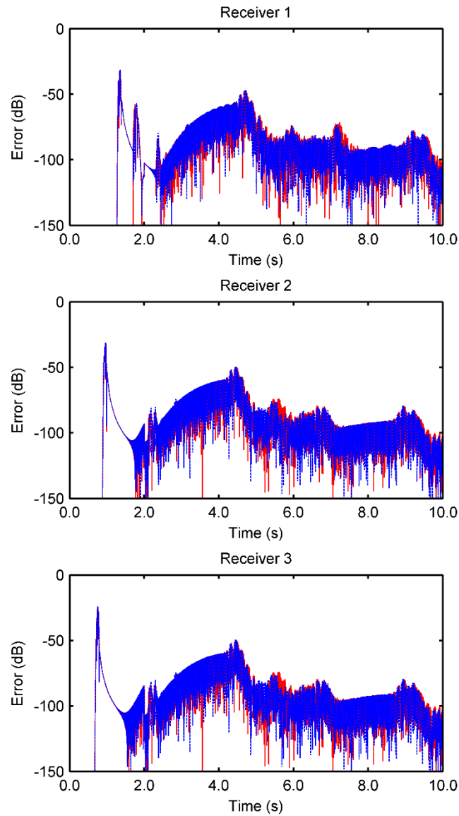
3 4 Figure 10. Comparison of the relative errors between the analytical solutions and the proposed method 5 (tenth-order CG scheme) (red solid line) or the classic SG PML method (tenth-order SG scheme) (blue dotted 6 line) at different receiving points and different grid spacings. d = 10 m, receiving points 1, 2, and 3.
