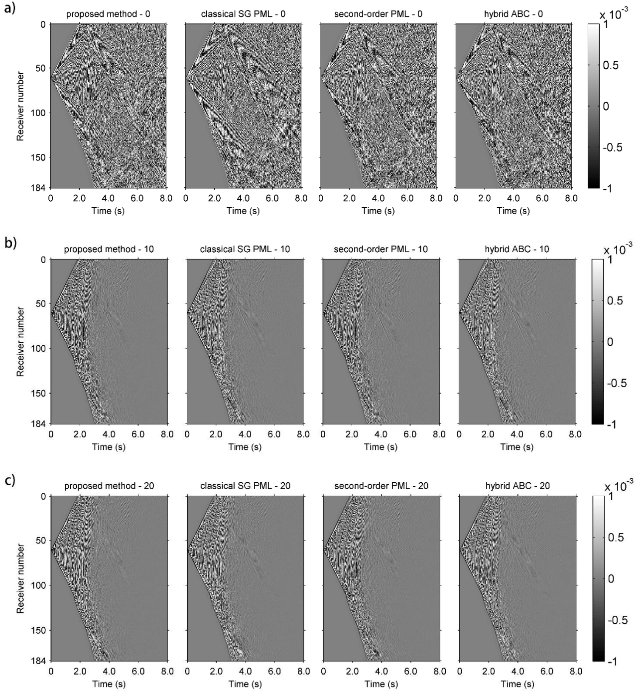
Figure 18. Receiving point records for the four methods for a different number of absorbing layers: (a) 0 absorbing layers; (b) 10 absorbing layers; and (c) 20 absorbing layers.
