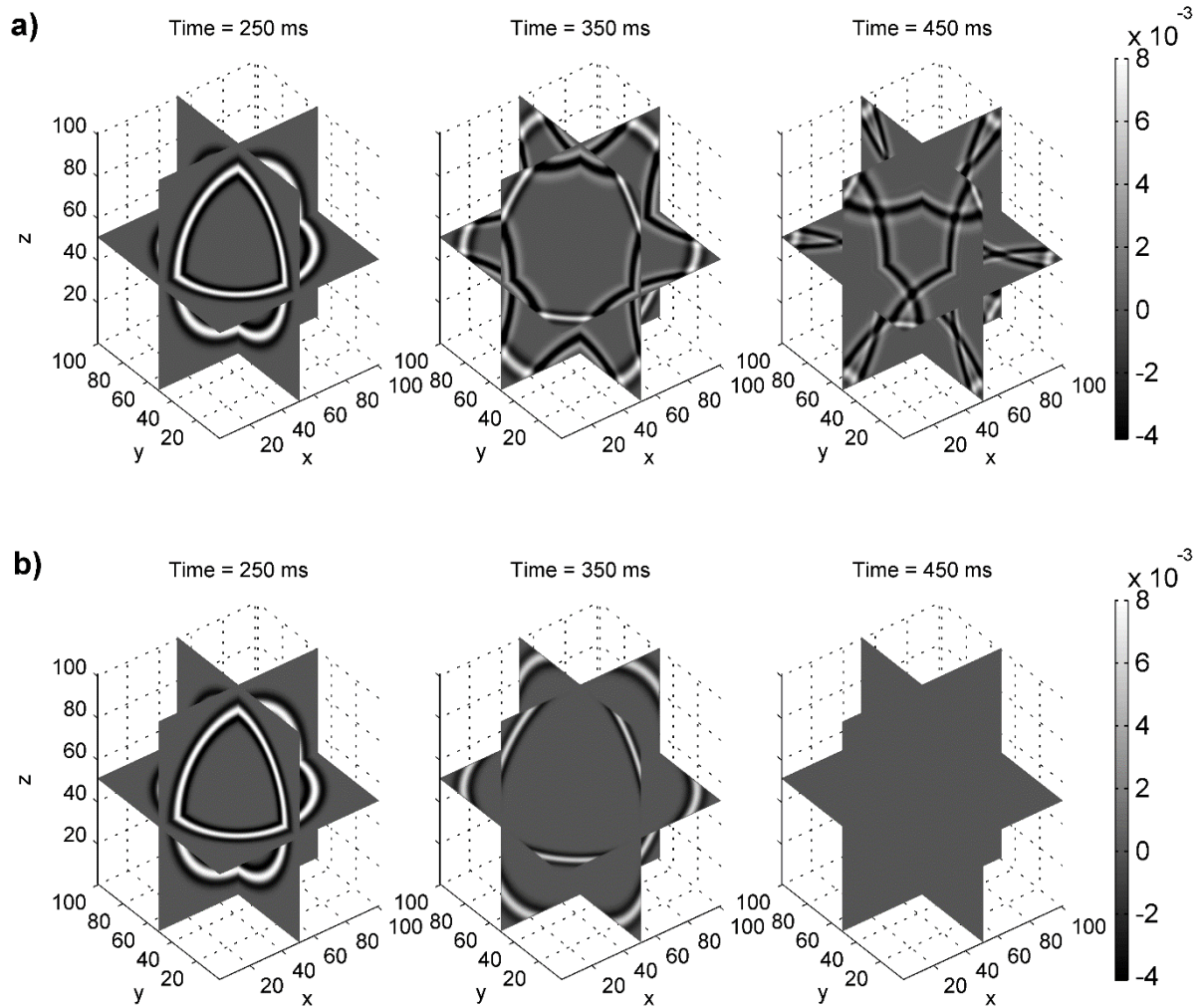
Figure 19. Wave field snapshots with different PML at different time, the three coordinate axis represent the number of grids in three directions.: (a) PML=0 at 250 ms, 350 ms and 450 ms; (b) PML=20 at 250 ms, 350 ms and 450 ms.
