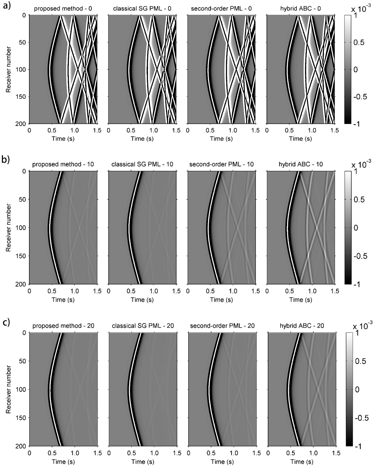
Figure 12. Receiving point records of the four methods for a different number of absorbing layers: (a) 0 absorbing layers; (b) 10 absorbing layers; and (c) 20 absorbing layers.
