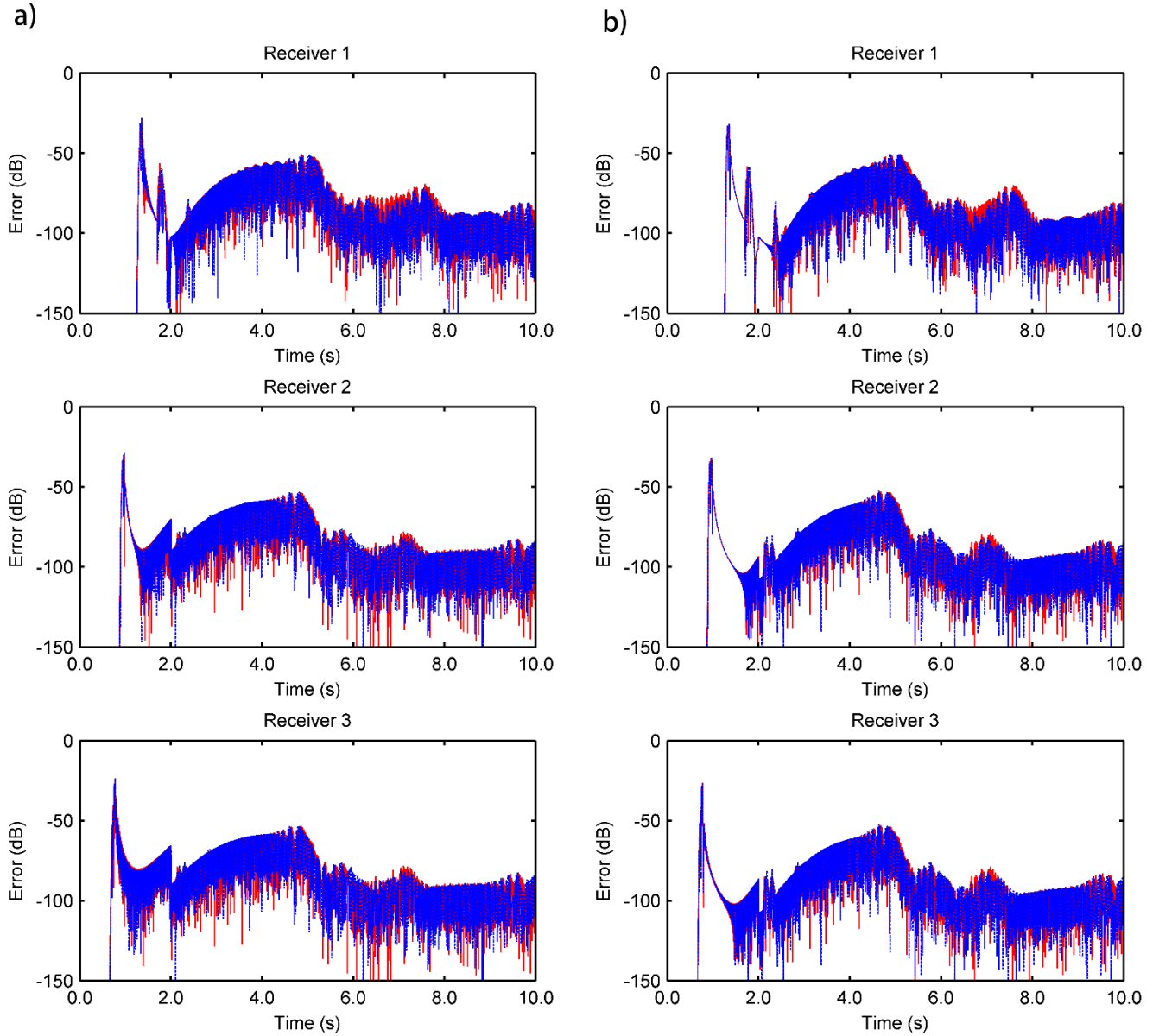
Figure 8. Comparison of the relative errors between the analytical solutions and the proposed method (fourth-order CG scheme) (red solid line) or the classic SG PML method (fourth-order SG scheme) (blue dotted line) at different receiving points and different grid spacings. (a) d = 12 m, receiving points 1, 2, and 3; (b) d = 10 m, receiving points 1, 2, and 3.
